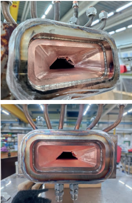
Figure 2 View inside the damaged absorbers of the wiggler sections West (top) and North (bottom)
