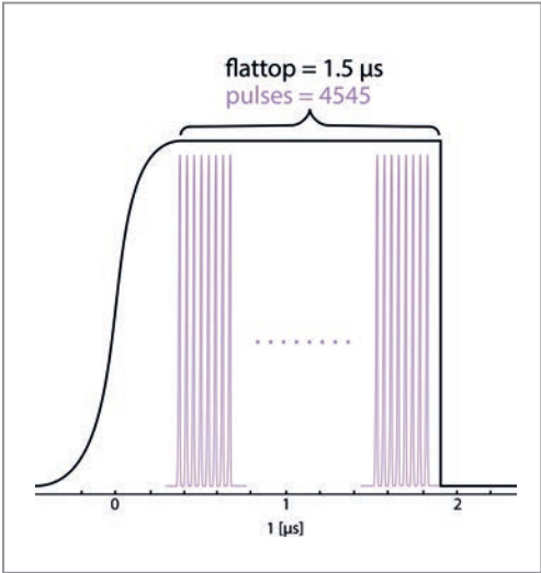
Figure 2 3 GHz pulse train mode: About 4500 bunches are equally distributed over the flat-top RF pulse length of 1.5 \mu s.
