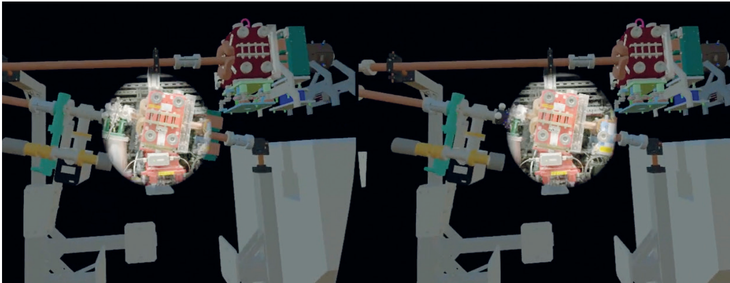
Figure 1 Screenshot from our immersive neural graphics VR system for virtual accelerator inspection, where the NeRF 3D model representing the physical reality of the European XFEL linear accelerator is merged with the virtual CAD model of the accelerator
