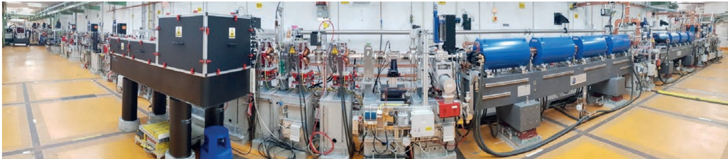
Figure 1 Fish-eye view of the fully installed ARES accelerator. The electron source (gun) can be seen on the right, the experimental area with the laser table in the middle and the PolariX TDS on the left.
