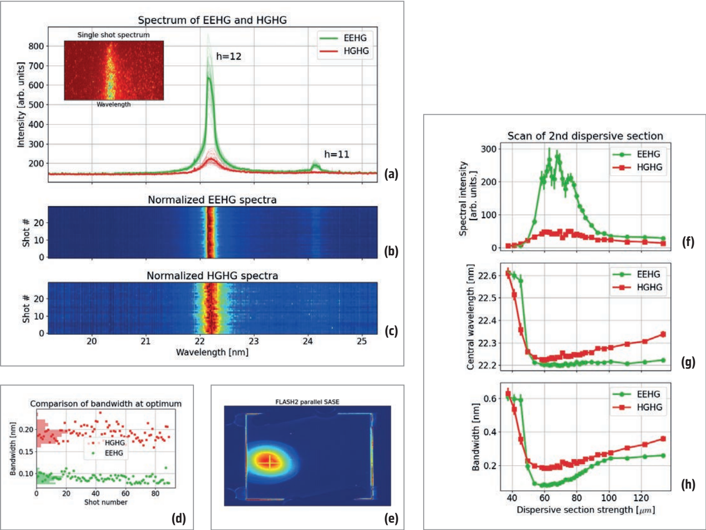
Figure 1 Parallel operation of seeded FLASH1 together with SASE in FLASH2. (a) Comparison of the average spectrum for HGHG and EEHG when lasing at 22.1 nm ( h = 12 ). The inset shows an example of a single-shot spectrum in false colours. (b, c) Single-shot spectra shown in narrower lines for 30 consecutive shots and in false-colour scale. (d) Comparison of the spectral bandwidth stability for 90 shots for EEHG and HGHG. Here, the beamline was optimised for EEHG, hence the relatively larger bandwidth and reduced spectral intensity of HGHG compared to EEHG (see also: a). (e) Transverse mode for SASE radiation at 30 nm with about 100 \mu J pulse energy. (f, g, h) Comparison of the spectral properties – intensity (f), central wavelength (g) and bandwidth (h) – as a function of the dispersive section strength for EEHG and HGHG.
