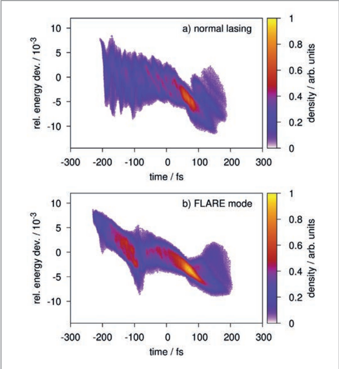
Figure 3 Measurements of the longitudinal phase space after the FLASH2 undulators: (a) Laser heater turned off: The spiky structure in the range from -200 fs to 0 fs is a strong indication for the FEL process. (b) Partial overheating with the FLARE setup: Suppression of the FEL process in a major part of the bunch. The characteristic spiky FEL structure is only present around -90 fs with a significantly reduced FEL pulse length.
