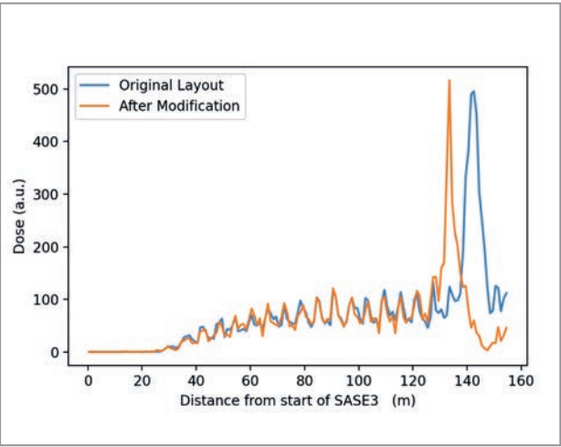
Figure 2 Simulation (left) and measurement (right) results before and after changing the aperture of the absorbers. In the simulation, no lead (Pb) shielding was added after the modification, which resulted in a higher radiation dose compared to the measurements.
