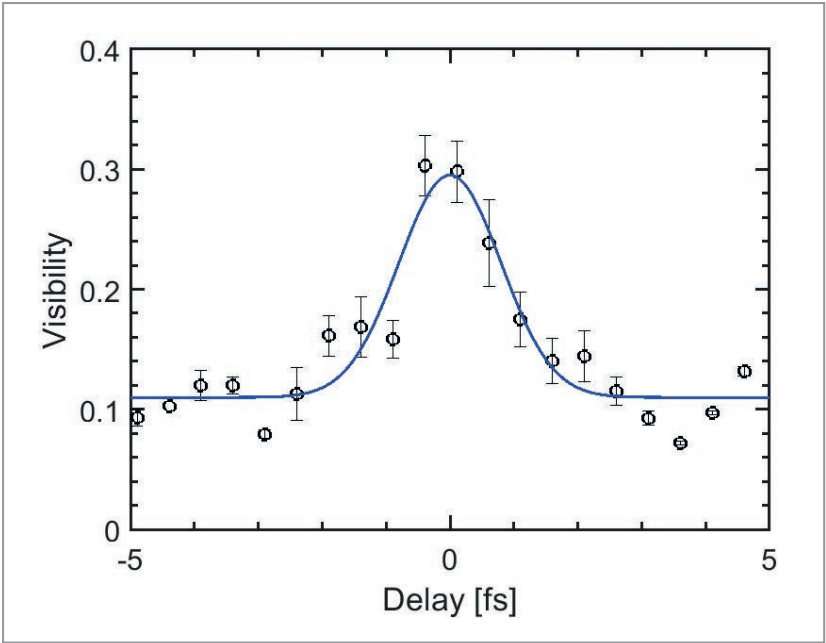
Figure 2 Field autocorrelation (AC) trace. The change in the interference fringes depends on the delay of the two overlapping photon pulses created using the split-and-delay unit at FLASH2. In the case of single-spike SASE pulses, the width of the AC trace is directly related to the photon pulse duration. The conversion factor was determined by modelling and leads to a measured photon pulse duration of 1.26 \pm 0.37 fs.
