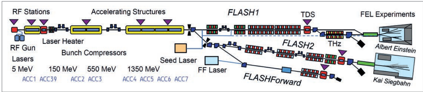
Figure 1 FLASH facility layout after the upgrade in 2022
