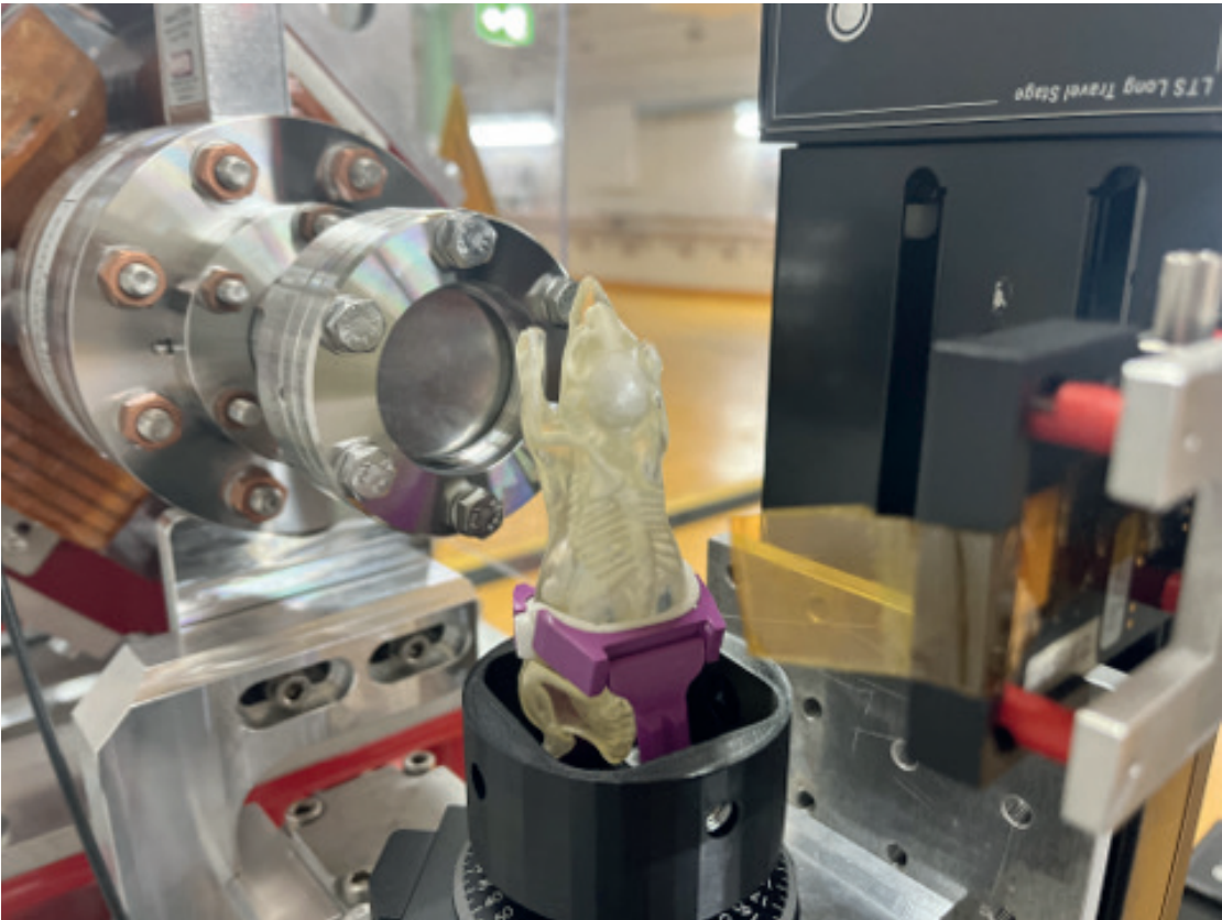
Figure 2 Experimental setup of the “electron CT” experiment. The titanium foil at the end of ARES is located on the left, the mouse phantom from UKE in the middle and the detector from the DESY Particle Physics Division on the right.
