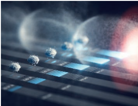
In a laser plasma accelerator, a high-intensity laser pulse (red) creates a plasma wave (white) in an ionised gas. This wave makes it possible to accelerate electrons to extremely high energies within just a few millimetres. Using machine learning, the scientists at DESY’s LUX experiment can now control the properties of the electron bunches, such as charge and energy spread (shown in rows here), with high precision.
