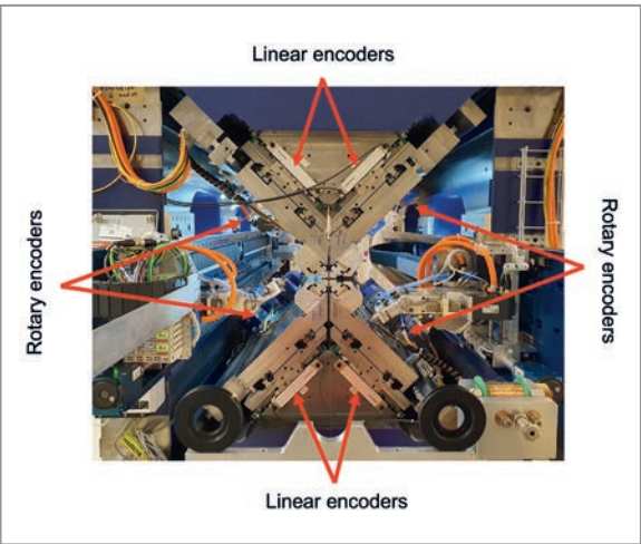
Figure 1 Left: APPLE-X undulators installed downstream of SASE3. Right: Location of the encoders on the APPLE-X undulators. Linear encoders are situated on the downstream side of the undulators, around 30 cm away from the electron beam. Rotary encoders are mounted on the motors located on the sides of the undulators at a distance of 30–40 cm from the electron beam.
