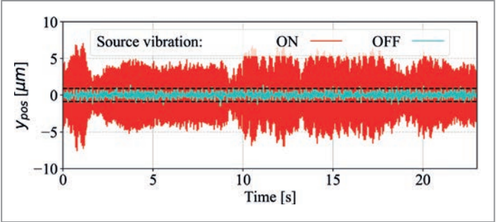
Figure 4 Vertical electron beam position changes at the undulator of the beamline P07 during excitation with a vibrating roller (red) and quiet reference without excitation (light blue). The PETRA III stability goal of 10% of the beam size is marked by the two black dashed lines.
