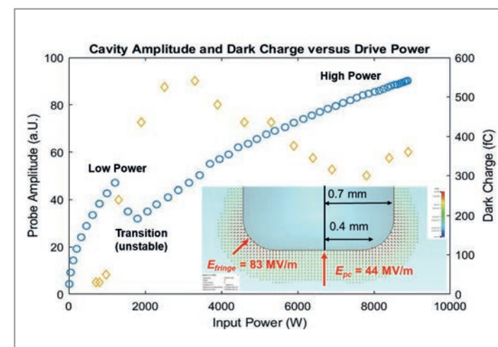
Figure 1 Left: UED RF gun test setup as currently installed in the CFEL building. Right: Cavity amplitude and dark charge emission response as a function of driving power. Inset: Electric field distribution of the pin cathode for a measured electron acceleration energy of 62 keV.
