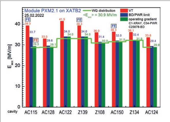
Figure 3 PXM2.1 and PXM3.1 cavities: Comparison of maximum gradients in vertical tests (VT, red) and cryomodule tests (blue). The operating gradient is indicated in green; the green line gives the gradients with an adapted RF power waveguide distribution.
