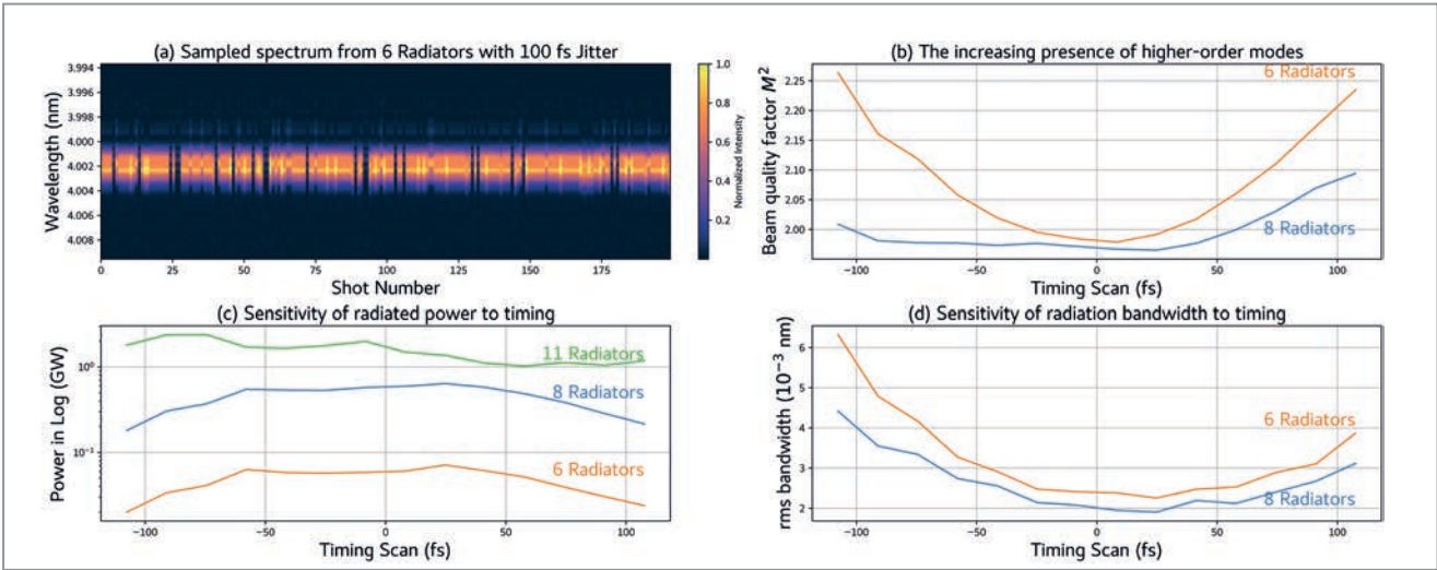
Figure 2 Example tolerance study data set. The optimised working point corresponds to a 1.35 GeV electron beam with linear chirp. (a) Photon beam spectra for 100 random samples. A shift in the central wavelength can be seen, which is due to the different beam energies involved in the FEL process. (b) Impact of timing on the transverse quality factor ( M^2 ) of the beam: As the quality factor increases, the FEL beam is composed of more transverse modes with higher divergence. (c, d) Illustration of the impact of timing changes on the spectral properties power (c) and bandwidth (d).
