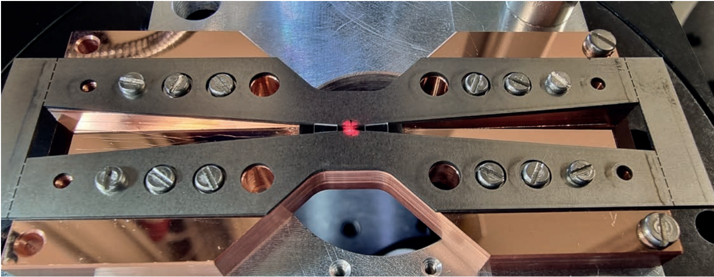
Figure 2 Three-layer THz photogun under assembly. The copper base forms the support structure, the photocathode as well as half of the horn antennae used to couple in the THz energy. Two tungsten "spacers", a steel divider and two dielectric trapezoids, which are used to construct the layered interaction region, can also be seen. A red helium-neon beam is used for alignment.
