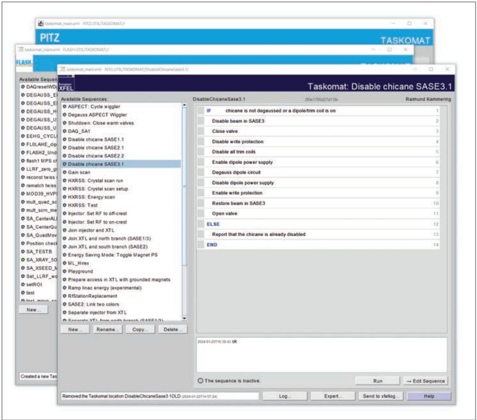
Figure 1 Taskomat sequence selectors for the European XFEL, FLASH and PITZ
