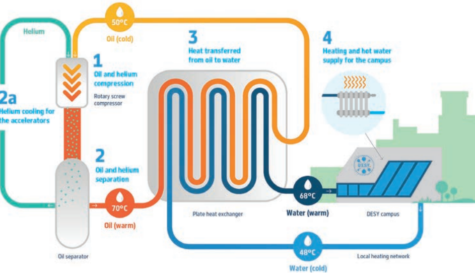
Waste heat recycling system at DESY: The accelerators and their support systems can be used to warm the entire campus. So far, a third of the campus is heated in this way.
