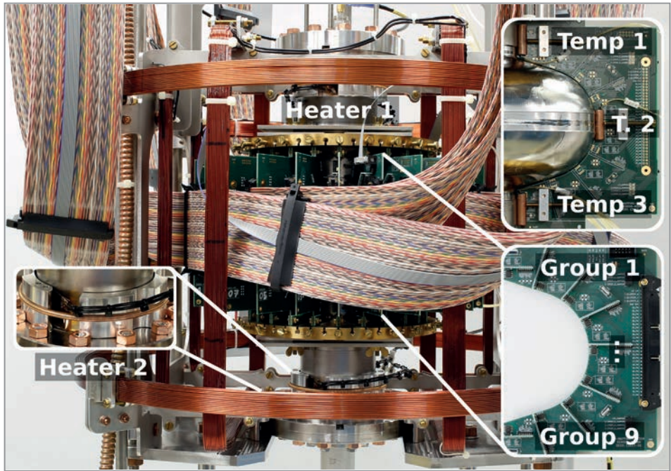
Figure 1 View into a vertical test stand for superconducting cavities. A single-cell niobium cavity is located in the centre, surrounded by a large number of electronic boards, each equipped with magnetic sensors (nine groups) or thermocouples. The complete setup is cooled in a vertical dewar using liquid helium. The cavity performance (accelerating field and thermal losses) is measured at 2 K together with a magnetic field mapping performed using the installed sensors of the system.
