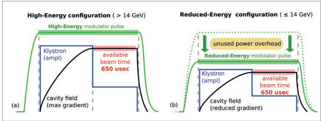
Figure 1 Modulator (green), klystron (blue) and cavity (black) pulse shape in the high-energy (a) and reduced-energy (b) configurations
