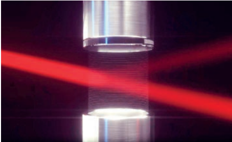
A laser beam passes between a loudspeaker-reflector array that creates a grating of air. The laser beam interacts with this grating and is deflected without contact.
