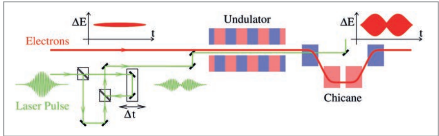
Figure 1 FLARE setup: An interferometer is used to control the shape of the laser pulse via the time delay ( \Delta t ) and thus the energy modulation that is transferred to the electron bunch in a undulator. This energy modulation is then transformed into an energy spread modulation in the subsequent chicane.
