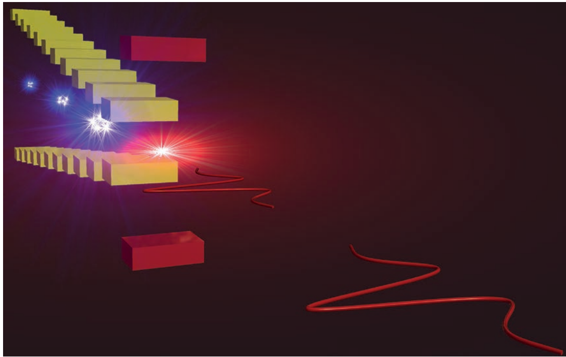
Figure 1 Schematic illustration of the new short-pulse scheme. The gaps of the magnetic segments of the undulator structure are decreasing along the undulator length, which changes the resonance conditions for the SASE lasing process. In this way, the long radiation pulse is suppressed, while the microbunching within the electron bunch is maintained. The last undulator segment – called the radiator – is then tuned to resonance with the incoming microbunching, resulting in the emission of ultrashort pulses that are not limited by the coherence time.
