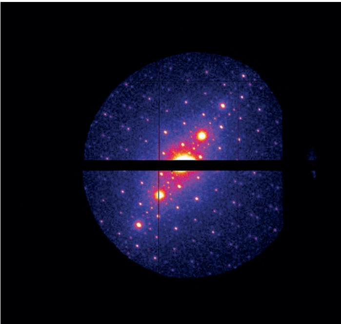
Figure 2 Diffraction image with super lattice reflections from a charge density wave recorded at REGAE from a 20 nm thick crystal of the 2D material tantalum disulfide (TaS 2 ) obtained by sample preparation with a microtome
