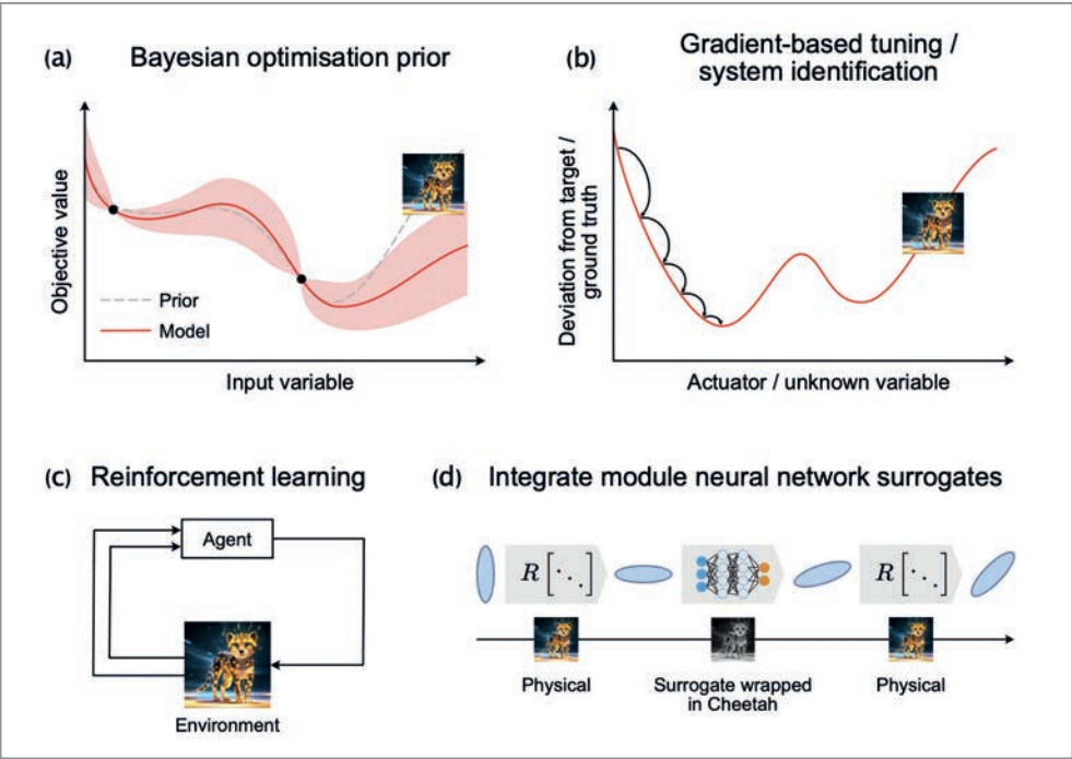
Figure 4 Overview of application examples for the Cheetah simulation code, illustrating where it is applied in each respective application
