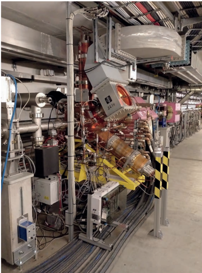
Figure 1 PETRA IV prototype single-cell 500 MHz cavity
