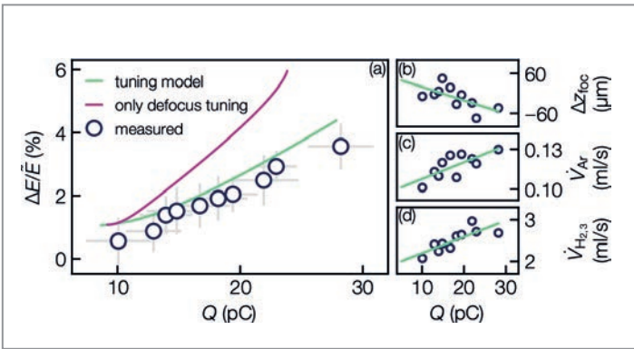
Figure 2 Tuning of the beam charge (left) at LUX, exploiting the tuning curve using the most relevant parameters (right) found through multi-objective Bayesian optimisation (green) and simple single-parameter tuning (red). Adapted from [1].
