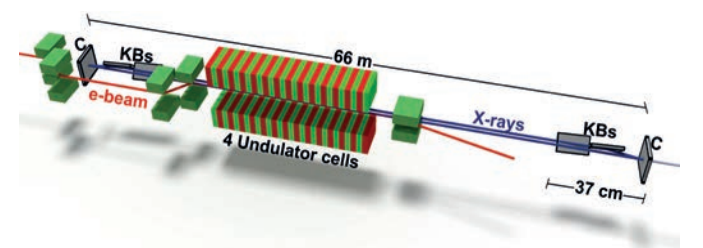
Figure 2 Sketch of the demonstrator setup (the illustration is not to scale; in addition, the undulator cells are not centred in the cavity, as it appears, but much closer to the upstream mirror, and the crystal and mirror assembly is only about 50 cm in size)
