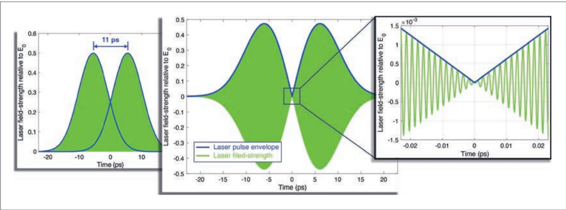
Figure 2 Left: Two laser pulses separated in the interferometer by 11 ps (without interference effect). Centre: Recombined laser pulse at destructive interference (i.e. the laser pulses have a phase difference of 180^\circ ). Right: Centre region enlarged to resolve individual laser wavelengths.
