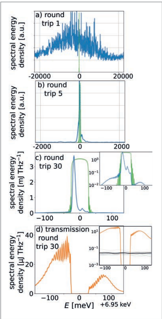
Figure 4 (a-c) Spectral representation of the X-ray pulse before reflection for different numbers of round trips (1, 5 and 30, respectively). The blue line denotes the X-ray field spectrum and the green line the crystal reflectivity. (d) Transmitted X-ray pulse in saturation. In the inset, the spectral energy density of a typical SASE pulse is shown on a logarithmic scale for reference.
