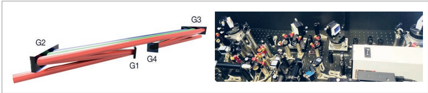
Figure 1 Left: Iso view of the out-of-plane compressor geometry. From [5]. Right: Energy-scaled test compressor.
