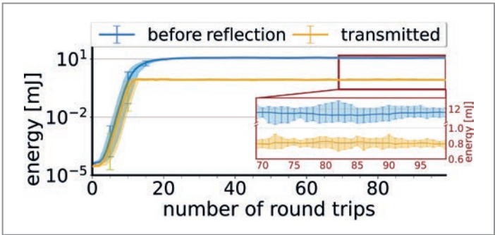
Figure 3 Evolution of the circulating and transmitted X-ray pulse energy as a function of the number of cavity round trips, showing exponential gain
