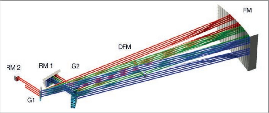
Figure 2 Left: Iso view of the two-transmission-grating stretcher including simulated beam paths. From [5].
