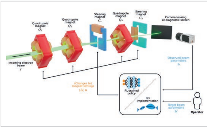
Figure 2 Control loop for reinforcement learning and Bayesian optimisation for transverse beam parameter tuning in the experimental area section of ARES
