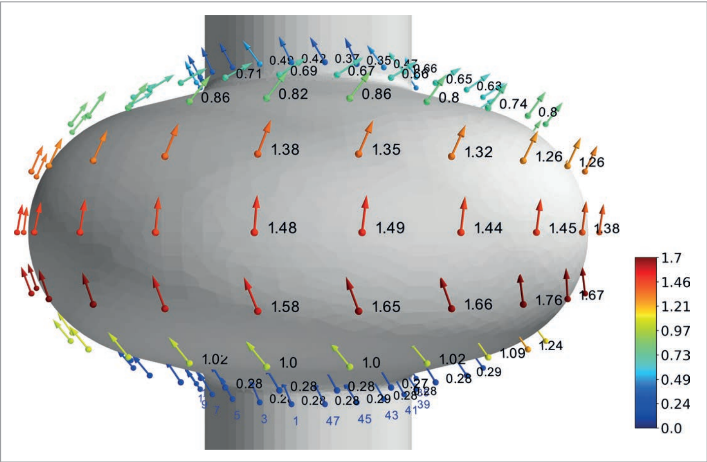
Figure 2 Magnetic flux distribution snapshot of the cavity 1DE26 recorded before mid-T heat treatment in the superconducting state for a cooldown velocity of -5 K/h and a spatial temperature gradient of 4 K over the complete cavity cell. The given numbers indicate the fraction of magnetic flux expelled. An inclined transition from the normal-conducting to the superconducting state of the cavity material at 9.2 K led to an asymmetrical magnetic flux expulsion.
