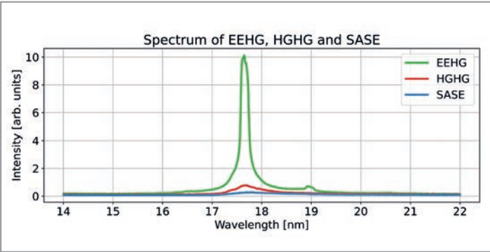
Figure 2 Spectrum of the 15 th harmonic optimised for EEHG compared to the residual high-gain harmonic generation (HGHG) and to SASE
