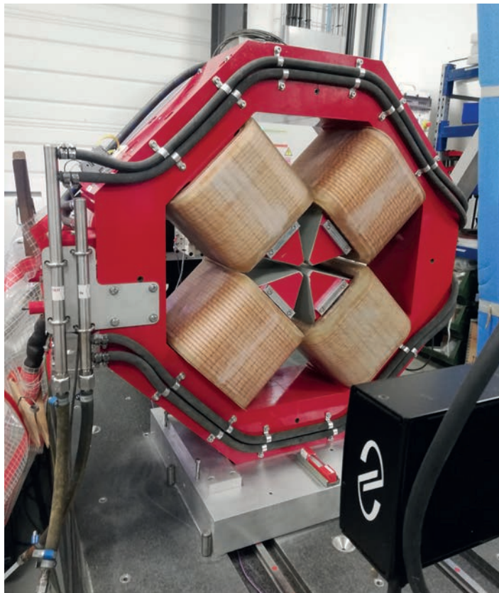
Figure 1 Prototype of the 115 T/m high-field quadrupole magnet for PETRA IV on a test stand at SIGMAPHI
