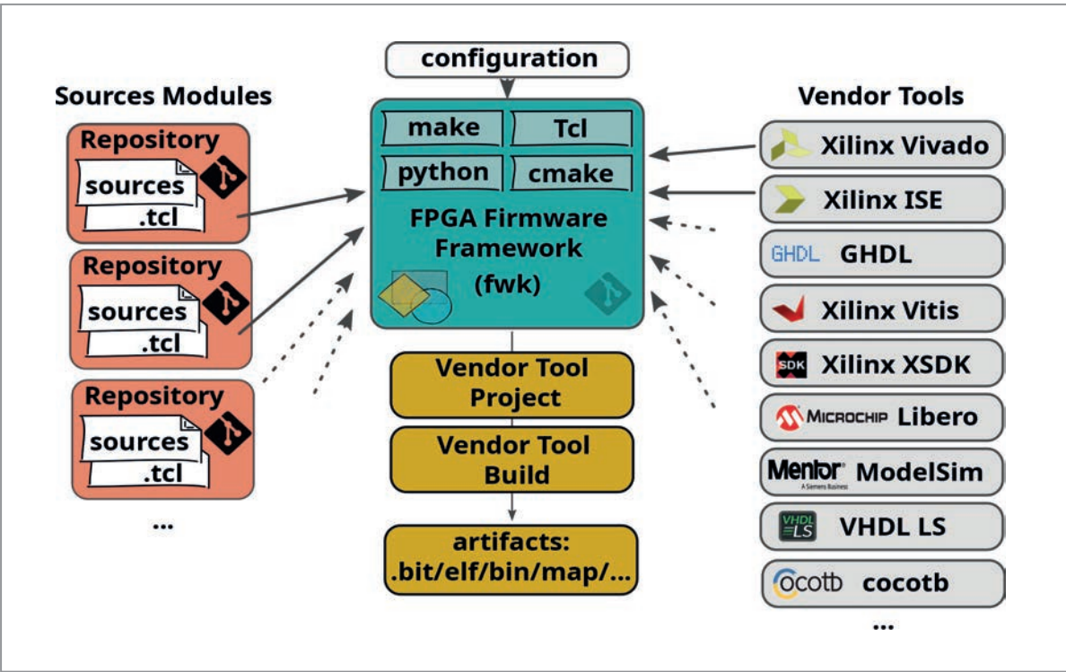
Figure 2 Major components of the FPGA firmware framework
