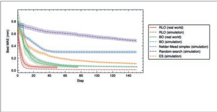
Figure 3 Averaged tuning objectives over time for different algorithms. Reinforcement learning (RL) achieves faster convergence to lower objective values than any other algorithm, while Bayesian optimisation (BO) is convincing in terms of ease of setup and engineering effort.
