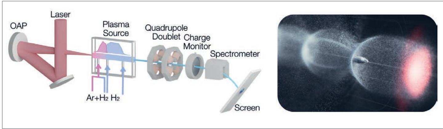
Figure 1 Schematic of the LUX accelerator (left) [2]: Laser pulses with 100 TW peak power are focused into a plasma source, where they drive a plasma wave (simulation on the right) and accelerate electron bunches to around 300 MeV. The accelerated electron bunches are focused into a set of diagnostics to measure, among other parameters, the charge and energy spectrum. To find optimal ways of tuning the beam parameters, the vast parameter space of the experiment is explored using a machine learning method called Bayesian optimisation. Adapted from [1] and Science Communication Lab [5].
