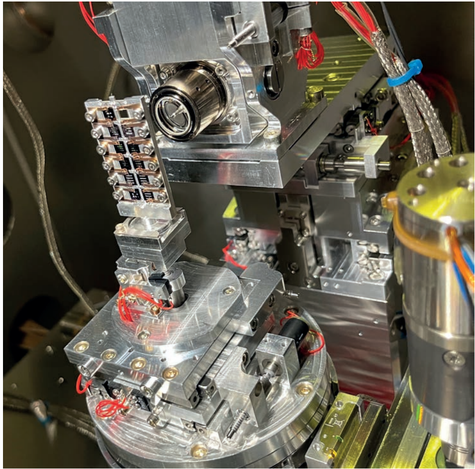
Figure 1 View inside REGAE's experimental ultrahigh-vacuum chamber equipped with an inline sample viewing microscope (top). A sample holder carrying 12 different samples (centre left) is mounted on an e-Roadrunner goniometer (bottom left).
