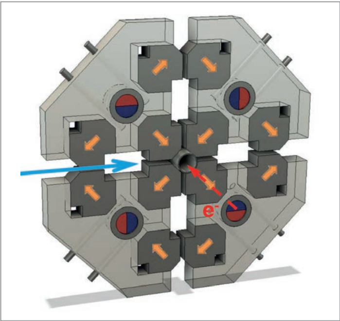
Figure 2 Different segments of the APPLE-III undulator
