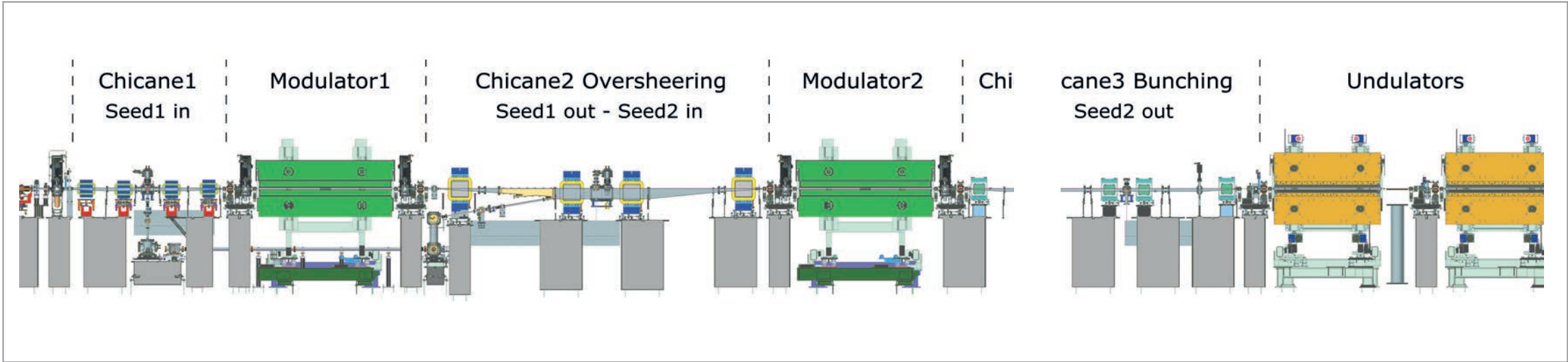
Figure 1 Excerpt from the full CAD model of the new FLASH1 beamline, showing the seeding section with the electron and laser beam propagating from left to right. The seeding section consists of three chicanes and two modulators to prepare a bunched electron beam so as to efficiently generate stable soft X-ray beams in the downstream undulators, two of which are displayed on the right. For shortest wavelengths, echo-enabled harmonic generation (EEHG) is used, where a laser beam is coupled in within the first chicane to be overlapped with the electron beam in the first modulator (green). Here, energy from the laser is transferred to the electron beam. The second chicane makes it possible to remove the first laser, couple in a fresh laser beam and simultaneously redistribute the energy-modulated electron beam to generate multiple slices with low energy spread. In the second modulator, a sinusoidal energy modulation is imprinted on the electron beam by the laser. Finally, in the third chicane, a very subtle rearrangement of the beam “bunches” the electron beam, meaning that sharp current spikes develop in the beam propagation direction. These spikes then allow for very stable lasing in the subsequent radiators (orange).
