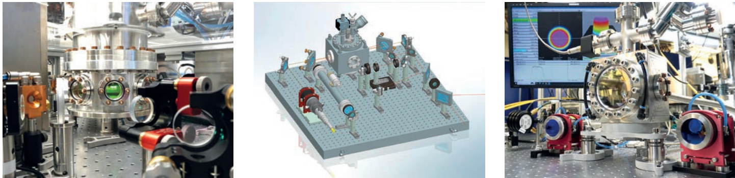
Figure 1 Left: Yb:YLF crystal bonded with a new bonding technique. Centre: 3D prototype design of a 450 W compact Yb:YLF laser unit. Right: Installation of a 2 J module for a Yb:YAG system
