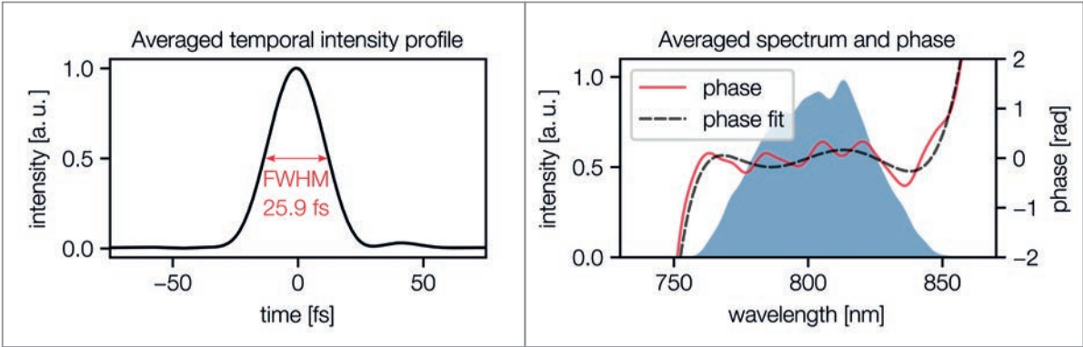
Figure 3 Measured pulse length of the compressed pulse. Left: Temporal intensity profile of the compressed pulse. Right: Measured spectrum and spectral phase. Both figures adapted from [5].
