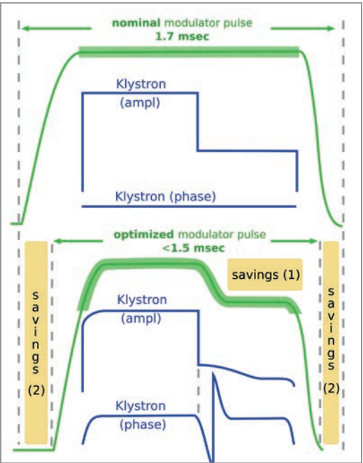
Figure 2 Nominal (top) and optimised (bottom) use of the modulator pulses, shown in green. The modulator pulse shape is shortened and tailored to the RF pulse profile. The impact of these modifications on the klystron output amplitude and phase is shown in blue.
