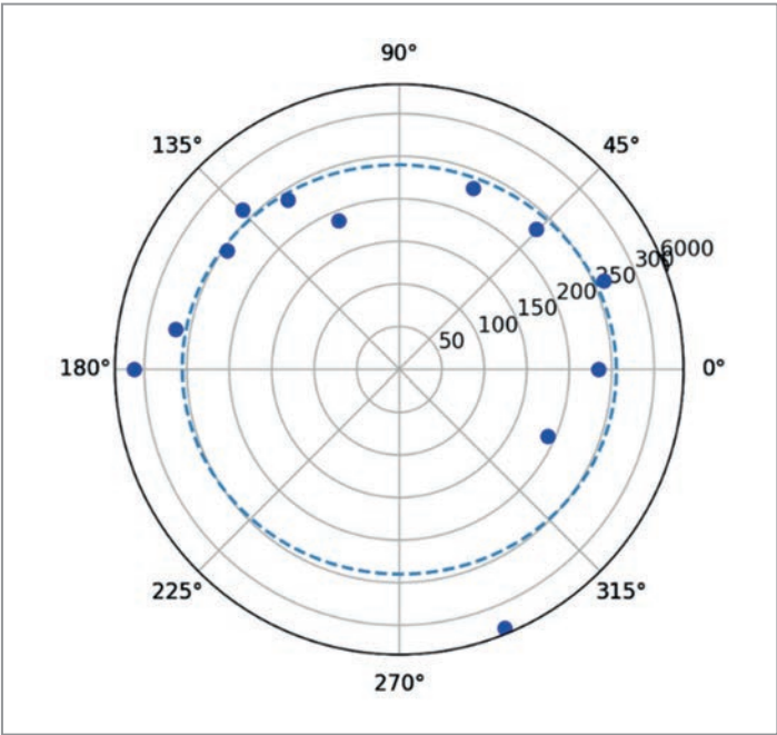
Figure 3 Measurement with the “ballchamber” when the APPLE-III undulator was set up for circular polarisation
