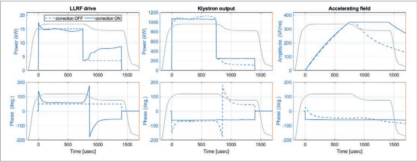
Figure 3 Amplitude (top) and phase (bottom) of the LLRF drive (left), klystron output (middle) and cavity field (right) without (dashed line) and with (solid line) the LLRF corrections. The modulator shape is shown in grey to visualise the time alignment with respect to the RF pulse.
