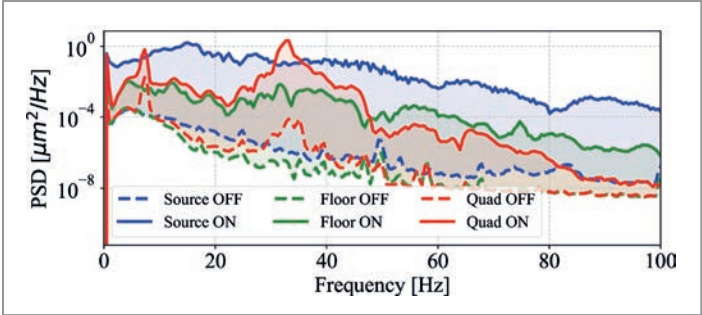
Figure 3 Frequency spectra of ground vibrations during the stone drop experiment measured close to the source (solid blue), on the tunnel floor (solid green) and on top of a quadrupole (solid red). The filling indicates the difference between the spectra with excitation (solid lines) and the quiet spectra without excitation (dashed lines).
