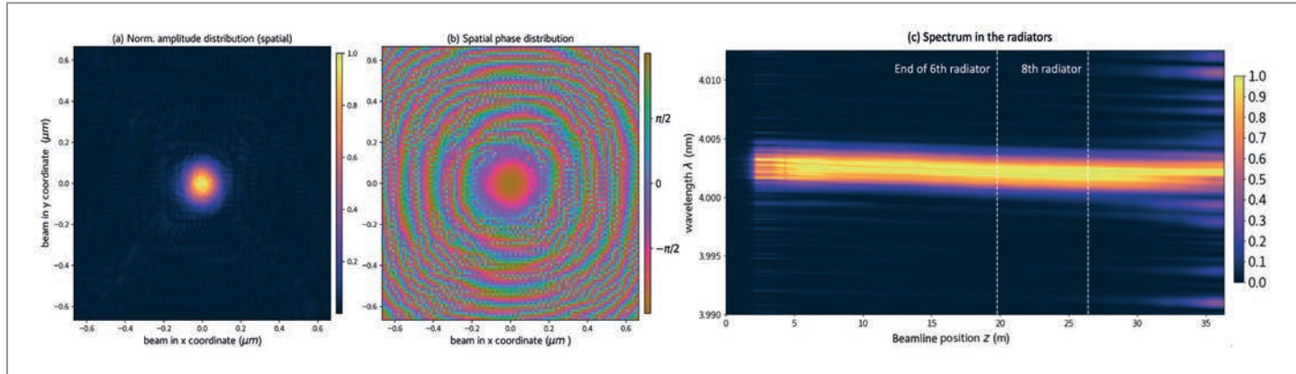
Figure 1 Transverse field (spatial) and longitudinal (temporal) properties of a simulation optimised for a 1.35 GeV electron beam with a chirp of 19 MeV per picosecond (highest value foreseen for the chirp at FLASH) with tapered circularly polarised radiators. (a) Amplitude and (b) phase of the projected FEL field after the sixth radiator. (c) Evolution of the spectrum along the beamline.
