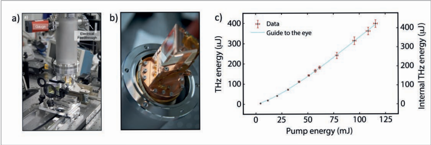
Figure 1 (a) Cryostat and imaging system for the tilted pulse front setup. (b) Large-aperture lithium niobate conversion medium, accepting drive beams of more than 100 mJ. (c) THz yield from one of the twin setups. 400 μJ of usable energy were collected, indicating that up to 800 μJ were generated within the crystal and can be collected with improved output coupling methods.
