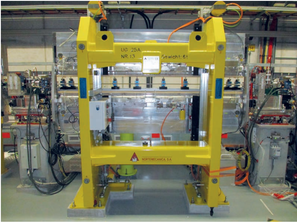
Figure 1 Afterburner undulator after installation in FLASH2
