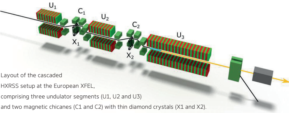
Layout of the cascaded HXRSS setup at the European XFEL, comprising three undulator segments (U1, U2 and U3) and two magnetic chicanes (C1 and C2) with thin diamond crystals (X1 and X2). These create a narrow-bandwidth notch in the spectrum, which is then amplified in the subsequent undulator section, resulting in bright X-ray pulses with sharply defined wavelengths.
