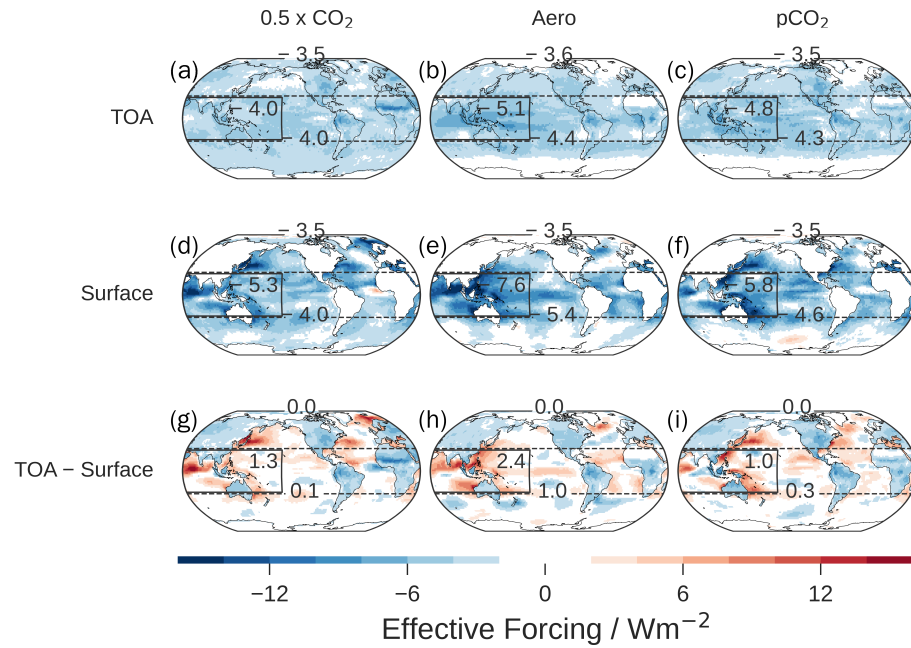
Figure B.4: Effective forcing of the radiatively forced simulations at TOA (row 1), surface (row 2), and their difference (row 3). The difference between TOA and surface effective forcing is the effective forcing on the atmosphere, and can be interpreted as a redistribution of negative forcing from blue to red regions, when going from the TOA to the surface. WP and tropics are shown with solid and dashed lines, and the field average over these regions is shown in the WP box and in the dashed line, respectively. The global mean is shown at the top of each panel. The standard errors are generally negligible compared to the shown precision, except: WP mean of surface and TOA-surface: \approx 0.2 \text{ Wm}^{-2} , and tropical mean of surface and TOA-surface: \approx 0.1 \text{ Wm}^{-2} .
