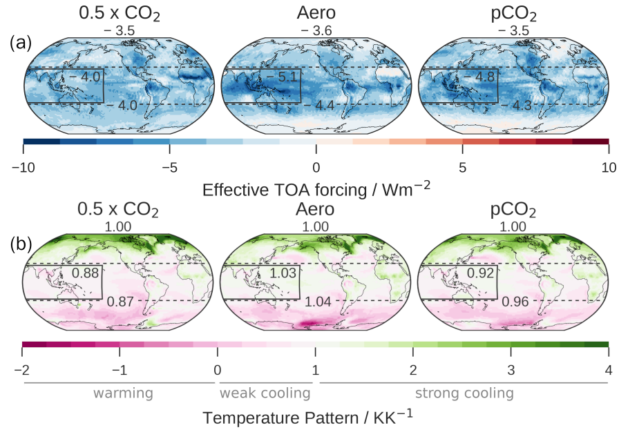
Figure B.3: (a) Annual-mean TOA effective forcing obtained from the difference between the forced simulations with fixed SST and the control simulation with fixed SST. (b) Ensemble-mean 2-meter temperature change patterns (ratio of local to global mean temperature change) of the radiatively forced, coupled simulations. Values greater than one (green) indicate stronger than global average cooling, lower than one (pink) weaker than average cooling. Values lower than zero indicate warming. WP and tropics are shown with solid and dashed lines, and the field average over these regions is shown in the WP box and in the dashed line, respectively. The global mean is shown at the top of each panel. Standard errors are negligible compared to the shown precision in (a). In (b), standard errors of the means over the WP and the tropics are \approx 0.04 - 0.05 \text{ KK}^{-1} .
