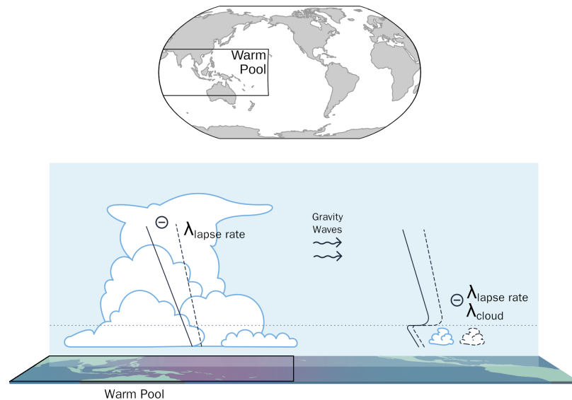
Figure 2.2: Top: Location of the Warm Pool (WP). Bottom: The pattern effect of the tropical Pacific Ocean. Solid lines represent the lapse rates of the climate base state, dashed lines a hypothetical state that follows from surface warming of the warm pool, which is located in the left half of the figure. Minus signs represent the negative lapse rate and cloud feedbacks.
