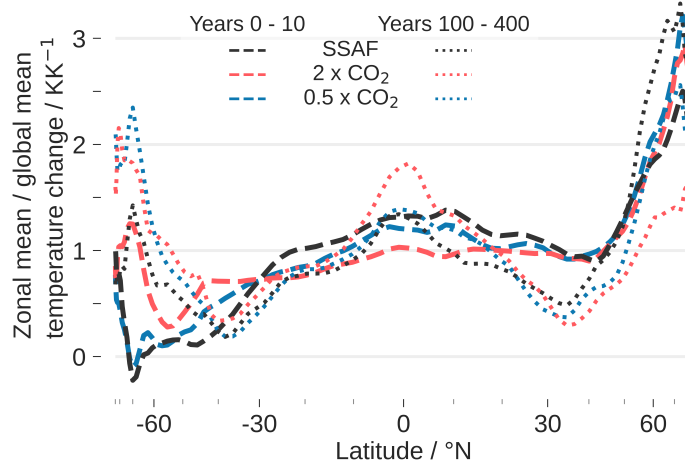
Figure A.3: Zonal mean temperature change pattern for the early (years 0 - 10) and the late (years 100 - 400) period. Values greater than one indicate stronger temperature change than the global average. A value of zero indicates no temperature change.
