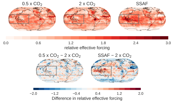
Figure A.6: Relative effective forcing (effective forcing normalized by its global average). The lower panels show the difference to the 2 \times \text{CO}_2 simulation. The solid and dotted lines indicate the boundaries of the warm pool region and the tropics, respectively.
