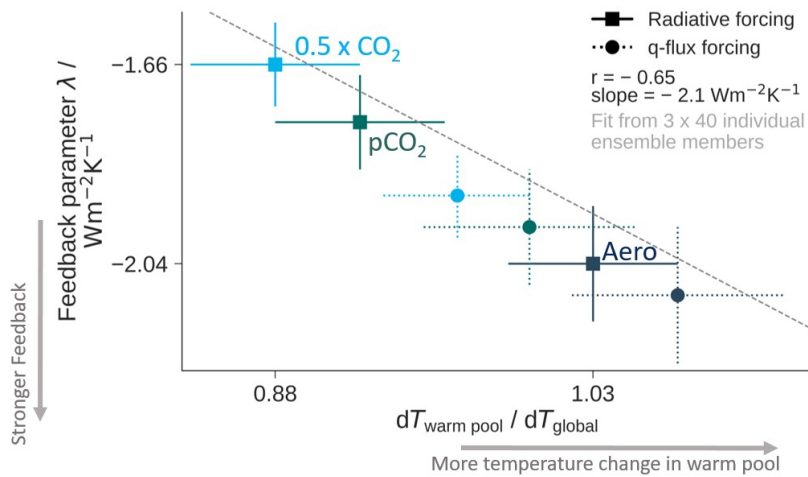
Figure 4.2: Scatter plot of feedback parameter vs ratio of WP mean to global mean temperature change. Squares represent results from the radiatively forced simulations (described in chapter 3). The circles are from the q-flux-forced simulations, which I discuss in section 4.6. Feedback parameters and associated standard errors are calculated by regression over 10 years, followed by ensemble averaging. The gray dashed line is a linear regression through the feedback parameter values from all 3 \times 40 = 120 ensemble members from the first decade.
