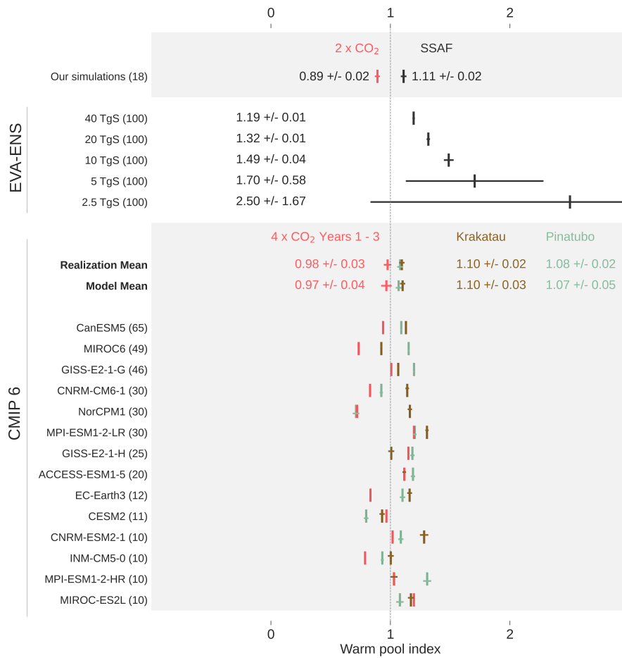
Figure A.7: Comparison of the WPI in our 18-member, 10-years ensemble of idealized SSAF simulations, simulations from EVA-ENS, and volcanic periods of the CMIP6 historical simulations. Numbers in parentheses indicate the number of ensemble members, models with less than 10 members are not shown. Error bars represent standard errors and are slightly shifted up and down in order to avoid indistinguishable overlaps. For 4 x CO 2 there are generally only one or a few realizations per model. The errorbar of the 2.5 TgS EVA-ENS simulations exceeds the figure limits.
