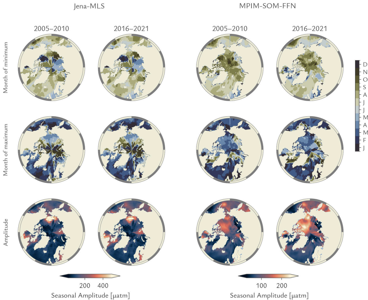
Figure B.5: Timing (month) of the ocean surface p\text{CO}_2 minimum (top row) and maximum (middle row) as well as the amplitude (bottom row) for different 5-year periods. Note the different color map extents of the amplitudes. The cyclic color bar representing the maps of timing equates dark shading with winter months and lighter shadings with summer months.
