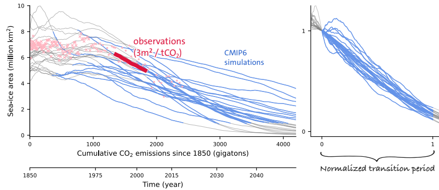
Figure 1.3: Time series of September SIA and its sensitivity to changes in anthropogenic CO 2 emissions (with permission from Stolla, 2023; labels modified). The left panel shows the data from both observations and model simulations. The thick red line marks the 30-year running average of the observations (light red markers), and the thin lines mark the 30-year running averages of the model simulations. The blue segments of the model data highlight the period in which the running average is between the 90th percent threshold and the 1 million km 2 minimum, defined as the transition period in Notz and Stroeve (2016). The right panel shows the normalized values of the model simulations, starting the transition period at x = 0 and ending at x = 1 . The SIA on the y -axis was normalized such that their value at the start of the transition period is at y = 1 .
