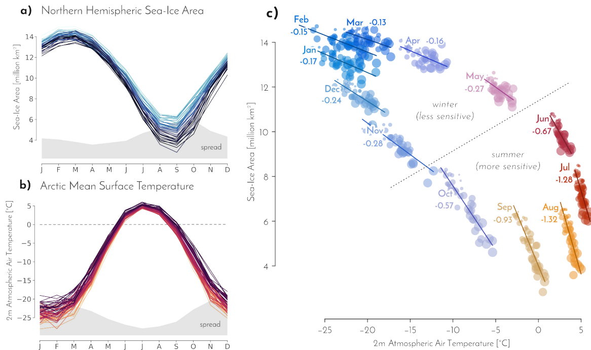
Figure A.3: Left: Seasonal cycles of (a) NH SIA and (b) Arctic mean TAS over time. Darker shadings represent more recent time steps. The grey-shaded area represents the spread of the respective month across the entire time series from 1979 to 2022. Right, (c): Monthly sensitivities of NH SIA (averaged across the three data products) with respect to spatially averaged Arctic TAS. Values denote the respective seasonal sensitivity in million \text{km}^2/\text{°C} . Markers of one month share the same color, with their size increasing over time. The breakpoints between May/June and October/November separate the seasonal cycle into a winter and a summer season.
