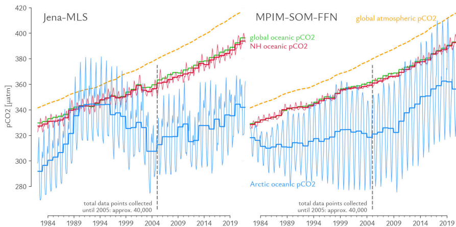
Figure B.3: Time series of atmospheric global (orange), and oceanic global (green), northern-hemispheric (red) and Arctic (blue) p\text{CO}_2 for Jena-MLS (left) and MPIM-SOM-FFN (right).
