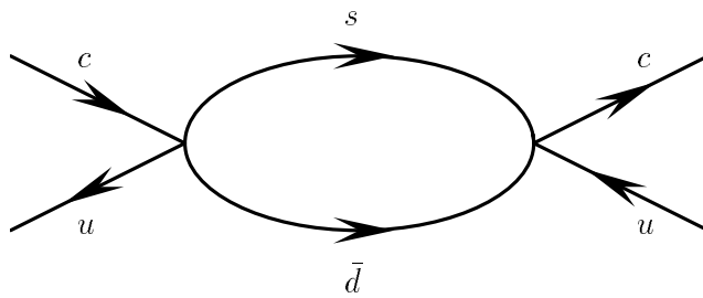
Figure 2: The diagram for the contribution of Pauli interference in the decays of charmed quark for the \Xi_{bc}^+ baryon.
