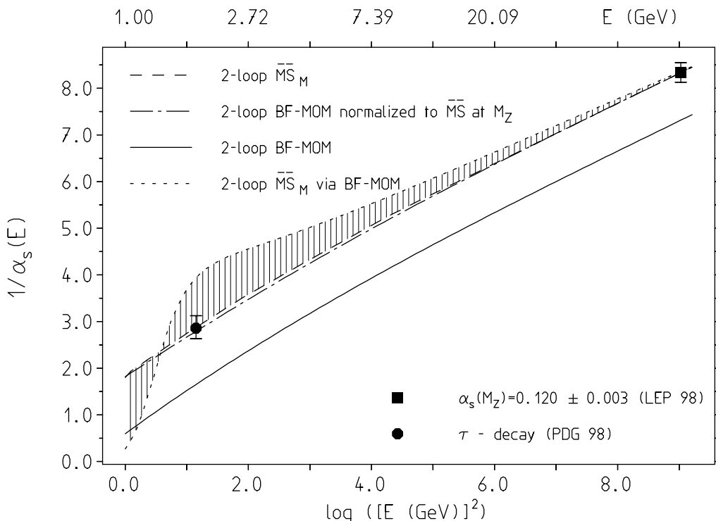
Figure 3: Comparison of \alpha_s in the BF – MOM and the \overline{\text{MS}} schemes with \alpha_s^{(5)}_{\overline{\text{MS}}} = 0.12 at scale M_Z = 91.19 GeV and \alpha_s_{\text{BF-MOM}} at this scale calculated using (23). The dotted line is the \overline{\text{MS}} coupling calculated from \alpha_s_{\text{BF-MOM}}(E) by inverting (23).
