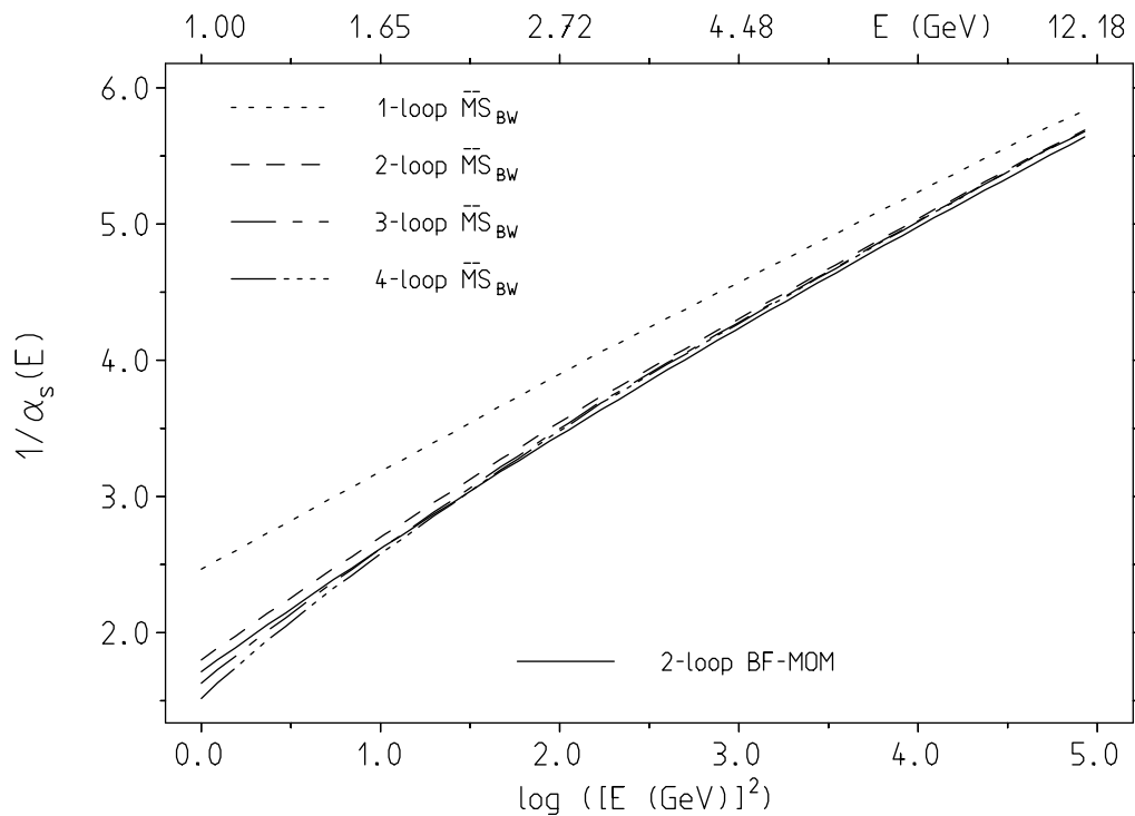
Figure 2: Comparison of the \alpha_s evolution in the space-like region normalized to a common value \alpha_s = 0.12 at scale M_Z = 91.19 GeV. The dotted, dashed, dash-dot and the dash-dot-dot-dot curves show, respectively, the one-loop, two-loop, three-loop and the four-loop \overline{\text{MS}} evolution for BW-matching. The full line represents the exact BF – MOM running coupling.
