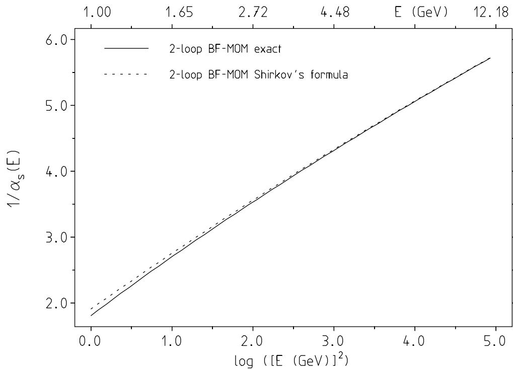
Figure 1: Evolution of \alpha_s in the BF – MOM scheme normalized to \alpha_s = 0.12 at the scale M_Z = 91.19 GeV. The dotted line represents the approximation by Shirkov's formula.
