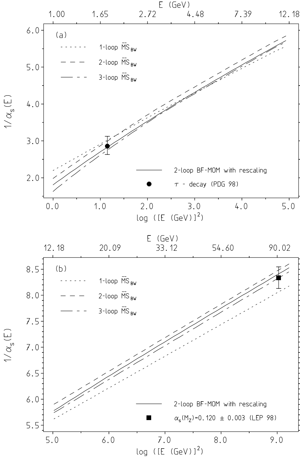
Figure 4: Comparison of \alpha_s((x_0 E)^2) in the BF – MOM and \alpha_s(E^2) in the \overline{\text{MS}} scheme with input values \alpha_s^{(5)\overline{\text{MS}}} = 0.120 at scale M_Z=91.19 GeV and \alpha_{s \text{ BF-MOM}} = 0.1189 obtained for the rescaled energy x_0 M_Z \simeq 190.90 GeV ( x_0 \simeq 2.1044 ).
