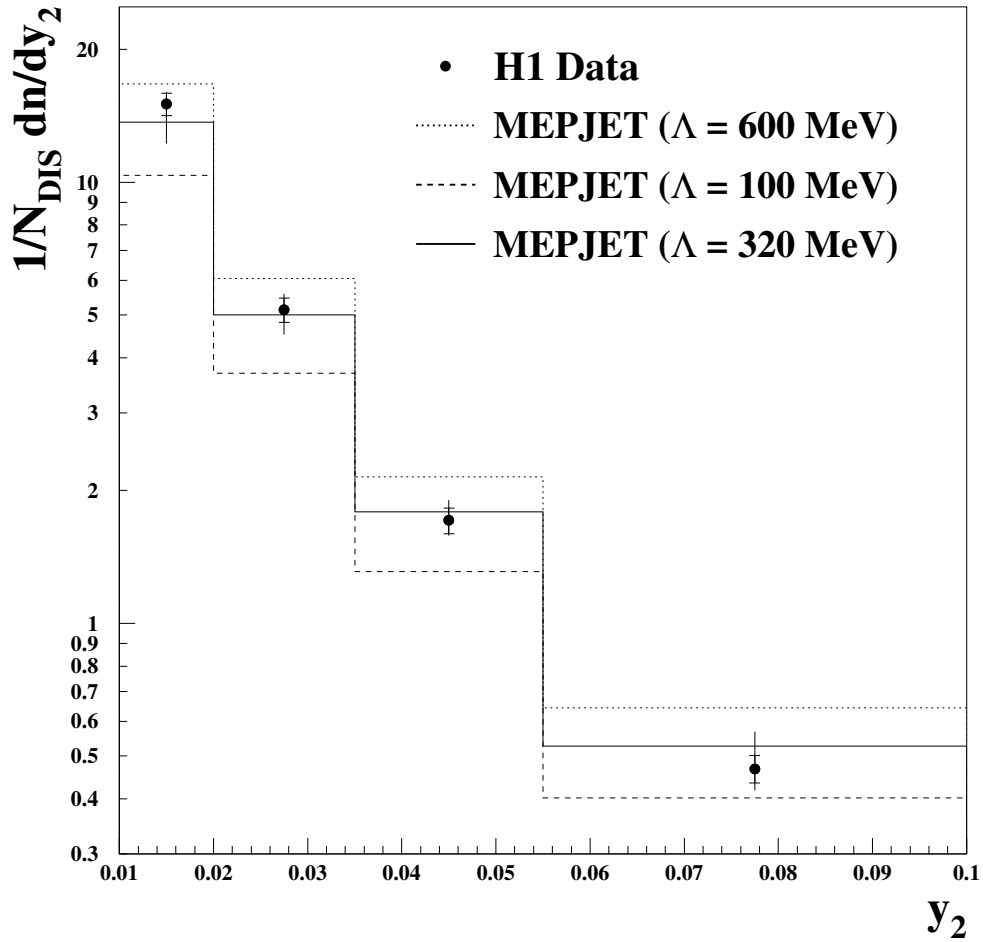
Figure 5: Distribution of the differential jet rate y_2 corrected for detector and hadronization effects compared with the NLO prediction of MEPJET for \Lambda_{\overline{MS}}^{(4)} = 600 \text{ MeV} (dotted line) and \Lambda_{\overline{MS}}^{(4)} = 100 \text{ MeV} (dashed line). The full line shows the NLO prediction for the fitted value of \alpha_s which corresponds to \Lambda_{\overline{MS}}^{(4)} = 320 \text{ MeV} . The error bars on the corrected data distribution correspond to the statistical and systematic errors added in quadrature. The inner error bars give the statistical error only.
