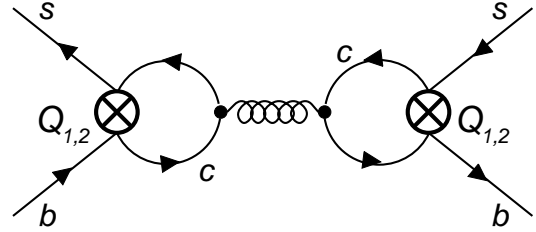
Figure 4: Penguin diagram contribution to \Gamma^{\text{non-spec}}(B_s) . The final state corresponds to a cut through either of the (\bar{c}, c) -loops. The contributions of Q_1 vanish by colour. This is the only NLO contribution to \tau(B_s)/\tau(B_d) - 1 involving Q_{1,2} without suppression factors of \Delta or z .
