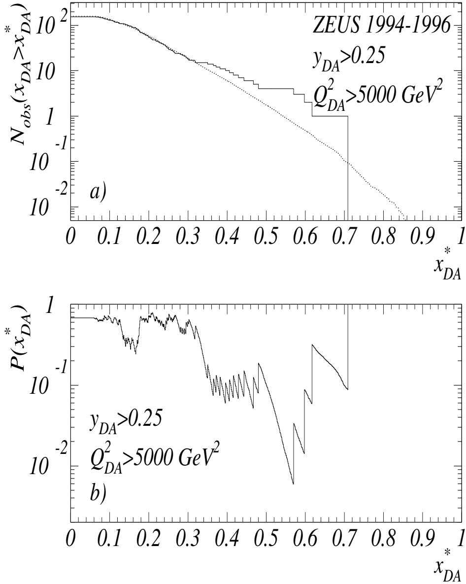
Figure 7: In (a), the solid line indicates the number of events observed with y_{DA} > 0.25 and x_{DA} > x_{DA}^* as a function of x_{DA}^* . The dotted line indicates the number of expected e^+p NC DIS events with y_{DA} > 0.25 and x_{DA} > x_{DA}^* . In (b) is shown the Poisson probability (eqn. 11) to observe at least as many events as were observed with x_{DA} > x_{DA}^* as a function of x_{DA}^* .
