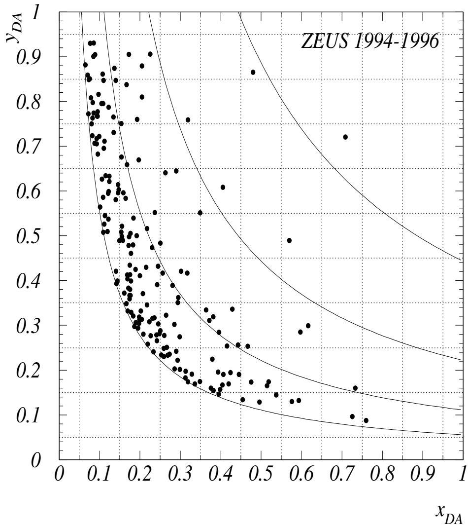
Figure 1: The distribution of the event sample in x_{DA} and y_{DA} . The lines indicate constant values of Q_{DA}^2 = x_{DA} y_{DA} for Q_{DA}^2 = 5000, 10000, 20000 and 40000 \text{ GeV}^2 .
