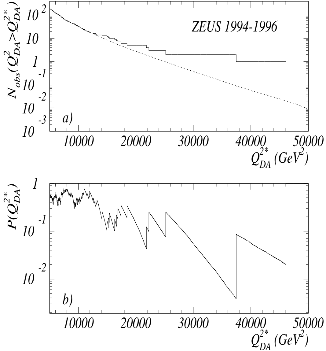
Figure 6: In (a), the solid line indicates the number of observed events with Q_{DA}^2 > Q_{DA}^{2*} as a function of Q_{DA}^{2*} . The dotted line indicates the number of events expected from e^+p NC DIS with Q_{DA}^2 > Q_{DA}^{2*} . In (b) is shown the Poisson probability (eqn. 11) to observe at least as many events as were observed with Q_{DA}^2 > Q_{DA}^{2*} as a function of Q_{DA}^{2*} .
