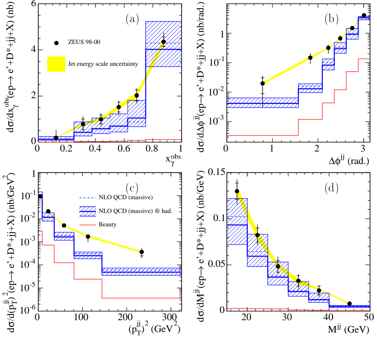
Figure 9: Dijet cross-sections (a) d\sigma/dx_\gamma^{\text{obs}} , (b) d\sigma/d\Delta\phi^{\text{jj}} , (c) d\sigma/d(p_T^{\text{jj}})^2 and (d) d\sigma/dM^{\text{jj}} for the data (solid dots) compared to massive QCD predictions with (solid line) and without (dotted line) hadronisation corrections applied. The theoretical uncertainties (hatched band) come from the change in scales simultaneously with the change in charm mass. The beauty component is also shown (lower histogram).
