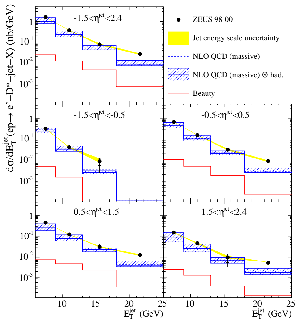
Figure 3: Cross-section d\sigma/dE_T^{\text{jet}} for jets in events (dots) containing at least one D^* meson for different regions in \eta^{\text{jet}} . The comparison is made to massive QCD predictions with (solid line) and without (dashed line) hadronisation corrections applied. The theoretical uncertainties (hatched band) come from the change in scales simultaneously with the change in charm mass. The beauty component is also shown (lower histogram).
