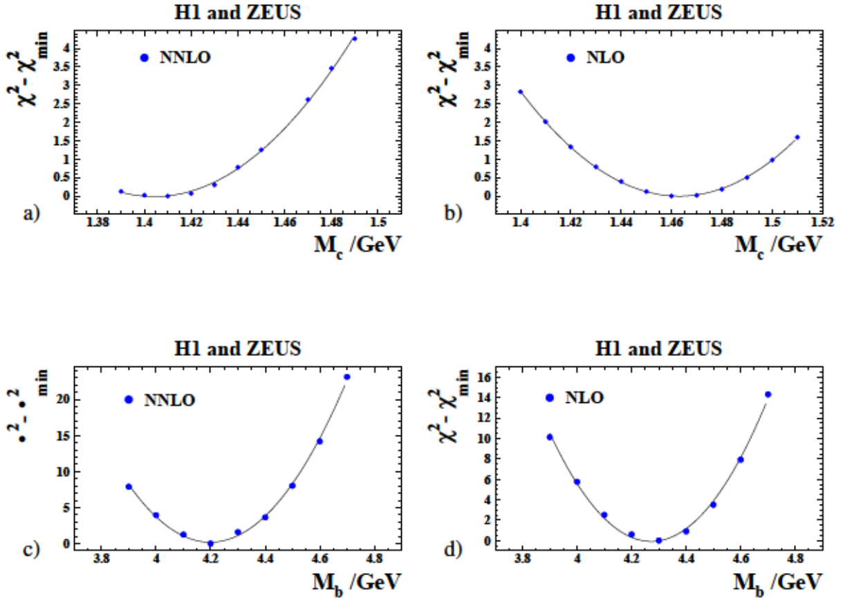
Figure 1: Difference between \chi^2 and \chi^2_{\min} versus a) M_c for M_b = 4.2 \text{ GeV} at NNLO with \alpha_s(M_Z^2) = 0.1155 , b) M_c for M_b = 4.3 \text{ GeV} at NLO with \alpha_s(M_Z^2) = 0.118 , c) M_b with M_c = 1.41 \text{ GeV} at NNLO with \alpha_s(M_Z^2) = 0.1155 , d) M_b with M_c = 1.46 \text{ GeV} at NLO with \alpha_s(M_Z^2) = 0.118 .
