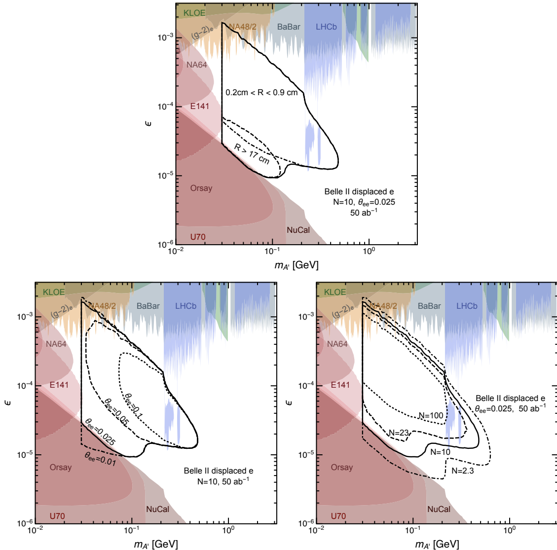
Figure 3: Expected sensitivity of the search for displaced electron final states at Belle II in the \epsilon - m_{A'} parameter plane for an integrated luminosity of 50 \text{ ab}^{-1} . In the top panel we show the individual sensitivities corresponding to the regions in which 0.2 \text{ cm} < R < 0.9 \text{ cm} (dash-dotted), 17 \text{ cm} < R < 60 \text{ cm} (dashed) and the sensitivity for both regions combined (solid) for 10 events and an angular cut \theta_{ee} = 0.025 . In the bottom panel we show the sensitivity for 10 events and different angular cuts \theta_{ee} (left) and a varying number of events for \theta_{ee} = 0.025 (right). Existing limits are taken from [44].
