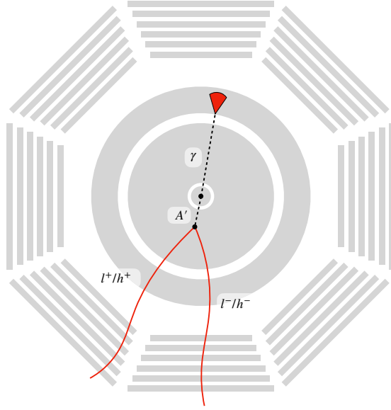
Figure 1: Schematic view of the Belle II detector ( xy -plane) and example displaced signature e^+e^- \rightarrow \gamma A', A' \rightarrow l^+l^-/h^+h^- ( l^\pm = e^\pm, \mu^\pm and h^\pm = \pi^\pm, K^\pm ).
