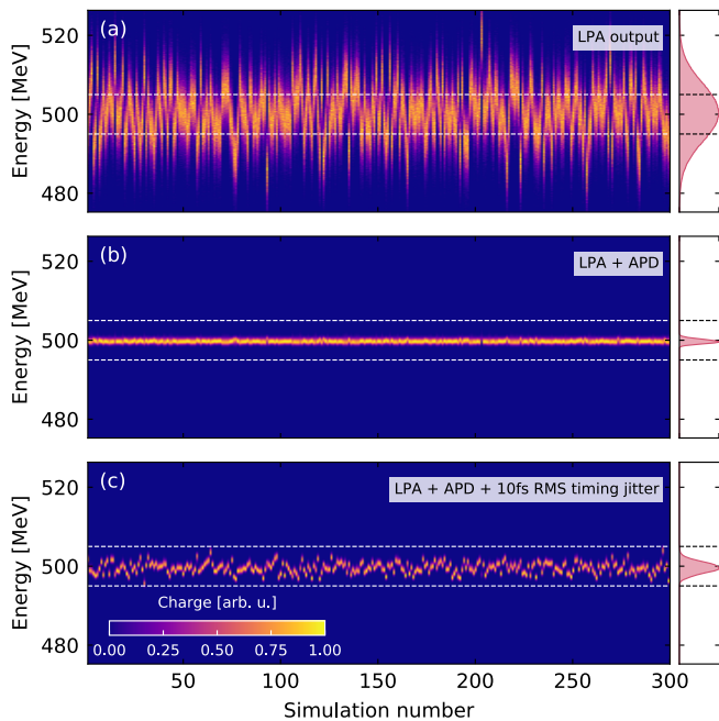
FIG. 3. Energy spectrum of 300 simulated beams with an initial 1% rms energy jitter and energy spread. (a) Initial spectrum of the Gaussian beam emulating the LPA output. (b) Final spectrum after lengthening and active dechirping. (c) Same as (b) but with a 10 fs rms timing jitter in the APD driver. The dashed lines represent a \pm 1\% energy deviation.
