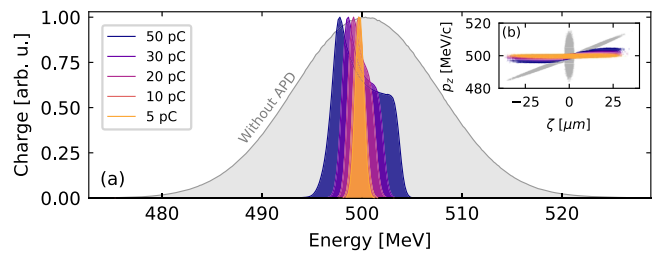
FIG. 4. (a) Energy spectrum of the LPA output with and without an APD for different values of the beam charge. Each curve is the projection of 300 simulations with an initial 1% rms energy jitter. (b) Final longitudinal phase space of beams with \langle \delta_i \rangle = 0 . Higher charge can lead to non-linearities due to beam loading. For reference, the phase space at the LPA and chicane exit is also included (gray).
