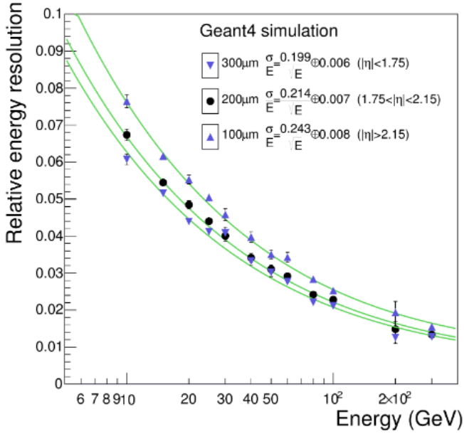
Figure 9.5: Energy resolution as a function of energy from a standalone simulation of incident electrons on HGCal, for different thickness of silicon sensors [203].
