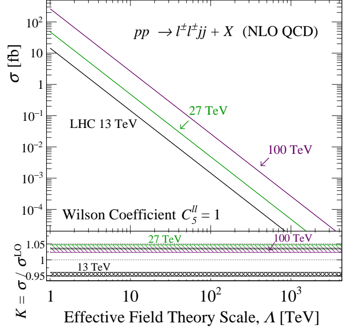
Figure 6.4: Cross section predictions at NLO in QCD for the W^\pm W^\pm \rightarrow \ell_i^\pm \ell_j^\pm process when mediated by the Weinberg operator for representative pp collider energies [78].
