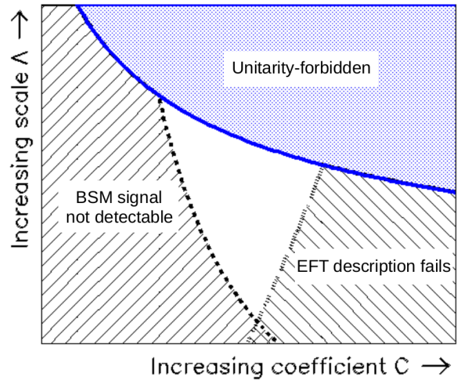
Figure 5.1: For a Wilson coefficient C and EFT cutoff scale \Lambda , a sketch of the regions in \Lambda – C space that are forbidden by unitarity (large \Lambda and large C ), are inconsistent with the assumptions of EFTs (small \Lambda and large C ), and are inaccessible to experiments (small C and/or large \Lambda ). Adapted from Ref. [115].
