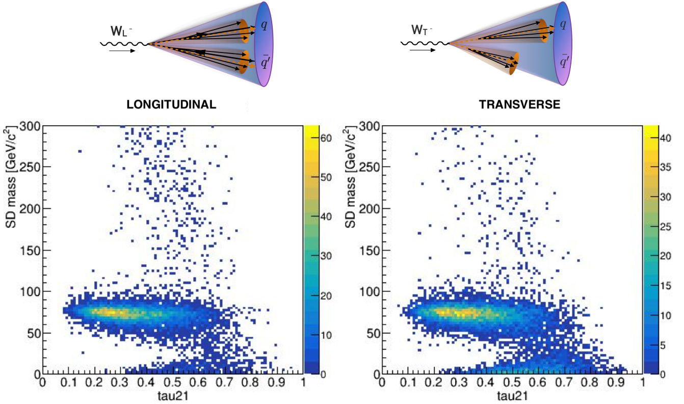
Figure 7.2: Top: Illustration of the decays of high- p_T W_L (Left) and W_T (Right) bosons in the lab frame showing that overlapping decay products are preferentially symmetric (for W_L ) or asymmetric (for W_T ) due to spin correlation. Lower: Scatter plot of the soft drop (SD) mass variable as a function of the “ N -subjettines” variable \tau_{21} for W_L (Left) and W_T (Right). Transversely polarized vector bosons (right) more frequently get reconstructed with a soft drop mass of zero and a 1-prong like substructure (i.e. larger \tau_{21} values) due to its decay products being emitted anti-parallel to the W momentum and falling out of the jet cone during the grooming process [172, 173].
