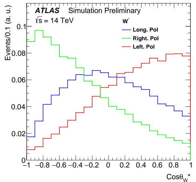
Figure 4.9: Normalized W^- polarization state templates at the reconstruction level and after the final event selection, including requiring m_{jj} > 600 GeV. Figure from Ref. [110].
