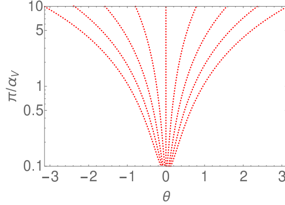
Figure 6: Flow of \pi/\alpha_V(\theta, \mu) for different initial values of \theta for t increasing from top to bottom.
