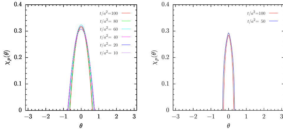
Figure 8: The Polyakov loop susceptibility as a function of \theta on the 16^4 (left) and the 32^4 lattice (right) for flow times ranging from t/a^2 = 10 to 100.
