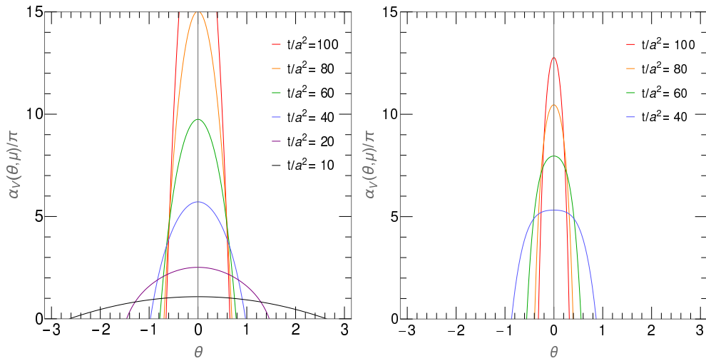
Figure 5: The running coupling \alpha_V(\theta, \mu) as a function of \theta on the 16^4 (left) and the 32^4 lattice (right) for flow times ranging from t/a^2 = 10 (bottom) to 100 (top). Note that \alpha_V \simeq 0.729 \alpha_{GF} .
