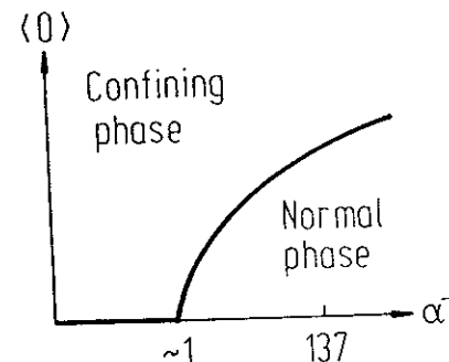
Figure: Speculated phase diagram for QED in the presence of a strong external electromagnetic field.
