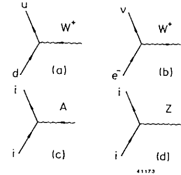
Figure 1: Charged current, QED, and neutral current interactions. The vertex factors are (a) -\frac{ig}{2\sqrt{2}}\gamma_\mu(1+\gamma^5)V_{ud} , (b) -\frac{ig}{2\sqrt{2}}\gamma_\mu(1+\gamma^5) , (c) -ieq_i\gamma_\mu , and (d) -\frac{ig}{2\cos\theta_W}\gamma_\mu[t_{3L}(i)(1+\gamma^5)-2\sin^2\theta_Wq_i] . V_{ud} is an element of the quark mixing matrix, q_i is the electric charge of fermion i (in units of e ), and t_{3L}(i) , the eigenvalue of the third generator of SU_2 , is +\frac{1}{2} for (u, \nu) and -\frac{1}{2} for (d, e^-) .
