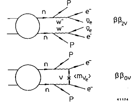
Figure 14: Diagrams for two neutrino ( \beta\beta_{2\nu} ) and neutrinoless ( \beta\beta_{0\nu} ) double beta decay.
