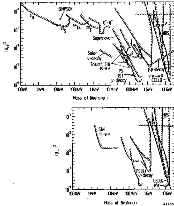
Figure 12: Limits on the mass and mixing of heavy neutrinos, from [97].
