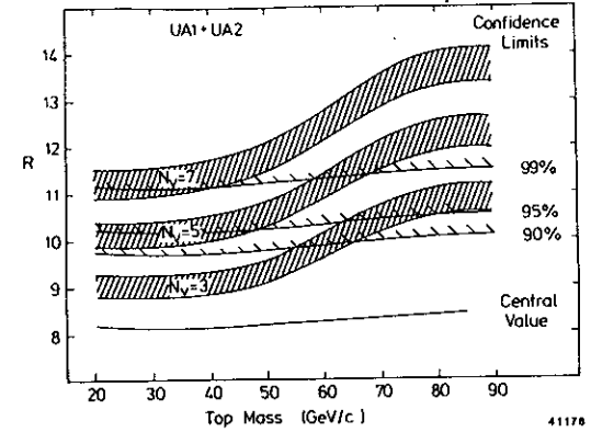
Figure 10: The value of R (27) as a function of N_\nu and m_t , and the experimental results from UA1 and UA2.
