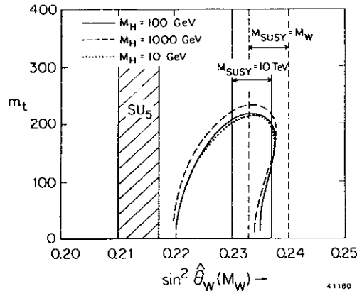
Figure 8: Allowed regions (90% c.l. ) in \sin^2 \hat{\theta}_W(M_W) and m_t for fixed values of M_H . Also shown are the predictions of ordinary and supersymmetric GUTs, assuming no new thresholds between M_W or M_{SUSY} and the unification scale.
