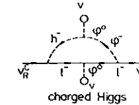
Figure 11: Dirac, pure Majorana, induced, and charged Higgs generated neutrino masses.
