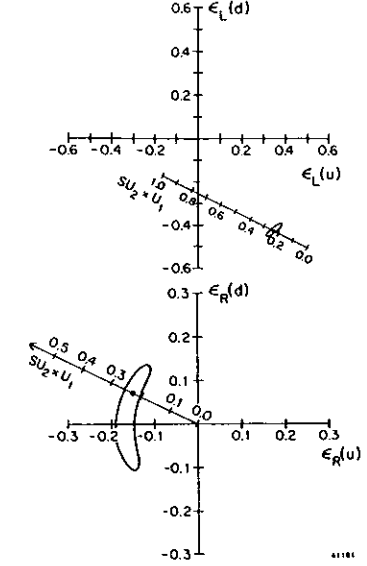
Figure 5: Allowed regions at 90% c.l. for the (weak) model independent \nu q parameters \epsilon_i(u) and \epsilon_i(d) , i = L or R and the predictions of the standard model as a function of \sin^2 \theta_W .
