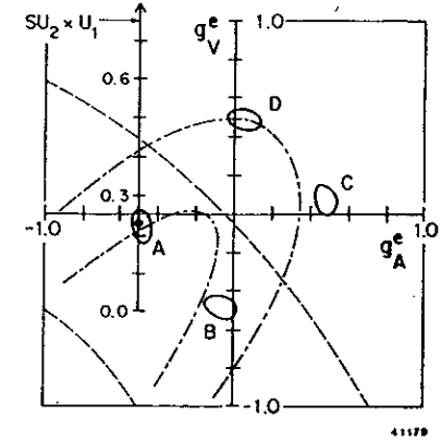
Figure 6: Allowed regions (90% c.l.) for the \nu e parameters g_V^e and g_A^e , for \bar{\nu}_\mu e (solid lines), reactor \bar{\nu}_\mu e (dot-dash), and \nu_e e (dash).
