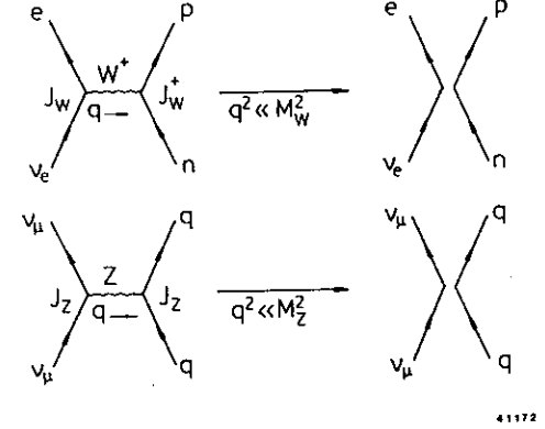
Figure 2: The effective four-fermion interactions for \nu_e n \rightarrow e^- p and \nu_\mu q \rightarrow \nu_\mu q .
