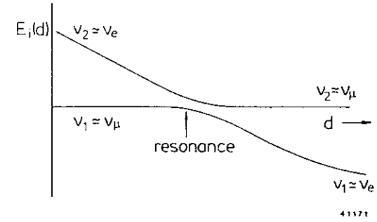
Figure 15: The energy eigenvalues of M' as a function of d , the distance from the center of the Sun.
