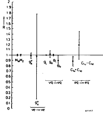
Figure 4: Experimental values of the W and Z masses and the neutral current couplings, relative to the standard model predictions for the global best fit value \sin^2 \theta_W = 0.230 (the value of g_L should be regarded as the major determinant of \sin^2 \theta_W rather than a prediction). C_{ii} , i = u, d are the coefficients in -L_{eff}^{NC} of the parity-violating eq interaction \frac{G_F}{\sqrt{2}} \bar{\nu} \gamma_\mu \gamma^5 \epsilon \bar{q}_i \gamma^\mu q_i . The other quantities are defined in the text. The error bars on g_V^e are large only because the predicted value ( -0.045 ) is so small.
