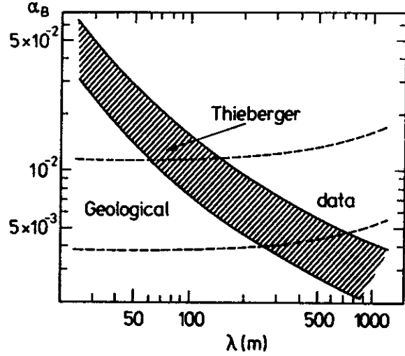
Figure 3: Allowed values of \alpha_B for Thieberger's experiment, plotted versus \lambda_B . The range for \alpha_B suggested by the geological data of [8] is also indicated
