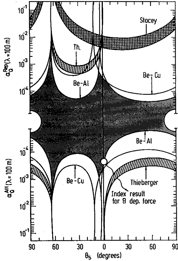
Figure 5: Bounds for \alpha_Q , at \lambda_Q = 100m , obtained by the experiment of Stubbs et al [11] and Adelberger et al [16]. Also indicated in the figure are the values of \alpha_B , at \lambda_B = 100m , obtained in the Index experiment [13], as well as the ranges allowed by the Thieberger result [12] and by the geological data (Stacey) [8]
