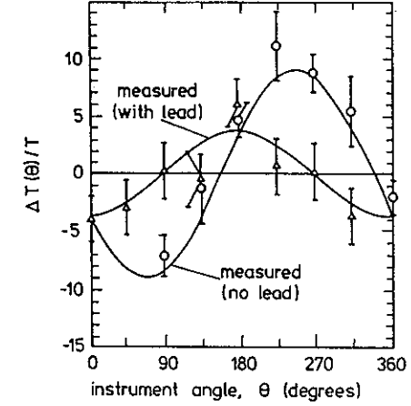
Figure 6: Results of the Index experiment for \frac{\Delta T(\theta)}{T} when the gravitational gradients are compensated (open triangles) and not compensated (open circles)
