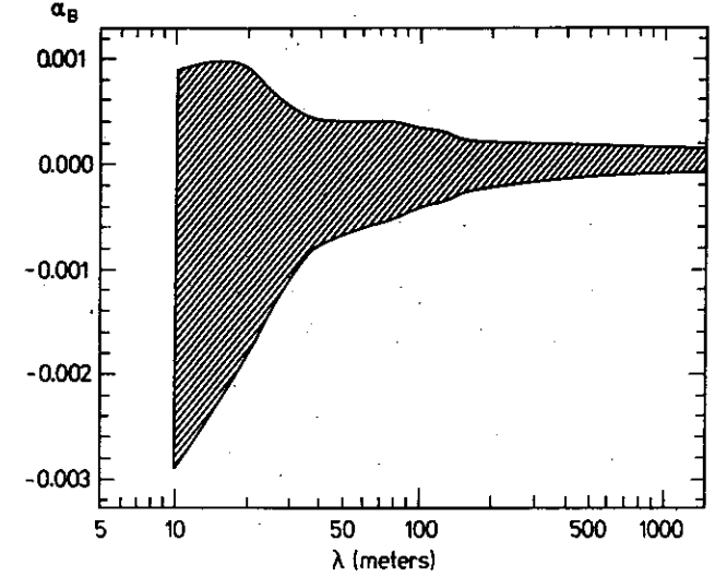
Figure 4: Allowed values of \alpha_B for the experiment of Stubbs et al [11], plotted versus \lambda_B
