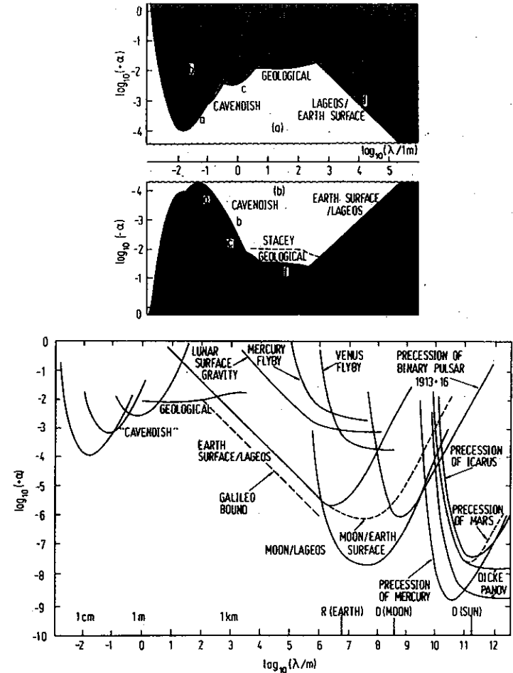
Figure 2: Compilation of bounds on \alpha and \lambda due to possible deviations of Newton law, from A. de Rujula [9]. The dotted line (Galileo bound) is the bound which arises from the results of [10], if one assumes that B -dependent 5^{th} forces exist
