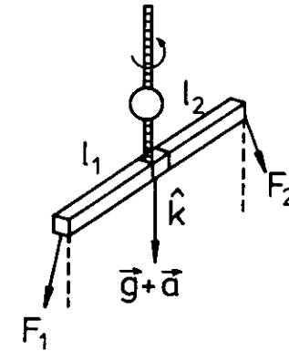
Figure 1: Schematic diagram of the Eötvös experiment
