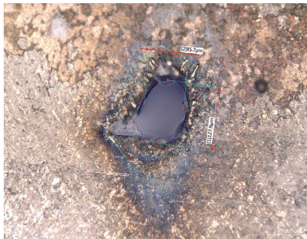
Figure 1 Microscope image of a burn-through hole in a steel cap generated by a 1.5 keV FEL beam
