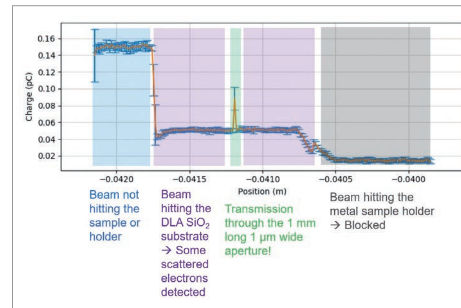
Figure 3 Charge measurement showing the transmission of the ARES electron beam through the 1 \mu\text{m} aperture of the ACHIP sample. The charge is measured by an intensity monitor downstream of the structure. When the beam is transmitted through the aperture (green area), the monitor measures the transmitted charge. In the purple area, electrons hit the sample and get scattered. In the grey area, the electrons are stopped by the sample holder.
