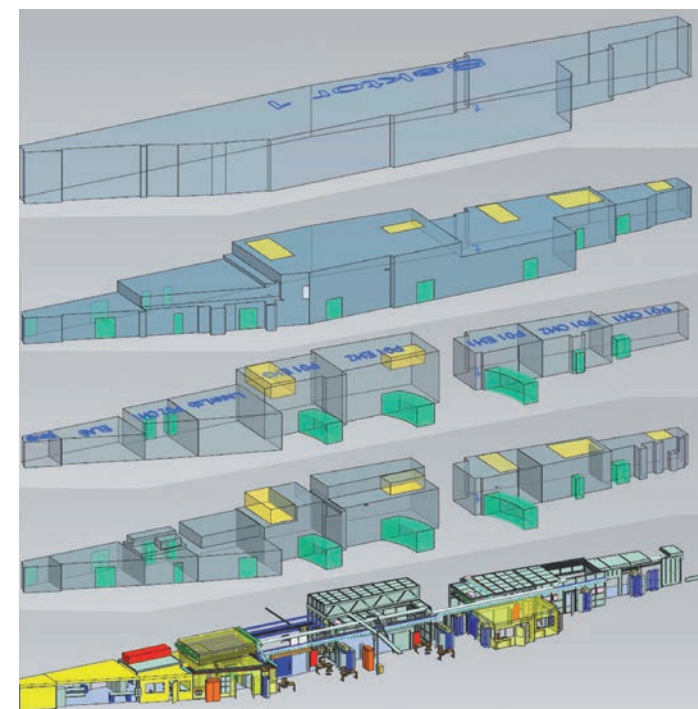
Figure 2 Sector 1 of the "Max von Laue" hall, from top to bottom, in detail grades (DG): DG1 (outline), DG2 (with interfaces), DG3 (interior) with huts in DG1, DG3 with huts in DG2, DG3 in full detail. Yellow areas designate crane transport routes, green areas indicate escape routes.
