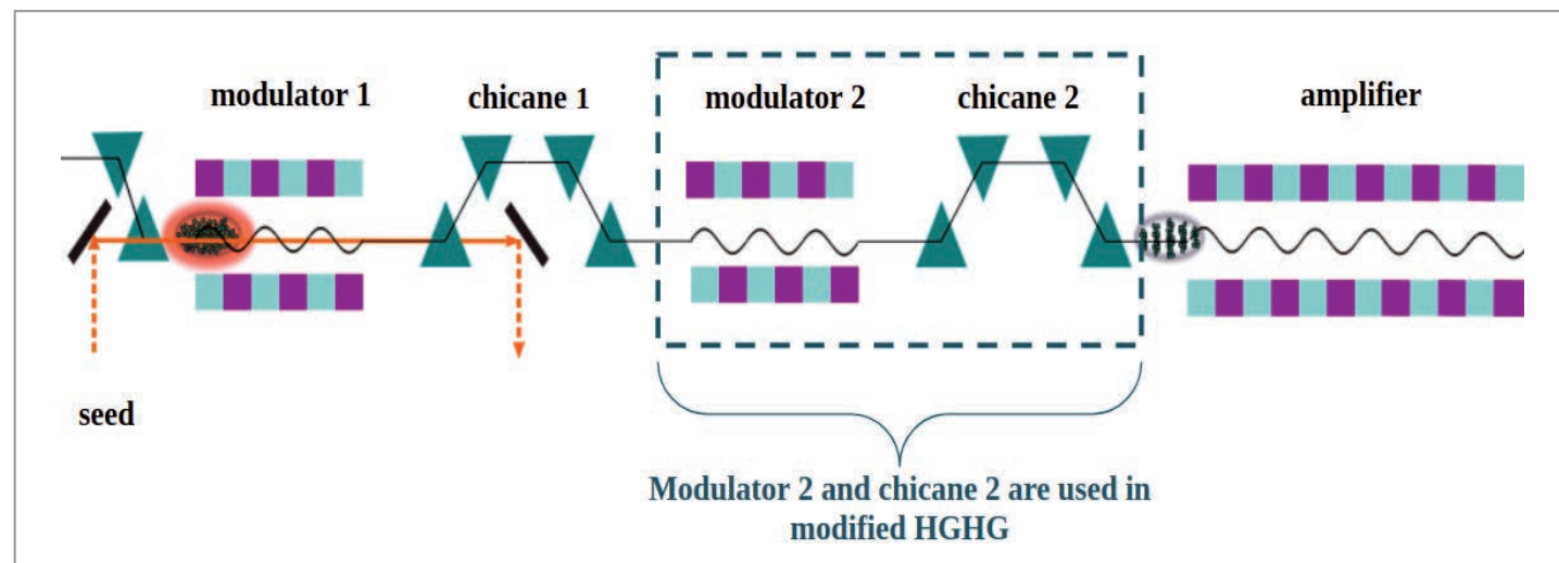
Figure 1 The standard HGHG scheme consists of one modulator undulator, one chicane and an amplifier and requires tens to hundreds of MW seed laser peak power to obtain FEL radiation at harmonics of the seed laser wavelength. By simply using in addition the modulator and chicane (as highlighted in the figure) that already exist in seeded FEL beamlines, the peak power requirements can be reduced by two orders of magnitude, allowing seed laser systems to operate at a higher repetition rate.
