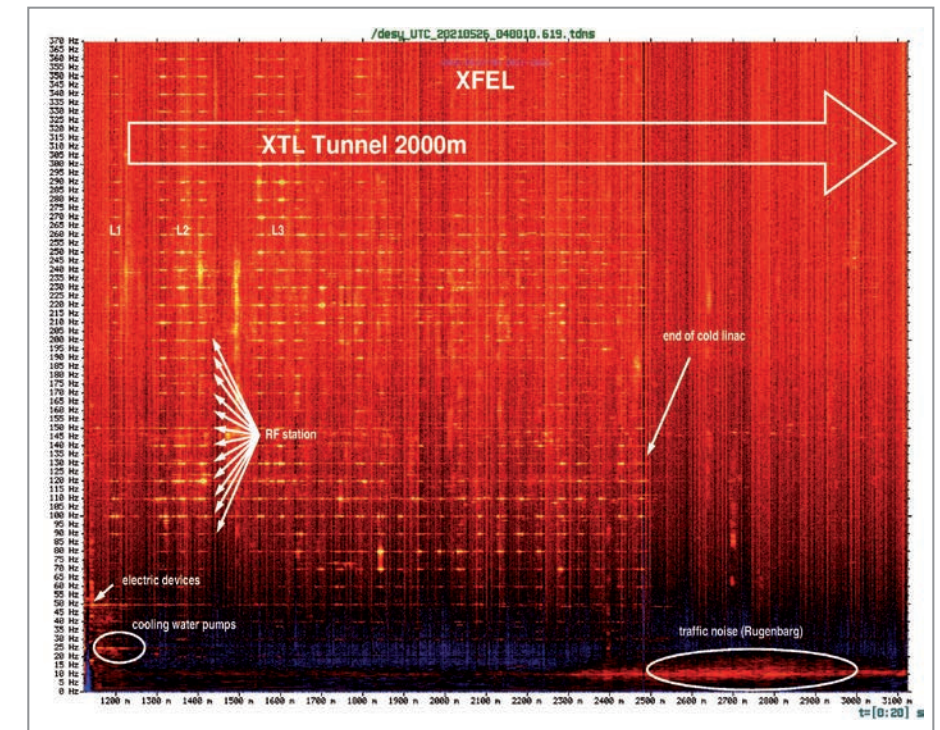
Figure 3 Spectra for all positions along the European XFEL tunnel during operation. The 10 Hz frequency ladders where the RF stations are located can clearly be seen.
