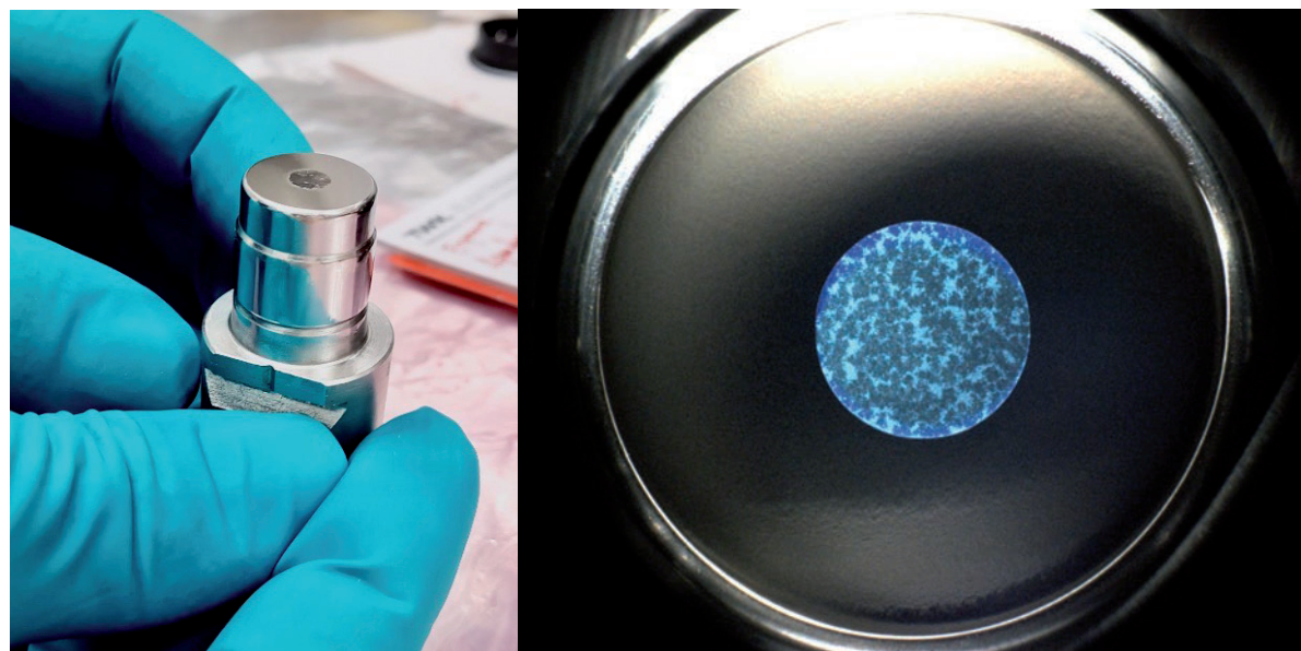
Figure 1 Left: Example of a FLASH Cs 2 Te photocathode designed, produced and analysed in the cathode lab at DESY. Right: Active area of the Cs 2 Te photocathode after deposition on the molybdenum plug (front view, plug diameter 16 mm, cathode diameter 5 mm).
