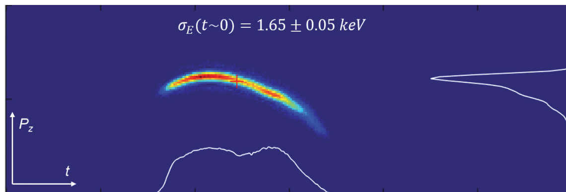
Figure 1 Slice energy spread measurements at PITZ show values much lower than those measured at higher-energy injectors (e.g. European XFEL, SwissFEL).
