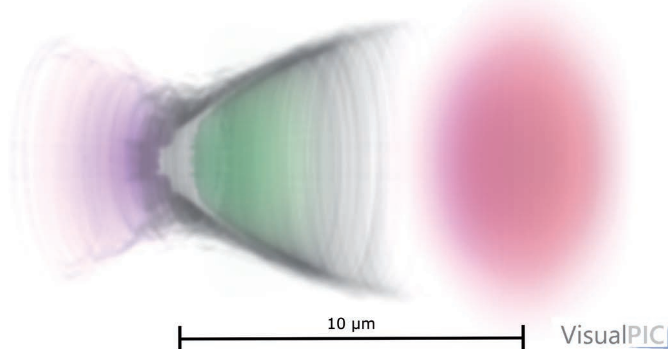
Figure 1 Schematic of laser plasma acceleration [2]. The laser (red) pushes away electrons (grey) so that a wakefield (green/purple) is created.
