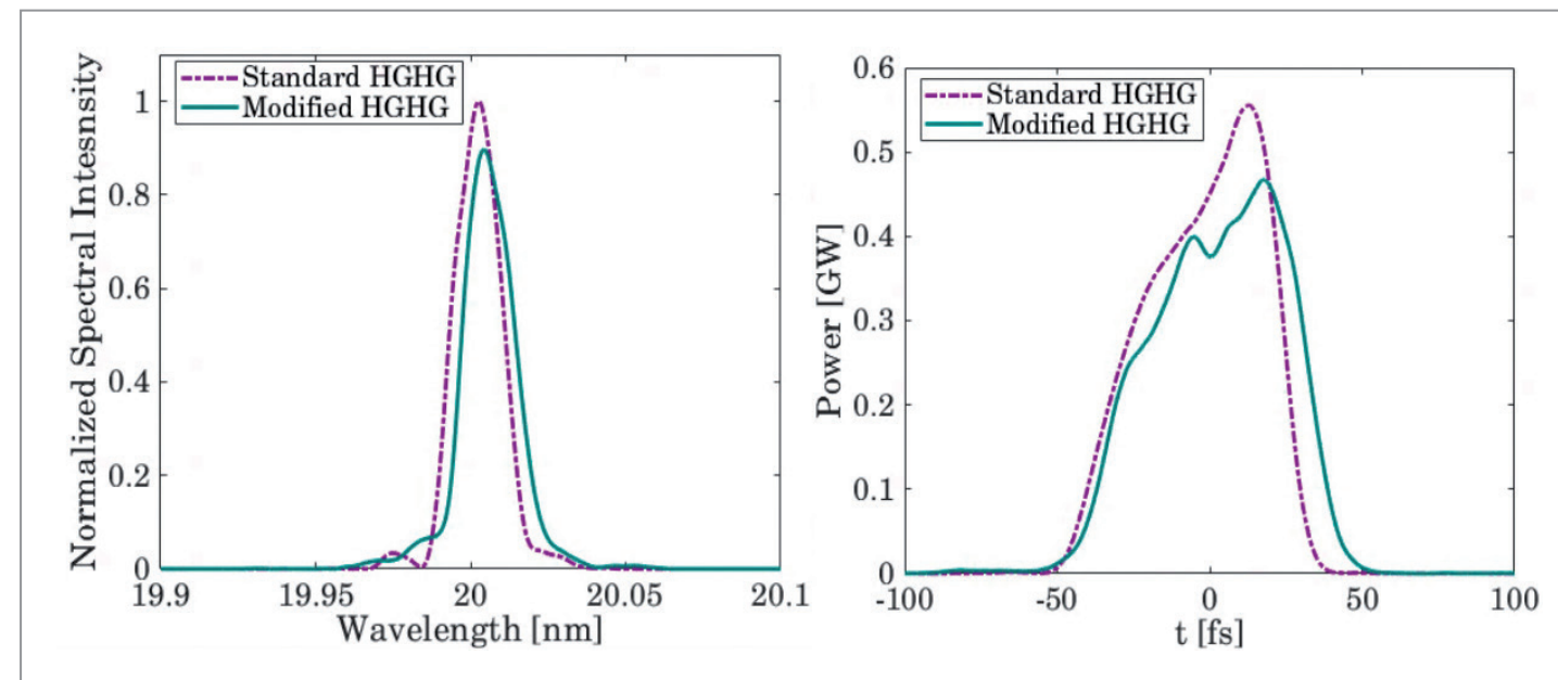
Figure 2 Comparison of the simulated output FEL radiation generated at the 15 th harmonic of a 300 nm seed laser. A seed laser peak power of 61 MW was used for the standard HGHG scheme, while only 0.17 MW were required for the modified HGHG scheme.
