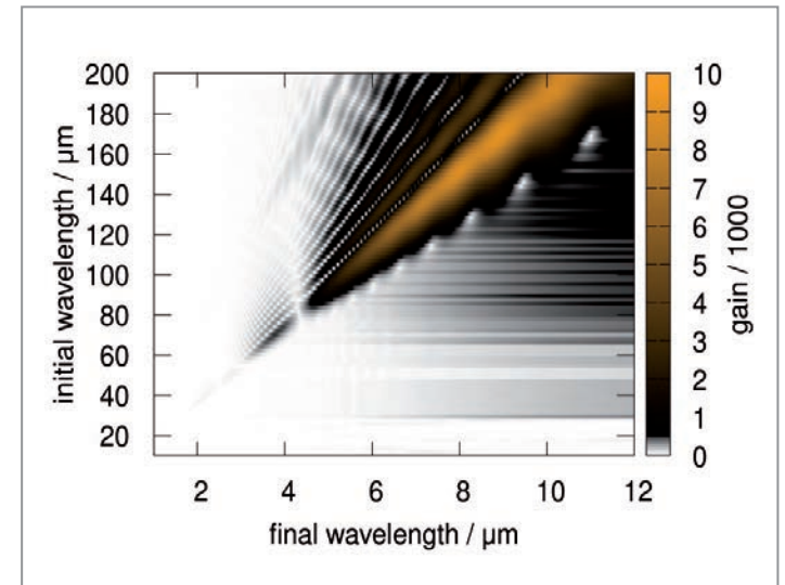
Figure 2 Example of a two-dimensional gain function calculated for FLASH2020+. Higher-order contributions are visible as additional bands next to the main diagonal.
