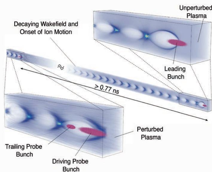
Figure 1 Conceptual representation of the plasma probe process. The rendering was performed using VisualPIC [1].
