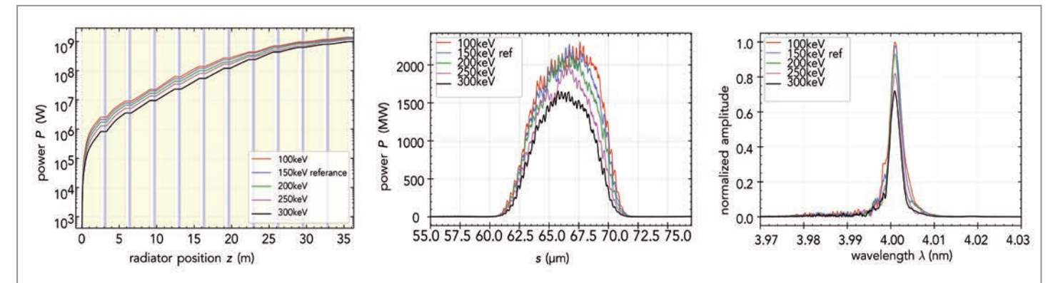
Figure 3 Sensitivity of an EEHG simulation for 4 nm with tapered radiators to the energy spread at the exit of the linear accelerator. Left: Power increase during propagation over 11 radiators. Centre: Power along the pulse behind the 11 th radiator. Right: Spectrum at the end of the radiator beamline.
