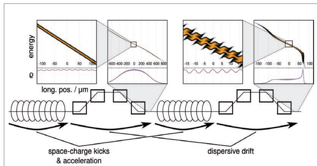
Figure 1 Sketch of the solvable microbunching model for a series of two bunch compression stages, each comprising accelerator modules and a magnetic chicane, together with plots of the phase space density and charge density \rho . Due to the microbunching mechanism, a small modulation of the initial charge density is converted into intricate substructures in the longitudinal phase space after the second stage.
