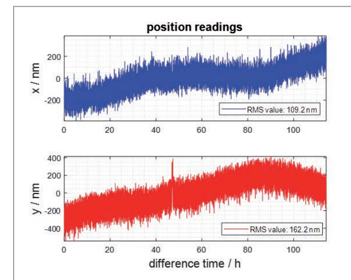
Figure 2 Evaluation measurements with the adapted Libera Brilliance+ readout electronics setup at PETRA III shown in Fig. 1, indicating that the long-term drifts in BPM position measurements in slow-acquisition data (0.1 Hz) over around four days in both transversal planes are well below the specification limit of 1 µm.
