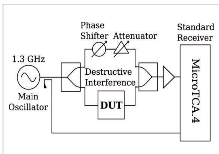
Figure 1 Simplified block diagram of the carrier-suppression-based receiver
