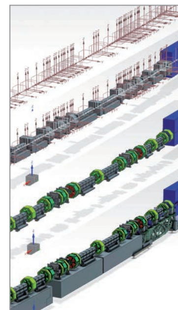
Figure 3 From lattice parametrisation to the full cell. From top to bottom: Coordinate systems of lattice components, DG1 models of accelerator components inserted, accelerator component conceptual models, vacuum system and supports added.
