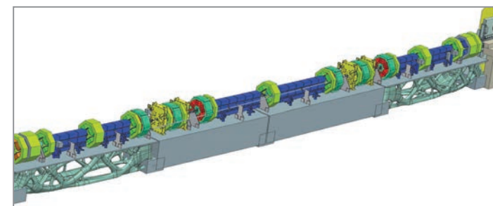
Figure 3 CAD model of the unit cell of the H6BA lattice
