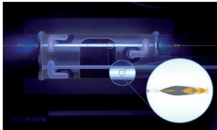
A 50 mm long plasma accelerator module in operation. The blue light is produced during the recombination of argon plasma after a high-voltage discharge. The magnification shows a simulated plasma wakefield corresponding to that of the FLASHForward experiment. It is generated by a leading electron bunch moving to the right; a trailing electron bunch is accelerated quickly and efficiently in it.
