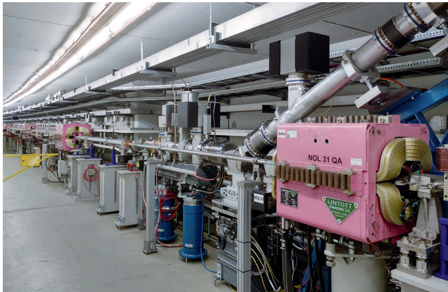
Figure 1 Dipole magnet and front-end components of the new dipole beamline P66 in the PETRA III tunnel
