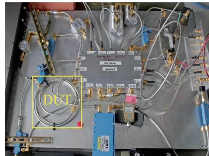
Figure 2 Setup of a carrier-suppression-based receiver prototype
