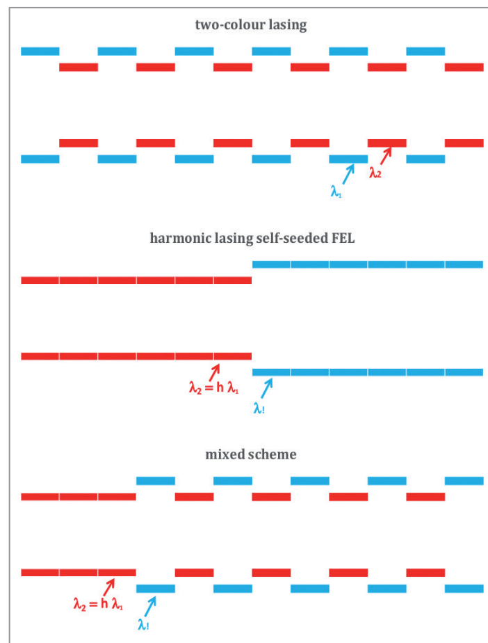
Figure 1 Tuning of the gaps of the undulator segments in the two-colour lasing scheme, the HLSS scheme and a mixed scheme used to optimise the setup to meet special experimental requirements
