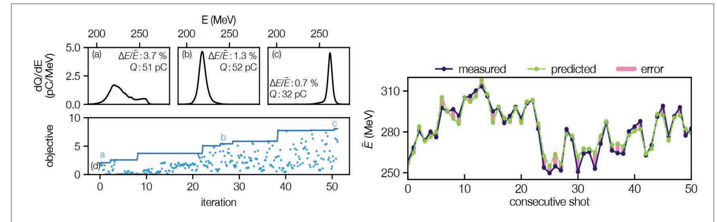
Figure 2 Application of machine learning at LUX: The left plot shows the evolution of the beam quality during the Bayesian optimisation procedure. As the algorithm does its work of maximising the objective, the spectra of the generated electrons (upper plot) become more and more narrow, resulting in a reduction of the energy spread. The right plot demonstrates the predictive capabilities of the neural network surrogate model. Using only the laser parameters as inputs, the model accurately predicts (green) the real measurements (blue) of the median electron energy. Figure adapted from [1] and [2].
