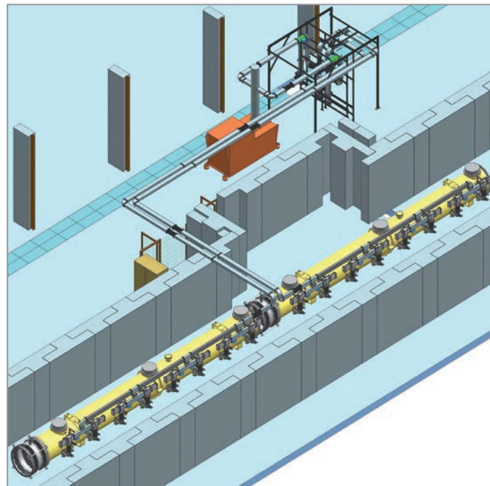
Figure 1 Design of the waveguide distribution between the RF station 1 and the accelerator modules ACC2 and ACC3
