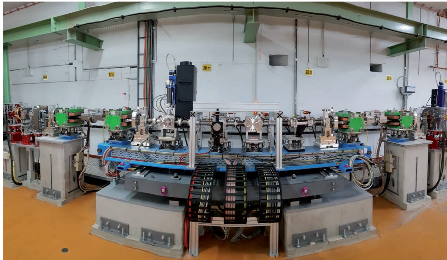
Figure 1 Fish-eye view of the movable magnetic bunch compressor with four dipole magnets (green) and beam instrumentation, beam position monitor, collimators and screen station (from right to left)
