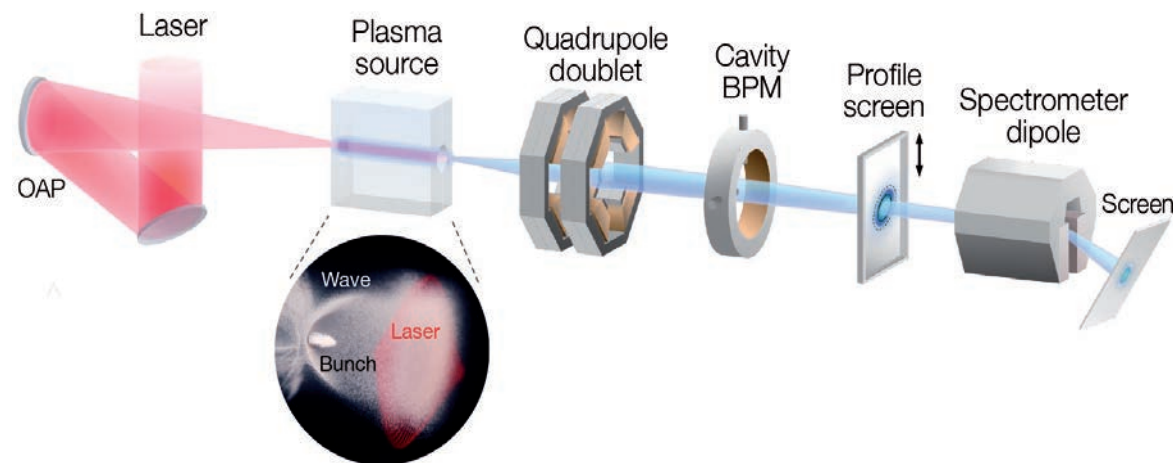
Figure 1 Schematic of the LUX accelerator: The 100 TW ANGUS laser is focused into a plasma source where it ionises hydrogen gas and drives a plasma wave (circular inset). An electron bunch is injected into the wave in a first nitrogen-doped section of the plasma source and then accelerated to hundreds of MeV in pure hydrogen over the following few millimetres. To analyse the beam parameters, the accelerated electron bunch is captured by quadrupole magnets and transported to several diagnostic devices. Figure adapted from [1] and Science Communication Lab.
