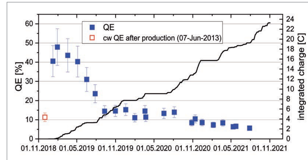
Figure 2 Quantum efficiency (QE) of the photocathode #105.2 presently in operation at FLASH. The red square indicates the QE measured in the lab after production. The blue squares are the QE measurements performed in the electron RF gun. As of November 2021, a charge of 23 C has been emitted (black line).
