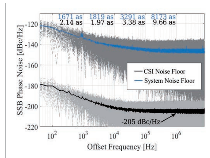
Figure 3 Phase noise limits for a standard receiver (blue curve) with sub-10 fs time resolution and for the carrier suppression interferometer prototype (black curve) with a time resolution of 10.76 as. The numbers above the graph correspond to the integrated jitter values per frequency decade.
