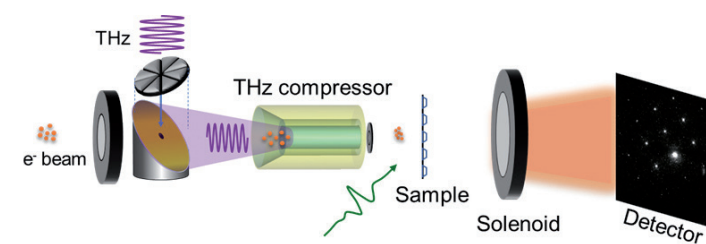
Schematic setup of the terahertz ultrafast electron diffractometer
