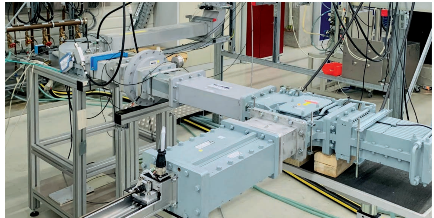
Figure 2 Isolator on the HPRF test stand
