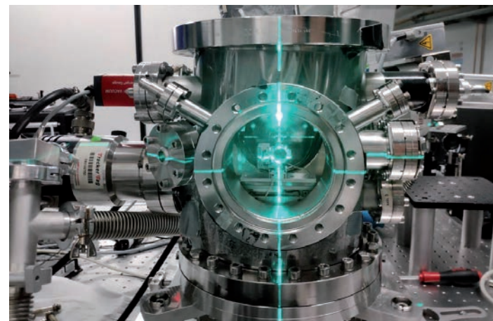
The terahertz ultrafast electron diffractometer fits on a lab table. It is adjusted with the help of an optical laser (green).
