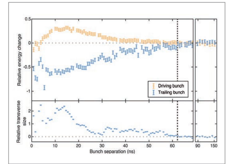
Figure 3 Residuals between energy spectra and transverse bunch size of both unperturbed and perturbed probe bunches. The vertical dashed line indicates the point of recovery of the plasma.
