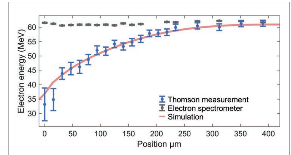
Figure 2 First in situ measurements of the electron energy evolution inside an LPA. The results are in good agreement with simulations of the process.
