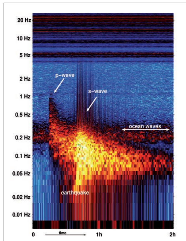
Figure 1 Spectrogram of an earthquake detected with the optical fibres. It originated in China on 21 May 2021 and had a magnitude of 7.3. The band at approx. 0.2 Hz stems from ocean waves.
