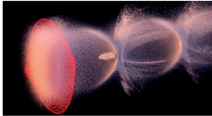
In laser plasma acceleration, an intense laser pulse (red) travelling through an ionised gas drives a bubble-shaped plasma wave consisting of electrons (light pink). An electron bunch (centre) riding this wave like a surfer is accelerated to high energies over extremely short distances. The rendering is based on real simulation data from the LUX experiment.
