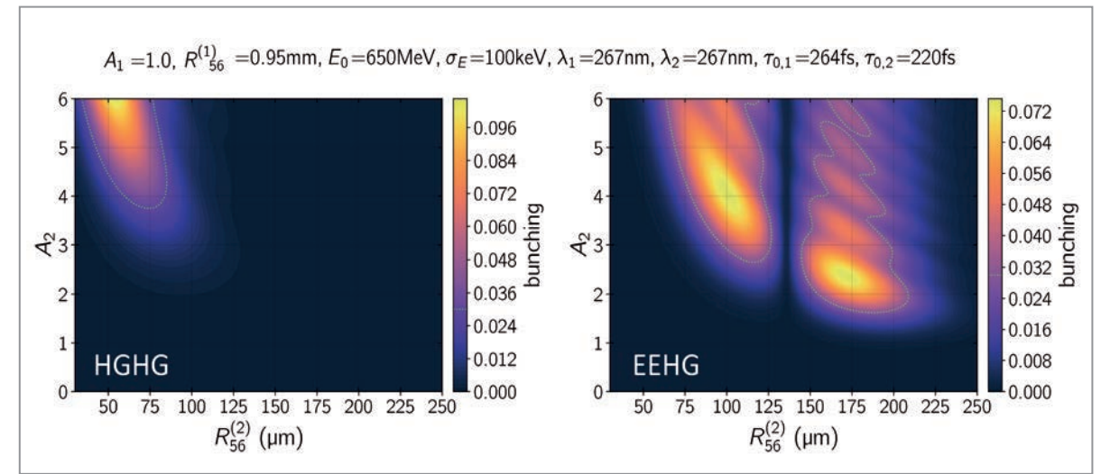
Figure 2 HGHG and EEHG bunching maps from analytical calculations [2] at the seventh harmonic for Xseed, which will be relied on for the next beamtimes in 2022/23
