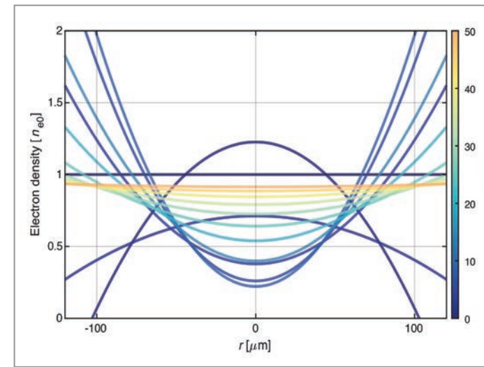
Figure 2 Experimentally derived radial plasma density profile as it evolves in time after the leading bunch has driven a wake.
