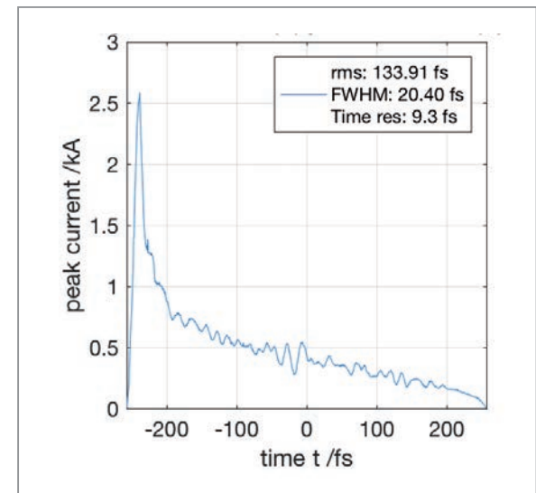
Figure 2 Current density of the electron bunch measured using the PolariX TDS. The measurement was performed during lasing with 3 \mu J at 5.9 nm and 26 \mu J at 17.7 nm using the mixed undulator configuration shown in Fig. 1 (bottom).
