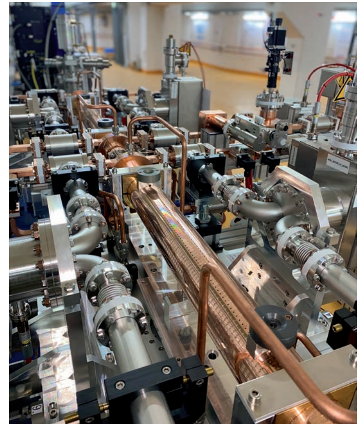
Figure 2 Detail of the X-band TDS system, showing the two copper deflecting structures. The waveguide system is visible on the top right.
