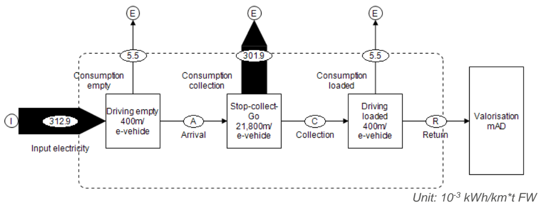
Figure 20: Energy balance of scenario 3
