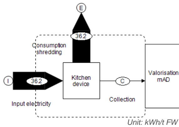
Figure 35: Energy balance of scenario 8
