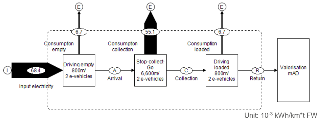
Figure 32: Energy balance scenario 7
