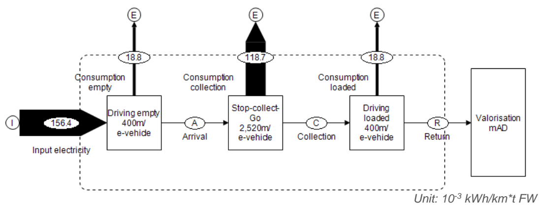
Figure 26: Energy balance of scenario 5
