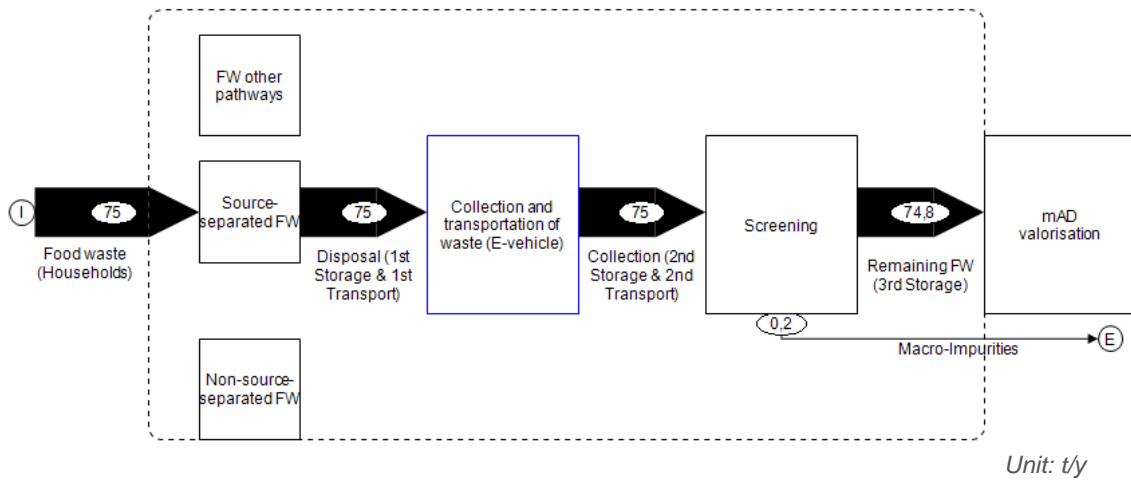
Figure 19: Mass balance of scenario 3
