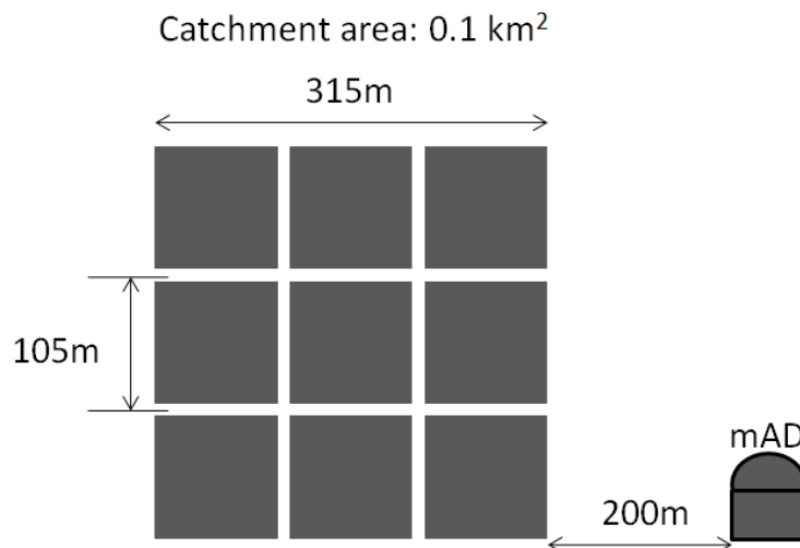
Figure 11: Example for the theoretical setting of the very small catchment area and a high population density in order to calculate the collection distances
