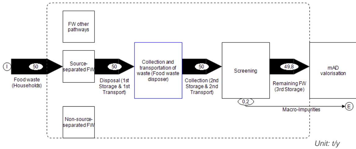
Figure 34: Mass balance of scenario 8
