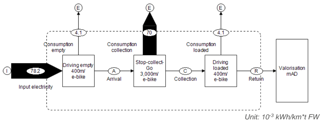
Figure 14: Energy balance of scenario 1
