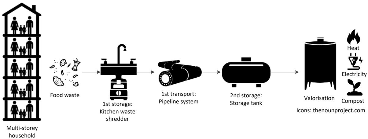
Figure 33: Scheme of collection scenario 8
