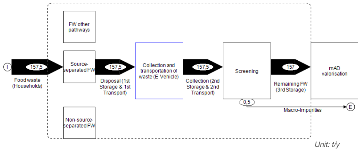
Figure 16: Mass balance of scenario 2
