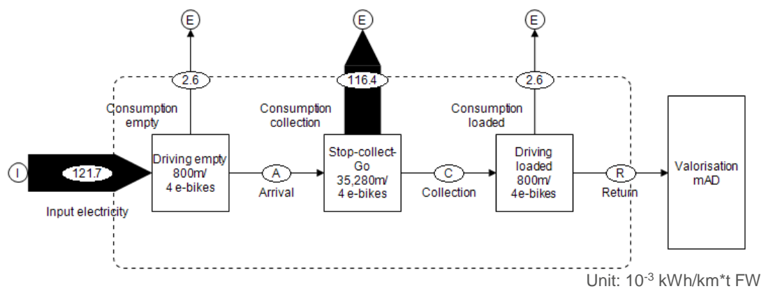
Figure 29: Energy balance of scenario 6
