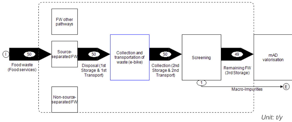
Figure 13: Mass balance of scenario 1
