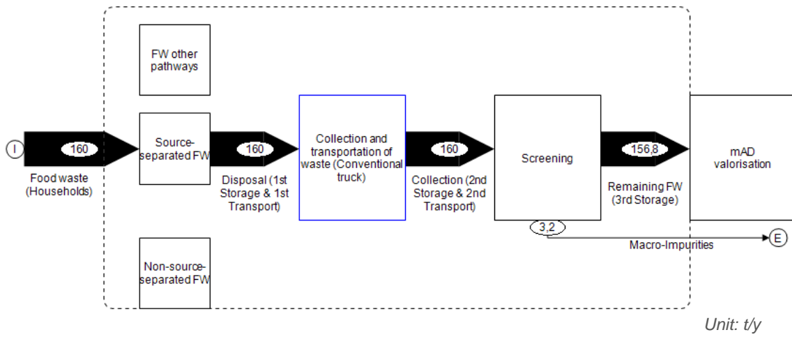
Figure 22: Mass balance of scenario 4
