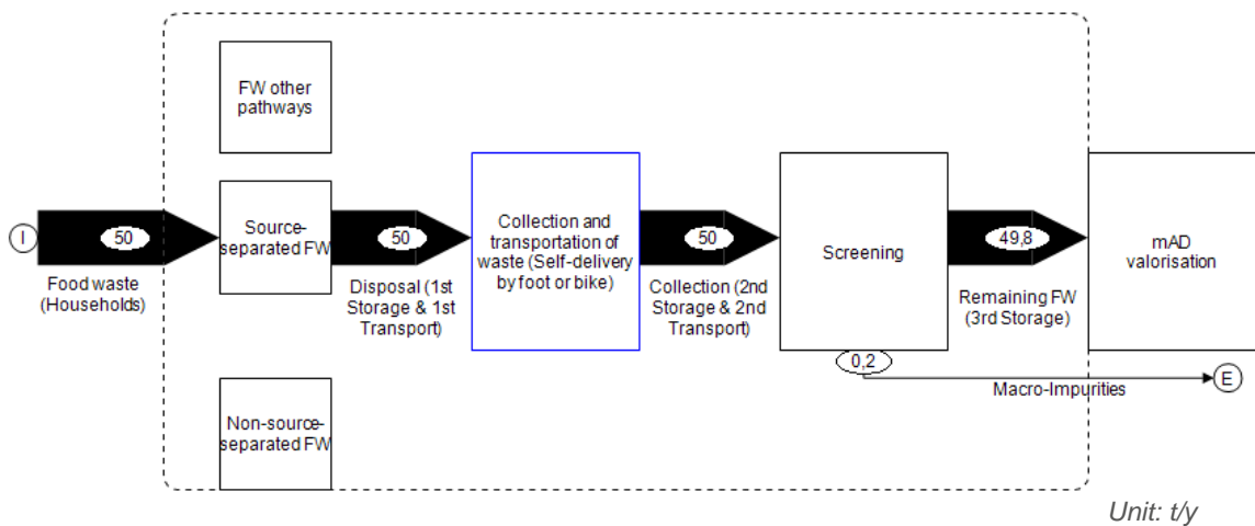
Figure 25: Mass balance of scenario 5
