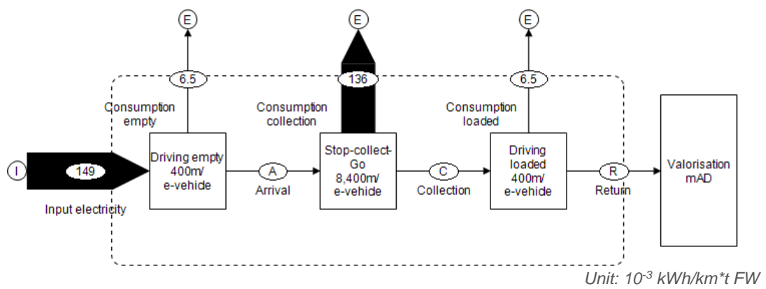
Figure 17: Energy balance of scenario 2
