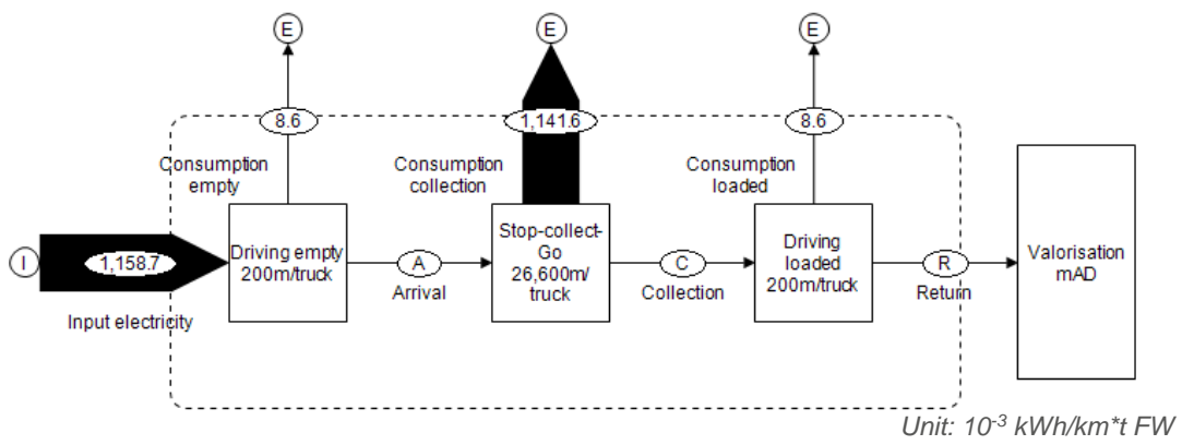
Figure 23: Energy balance of scenario 4
