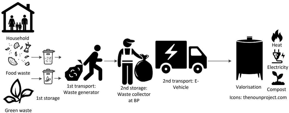
Figure 15: Scheme of collection scenario 2
