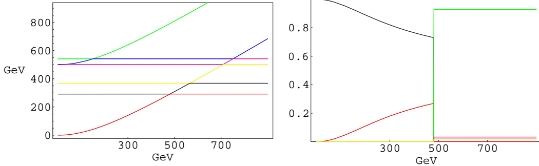
Figure 1: Plot of the neutralino mass spectrum as a function of M (left), for values \tan(\beta) = 3 , \mu = 500 , m_2 = 400 , m_1 = 300 , m_S = 500 , \delta = 0.029 and of the (squared) components of the LSP also as a function of M (right).
