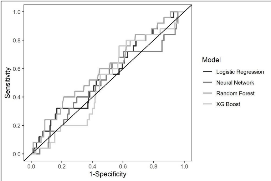
Figure 2 Receiver Operating Characteristics Curves
