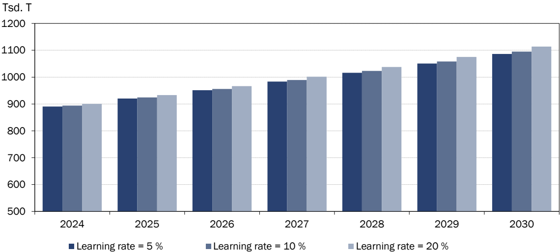
Figure 8: Global production capacities - impact of learning rates
