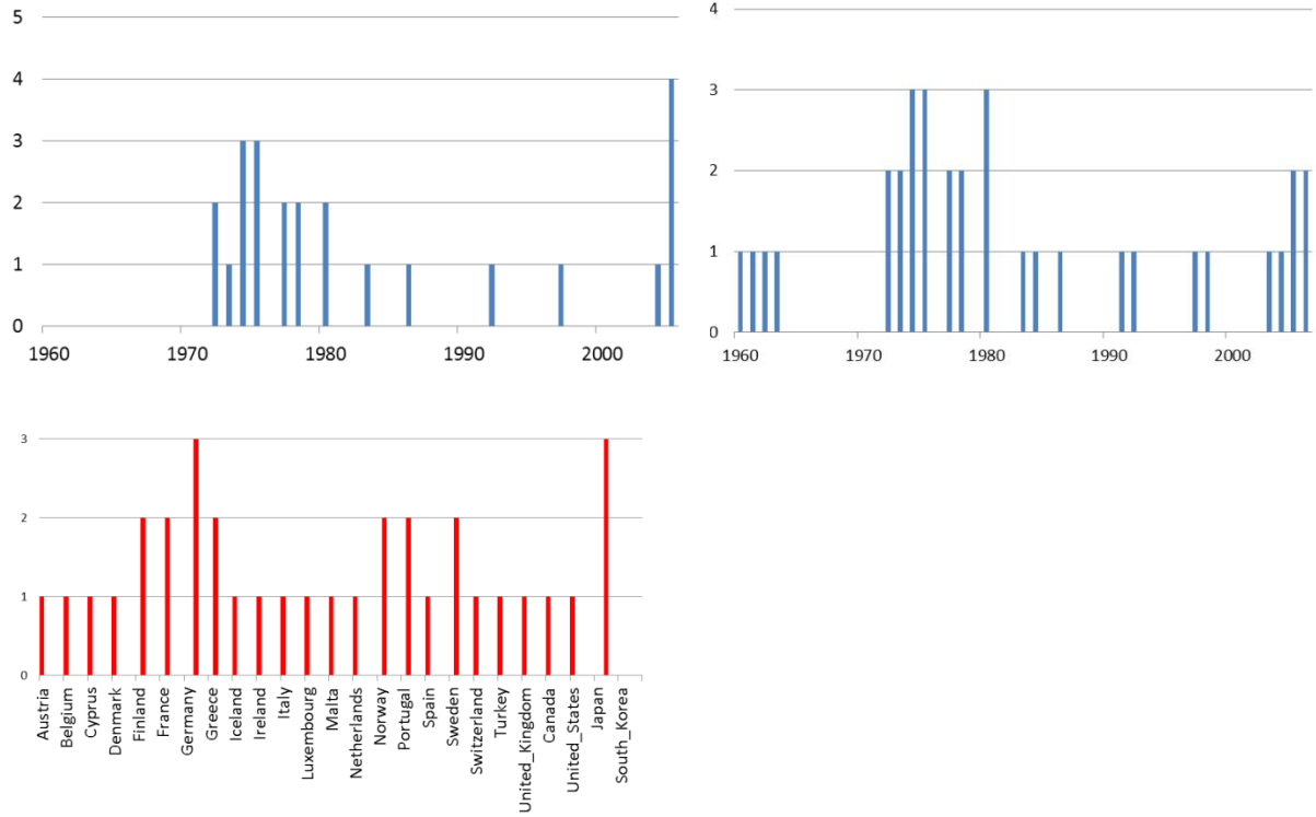
Left: results of Andrews-Quandt test on one unknown structural break, right: results of Bai-Perron test on multiple structural breaks. x-axis: time, y-axis: number of break points Results of Bai-Perron test on multiple structural breaks for all countries in the sample. x-axis: countries tested, y-axis: number of break points for every country
