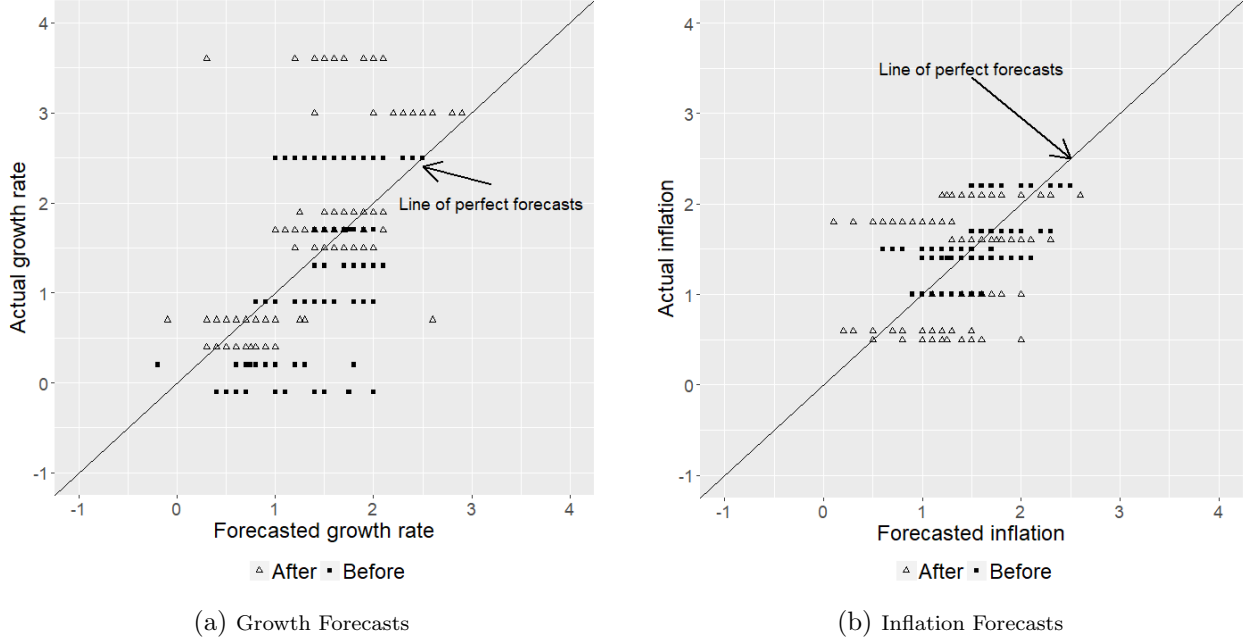
Figure 4: Correlation of Forecasts and Actuals
