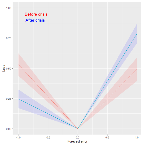
(c) Lin-Lin Loss Function, Inflation Forecasts
