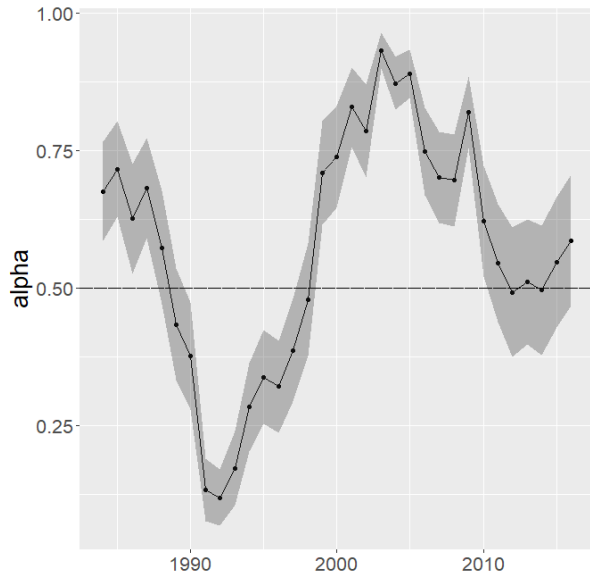
(a) Estimates Quad-Quad, Growth
