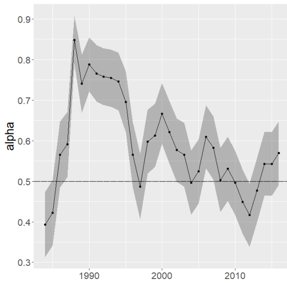
(c) Estimates Lin-Lin, Inflation
