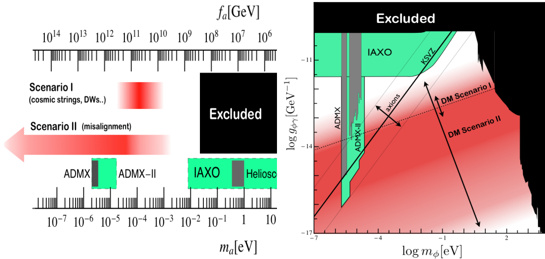
Figure 1: Parameter space for axions (left), ALPs (right) where they can account for the cold DM of the Universe together with excluded regions and the forecasts of ADMX and IAXO [20].
