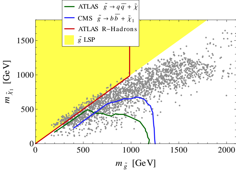
Figure 4: Parameter points with successful gauge coupling unification (gray). Also shown are the constraints on the gluino mass for the decay modes \tilde{g} \rightarrow q\bar{q} + \tilde{\chi}_1 and \tilde{g} \rightarrow b\bar{b} + \tilde{\chi}_1 by ATLAS and CMS (see text). The yellow region features a gluino LSP which is constrained by the ATLAS search for stable R-hadrons.
