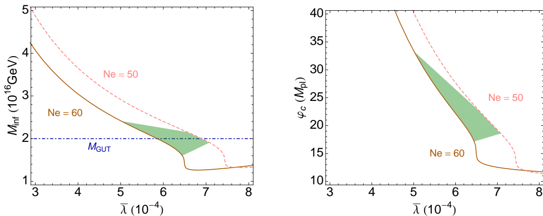
FIG. 2: Lines in the \bar{\lambda} - M_{\text{inf}} plane (left) and the \bar{\lambda} - \varphi_c plane (right), which are determined by the measured amplitude of the scalar power spectrum for N_e = 60 and 50. The shaded regions are allowed by the bound on n_s and r obtained from the Planck data. M_{\text{GUT}} = 2 \times 10^{16} GeV.
