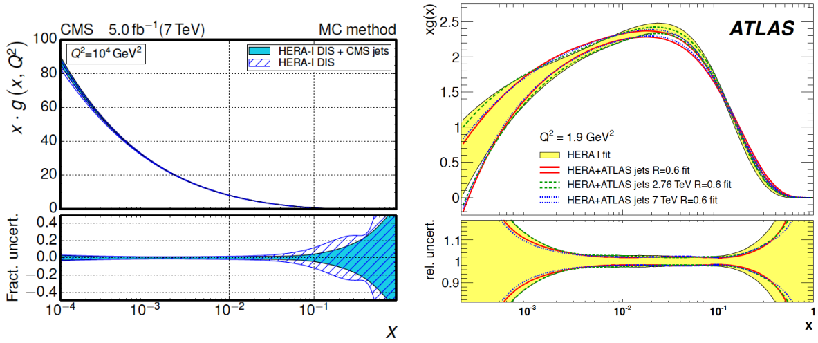
Fig. 4: Left plot: impact of the CMS 2011 inclusive jet data on the gluon PDF, from Ref. [48]. Right plot: impact of the ATLAS measurement on the ratio of inclusive jet cross-sections between 7 TeV and 2.76 TeV on the gluon PDF, from Ref. [24].
