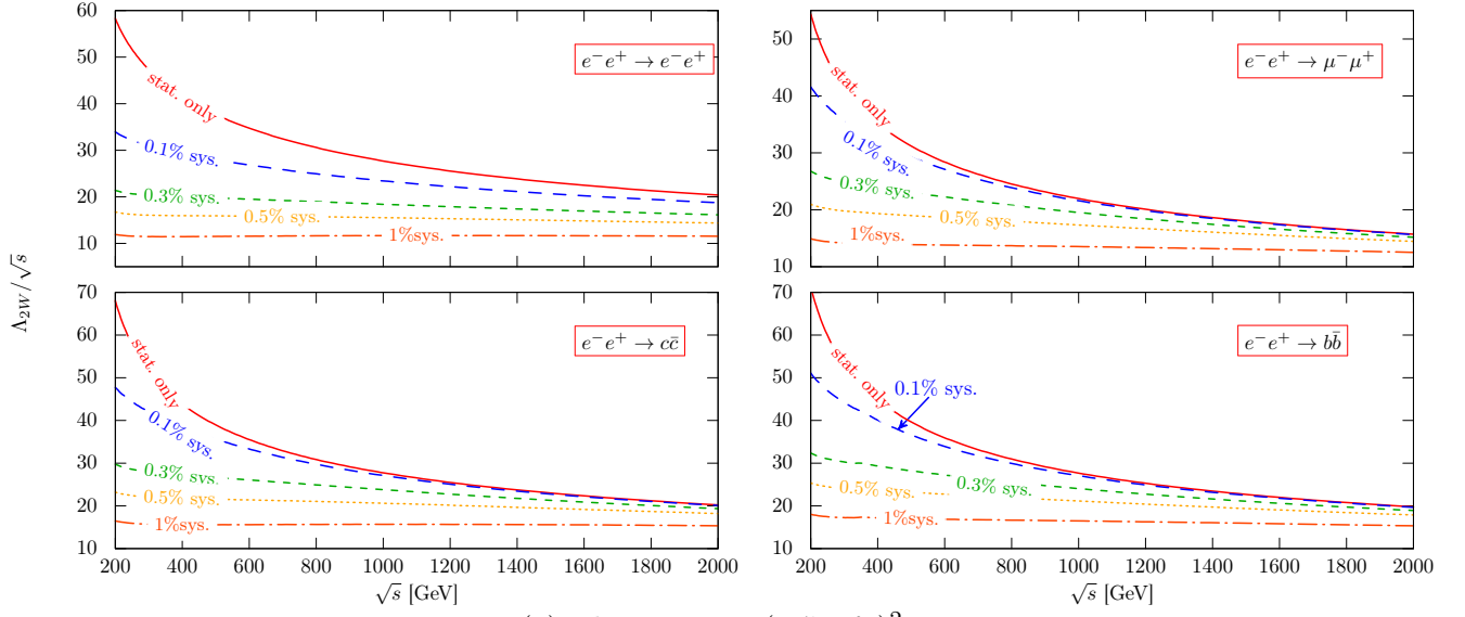
(a) The operator (D^\mu W_{\mu\nu}^a)^2
