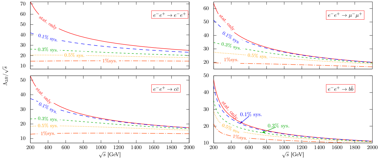
(b) The operator (\partial^\mu B_{\mu\nu})^2
