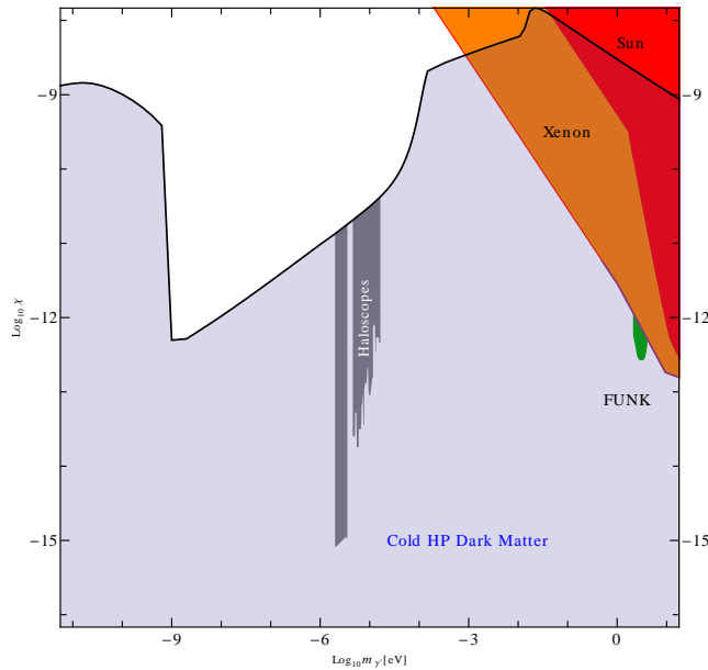
Figure 2. Parameter space of hidden photon dark matter in the sub-eV range. The blue shaded region is the viable HP DM parameter space as discussed in [15]. Other regions see text.
