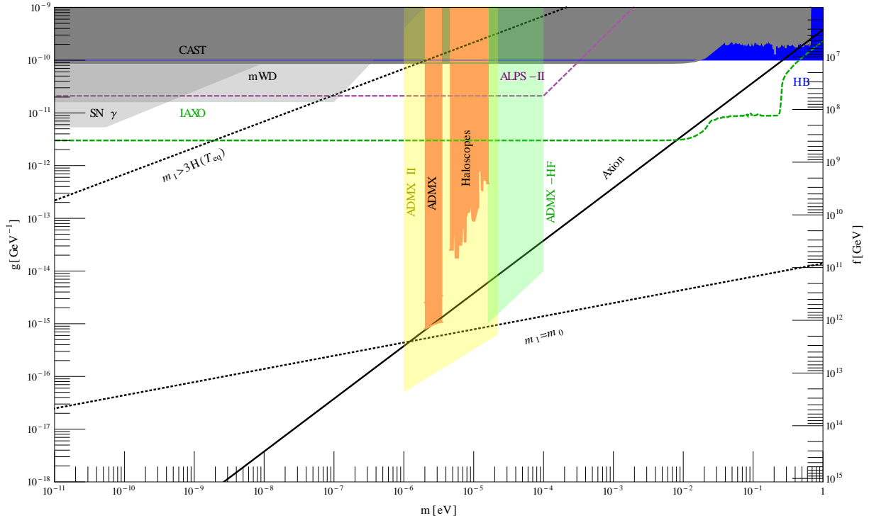
Figure 1. Parameter space of axion and axion-like particle DM (photon-coupling) in the sub-eV range. See text for details.
