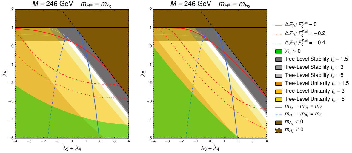
Figure 8. \lambda_3 + \lambda_4 vs \lambda_5 for M = 246 \text{ GeV} and assuming respectively m_{H^\pm} = m_{A_0} (Left) and m_{H^\pm} = m_{H_0} (Right). Red lines show constant values of \Delta \mathcal{F}_0 / \mathcal{F}_0^{\text{SM}} , with the green region corresponding to \Delta \mathcal{F}_0 / \mathcal{F}_0^{\text{SM}} < -1 ( \mathcal{F}_0 > 0 ). Blue lines show the contours m_{A_0} - m_{H_0} > m_Z (solid) and m_{H_0} - m_{A_0} > m_Z (dashed). The grey and orange regions are respectively excluded by boundedness from below of the scalar potential and by unitarity, for t_\beta = 1.5, 3, 5 (dark to light). The brown region is unphysical ( m_{H_0} < 0 and/or m_{A_0} < 0 ).
