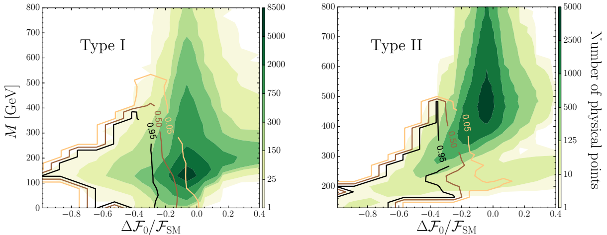
Figure 3. Distribution of physical points, as in Figure 1, and \mathcal{P}_{\xi > 1} contours in the (\Delta\mathcal{F}_0/\mathcal{F}_{SM}^{\text{SM}}, M) plane.
