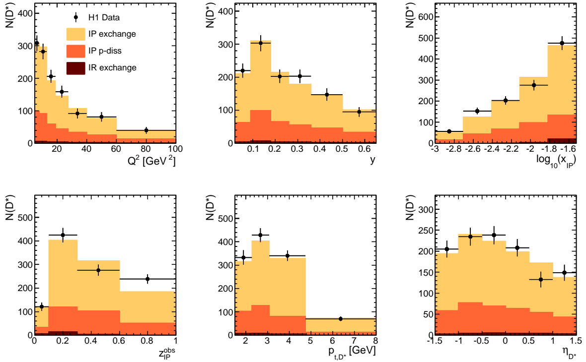
Figure 3: The differential N(D^*) distributions obtained from \Delta m fits to the data and simulation as a function of Q^2 , y , \log_{10}(x_P) , z_P^{obs} , p_{t,D^*} and \eta_{D^*} . The data are represented with dots. The contributions of individual processes in the simulation, reweighted RAPGAP, are indicated by filled histograms as follows; elastic proton pomeron exchange (light orange), proton dissociation (dark orange) and reggeon exchange (dark red).
