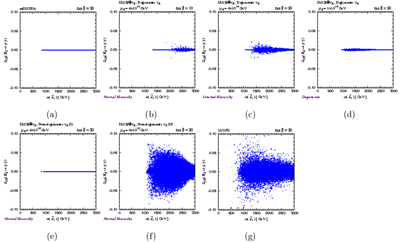
FIG. 9: The mixing-induced CP asymmetry in B_d \rightarrow \rho\gamma as functions of m(\tilde{d}_1) for the same parameter sets as those for Fig. 6.
