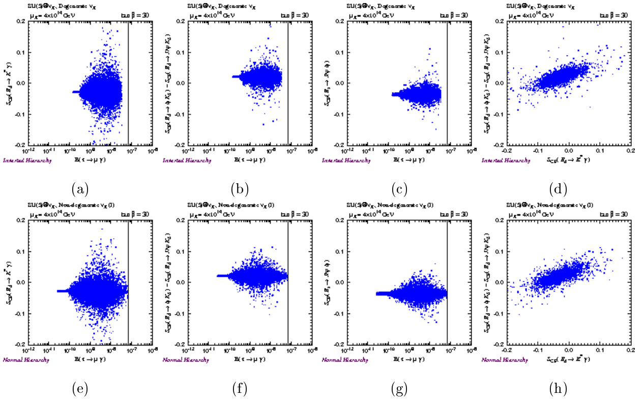
FIG. 13: Correlations among b \rightarrow s observables and B(\tau \rightarrow \mu\gamma) .
