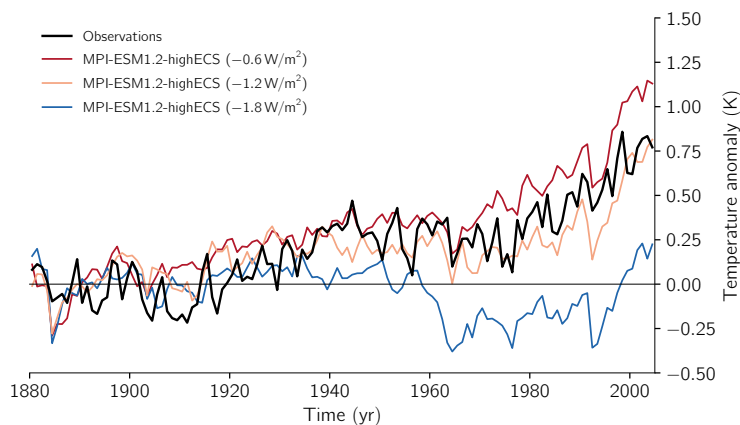
Figure 3.3: Comparison of the MPI-ESM1.2-highECS model to observations. The curves show the instrumental temperature record and model runs with different aerosol-cooling strengths. The model was run four times with each aerosol setting, and the ensemble mean is displayed.
