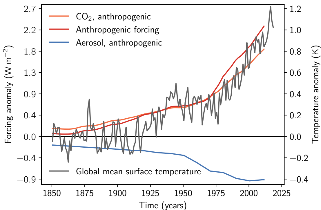
Figure 1.1: Temperature change and human intervention in the radiative forcing. Global mean surface temperature anomaly from the dataset (version 2) provided by Cowtan and Way (2014). The reference period for the temperature anomalies is 1850-1900. The forcing time series are those collected by the IPCC (IPCC 2013a). Note that the striking temperature increase since the 1970s coincides with the increase of the total anthropogenic forcing after the reduction in the anthropogenic aerosol forcing.
