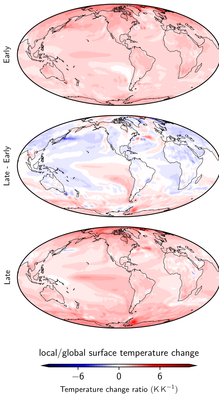
Figure 4.5: SST pattern in the MPI-ESM1.2 model for an abrupt4xC02 experiment with cloud-locking. The slope of the regression of local surface temperature change on global mean surface temperature change. Top panel: Early period (years 1-20). Bottom panel: Late period (years 21-150). Middle panel: Late-Early. Same colour scale as in figure 4.3. Note the stronger southern polar amplification during the late period in comparison to the free-cloud case.
