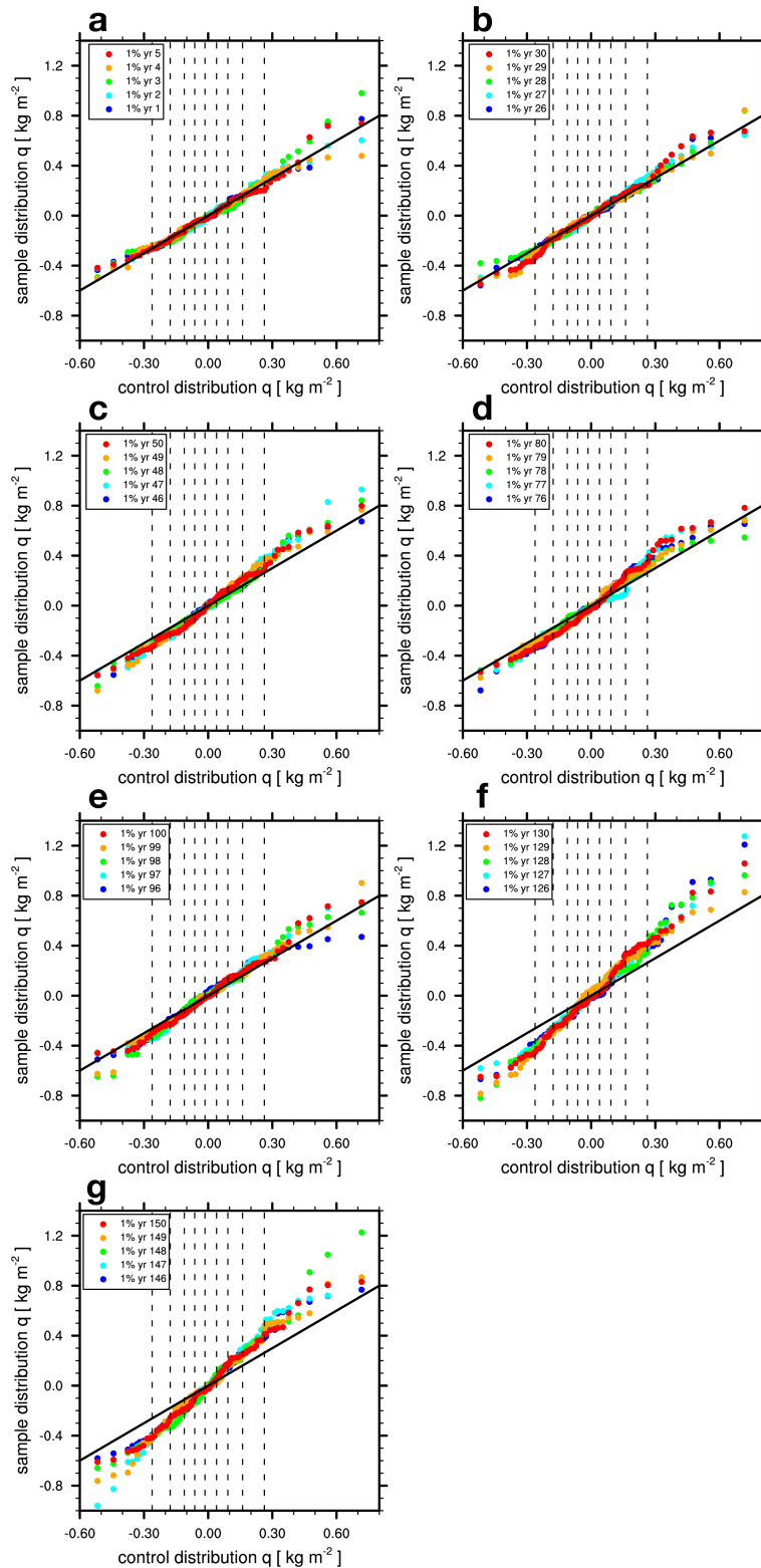
Figure 1.9: Robust changes in the extreme events appear after 30 years, a broadening of the whole distribution occurs more gradually. QQ plots similar to figure 1.6 for different 5-year windows over the whole length of the simulation. The vertical dashed lines indicate deciles of the control distribution. a: years 1-5, b: 26-30, c: 46-50, d: 76-80, e: 96-100, f:126-130, g: 146-150.
