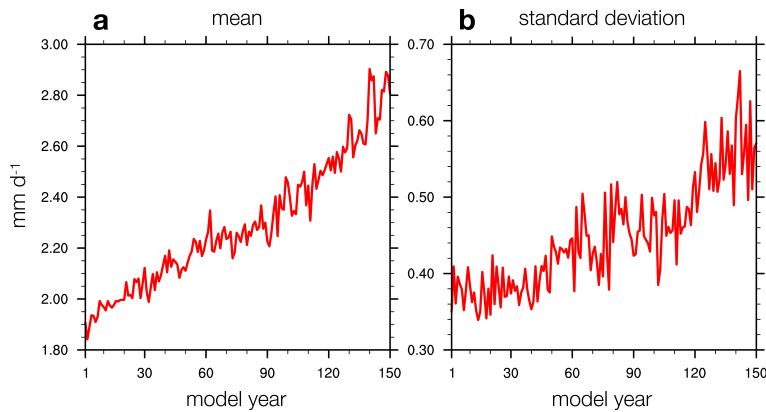
Figure 2.6: Increase in mean rainfall and rainfall variability over the Sahel in response to global warming. Time series of (a) ensemble mean and (b) ensemble standard deviation for JJASO Sahel rainfall in the 1% CO 2 experiment.
