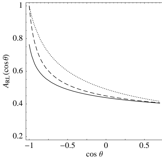
(c) m_X = 30 GeV.
