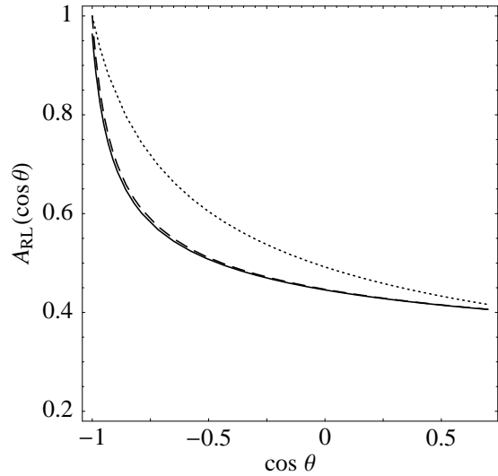
(b) m_X = 10 GeV.
