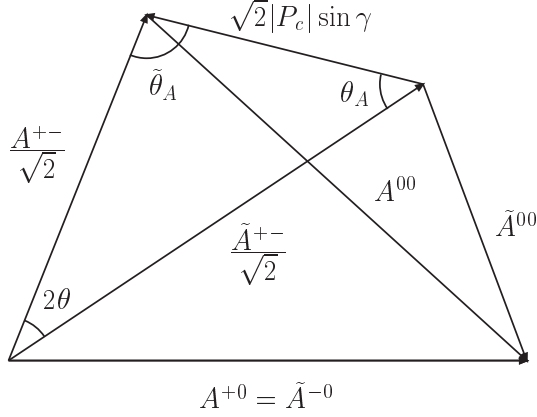
Figure 2. The isospin triangle for the B \rightarrow \pi\pi decay amplitudes A^{ij} and the same for the phase-shifted charge-conjugate ones \tilde{A}^{ij} = e^{2i\gamma} A^{ij} in the complex plane.
