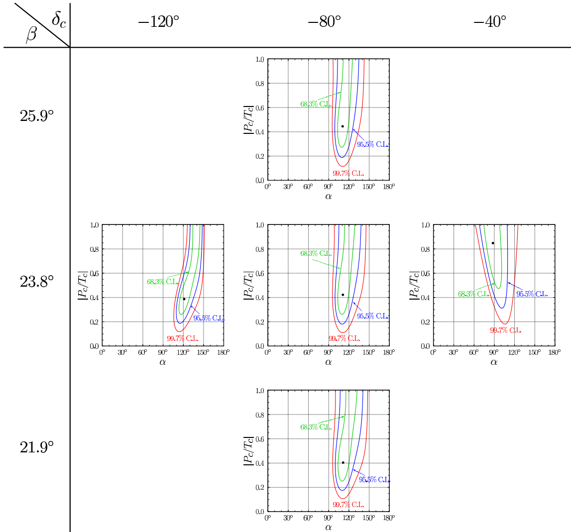
Figure 8. The correlation |P_c/T_c| - \alpha corresponding to the 68.3%, 95.5%, and 99.7% C.L. ranges of C_{\pi\pi}^{+-} and S_{\pi\pi}^{+-} for \delta_c = -120^\circ, -80^\circ, \text{ and } -40^\circ .
