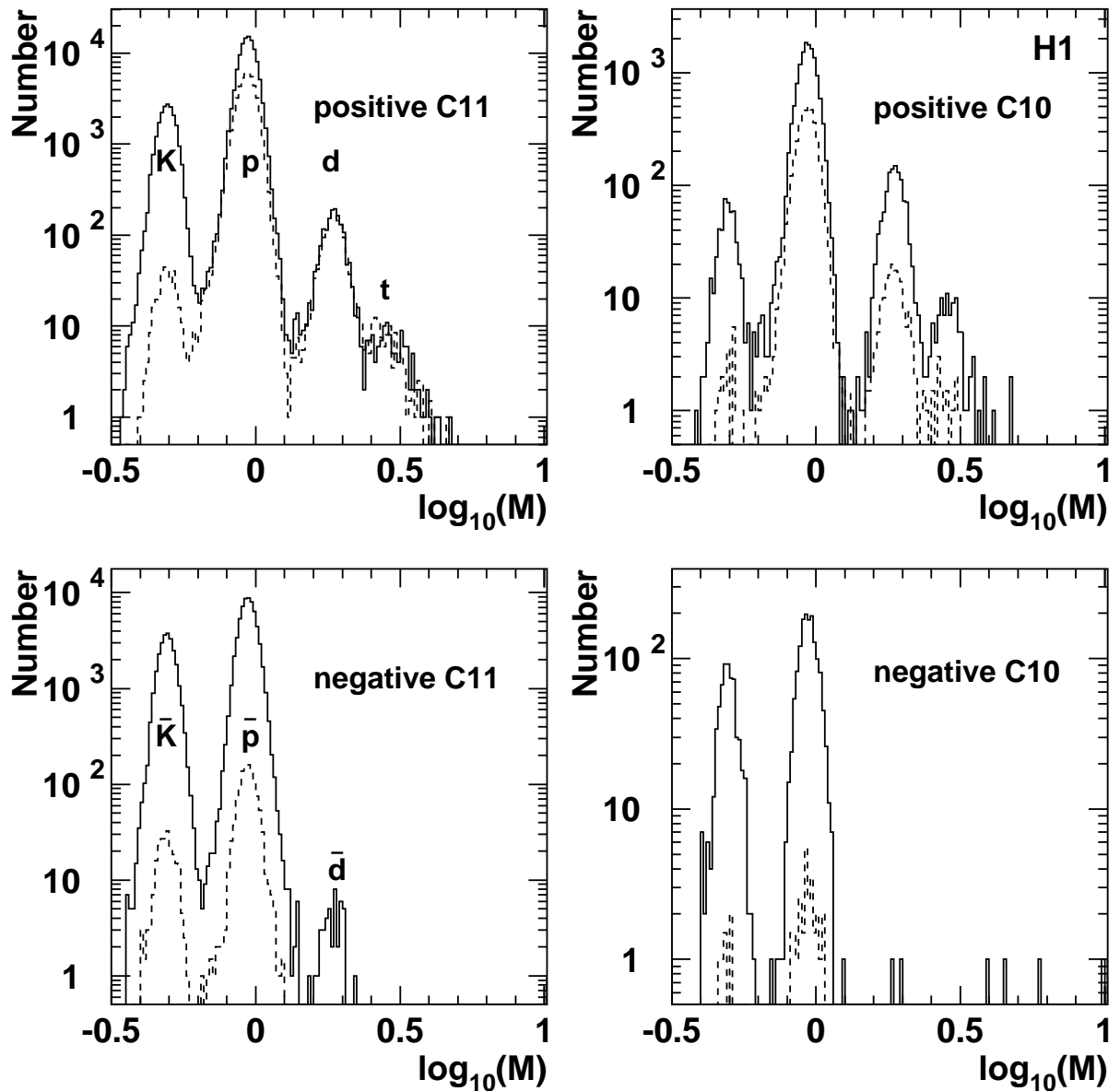
Figure 4: The mass spectra (with M in GeV) for positive and negative particles in the hard selected sample for the mainly photoproduction ( C_{11} ) and mainly pG ( C_{10} ) samples. The dashed lines show the material background deduced from the sideband subtraction method.
