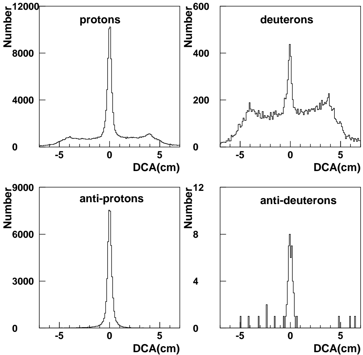
Figure 2: The distribution of the distance of closest approach (DCA) of the track to the event vertex in the plane transverse to the beam direction for p , d , \bar{p} and \bar{d} candidates with momenta larger than 0.5 GeV from the hard selection and before any track timing cuts. The peak at zero from beam induced events sits on the material background which is much smaller for \bar{p} , \bar{d} than for p , d .
