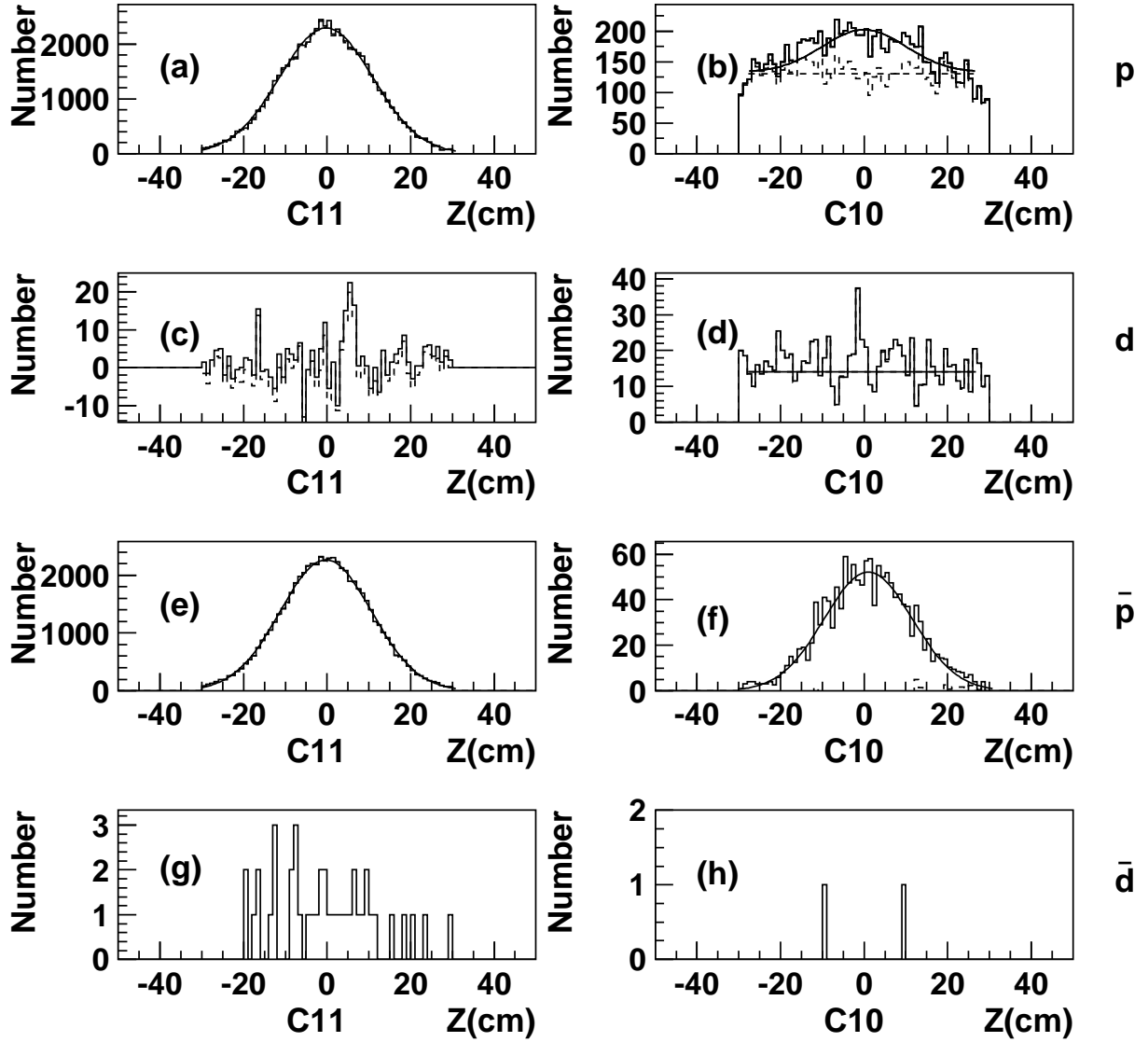
Figure 3: The z vertex distributions for identified protons (a,b), deuterons (c,d), anti-protons (e,f) and anti-deuterons (g,h) in the hard selected samples after correction for the material backgrounds. The C_{11} samples (figures a,c,e,g) are dominated by photoproduction events and the C_{10} sample (figures b,d,f) are dominated by pG events. The solid curves (figures a,b,c,d) show the fits of a Gaussian distribution (expected from photoproduction) and a linear background (expected from pG interactions). The lack of background and the relatively small number of events in (f) show that there is little \bar{p} production in pG events. The number of \bar{d} events in (h) is compatible with that expected from the \gamma p contamination of C_{10} sample. The lack of background in (a) and (e) shows that there are few pG events in the C_{11} sample. The dashed histograms represent the background after subtraction of the fitted (b) or calculated (c,f) Gaussians.
