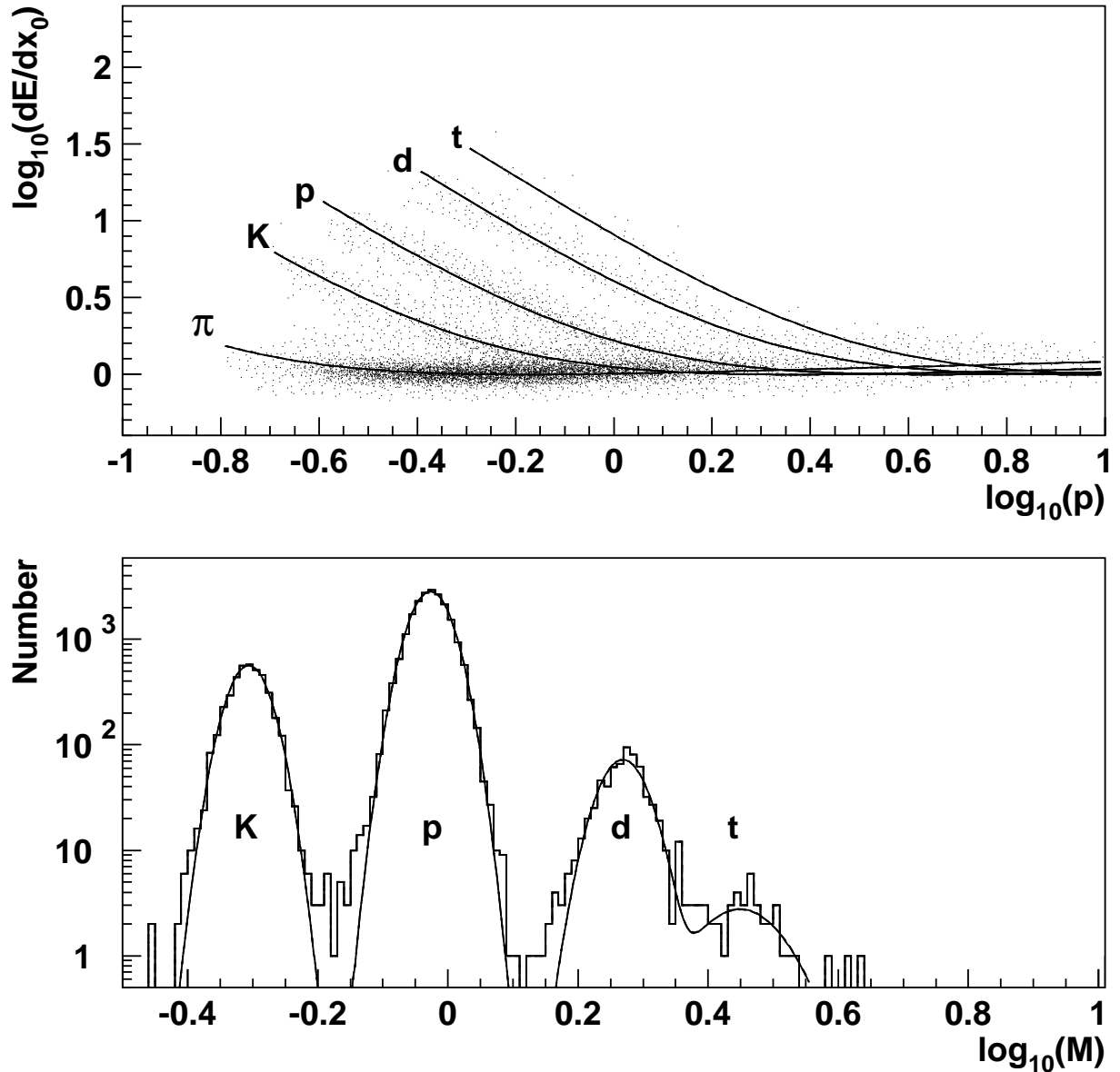
Figure 1: Upper plot - the observed specific ionisation energy loss, dE/dx , (normalised to that from a MIP), obtained from the log-likelihood method, versus track momentum (in GeV) for a sample of positively charged tracks from the hard selection (before application of the specific energy loss cut, see text). The smooth curves show the expected mean specific energy loss for the different particle species. Lower plot - the spectrum of masses (in GeV) for \log_{10} dE/dx > 0.4 , deduced as described in the text. The smooth curves represent Gaussian fits to each peak.
