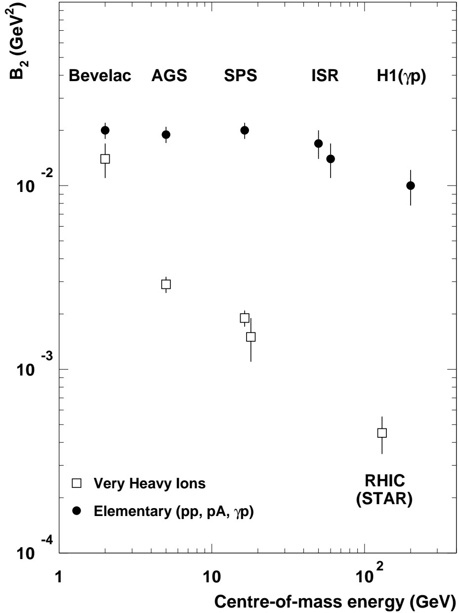
Figure 7: The dependence of B_2 on centre-of-mass energy for very heavy ion collisions (open squares) and interactions of more elementary particles (closed circles). The heavy ion data are the Ne-Au data at the Bevelac [21], the E886 Au-Pt data at the AGS [22], the Pb-Pb data of NA44 [23] and NA52 [24] at the SPS and the Au-Au data of STAR [7] at RHIC. The “elementary” data are the pA data of [21, 22, 25], the pp data at the ISR [5, 6] and the photoproduction data presented here. In the latter the error bar represents the total uncertainty i.e. the sum in quadrature of the systematic and statistical uncertainties.
