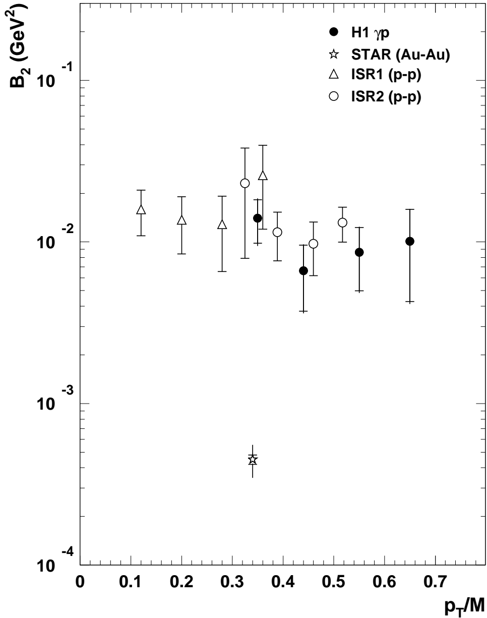
Figure 6: The p_T/M dependence of the parameter B_2 for \gamma p (this experiment), pp [5, 6] and Au-Au interactions [7]. The values of B_2 for the pp data are deduced from the measured cross sections [5, 6]. There is a theoretical uncertainty of about 20% (not shown) in the determination of B_2 for the photoproduction and pp data, which arises from the calculation of the fraction of anti-protons produced directly (see text). The inner error bars on the H1 data indicate the statistical and the outer the total uncertainties.
