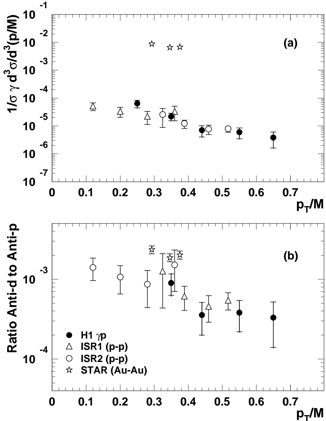
Figure 5: a) The measured invariant cross section (normalised to the relevant total cross section) for inclusive \bar{d} production, compared with the pp and Au-Au data. b) The measured \bar{d} to \bar{p} production ratio as a function of p_T/M (solid points) compared with pp data from the ISR at \sqrt{s} = 53 GeV in the central region [5, 6] and RHIC data on Au-Au collisions [7]. The inner error bars on the H1 data indicate the statistical and the outer the total uncertainties.
