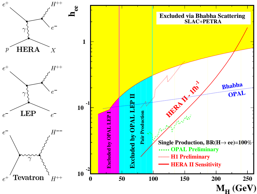
Figure 3.2: Mechanisms involving doubly charged higgs at colliders (left) and world status of the limits on the coupling to electrons h_{ee} versus Higgs mass. The previsions for next running period at HERA II is also indicated.
