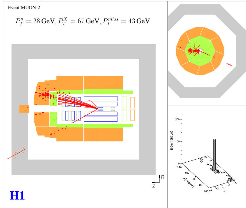
Figure 2.13: Display of an event with an isolated muon, missing transverse momentum and a prominent hadronic system. The acoplanarity between the lepton and the hadronic system is the signature of an undetected particle.
