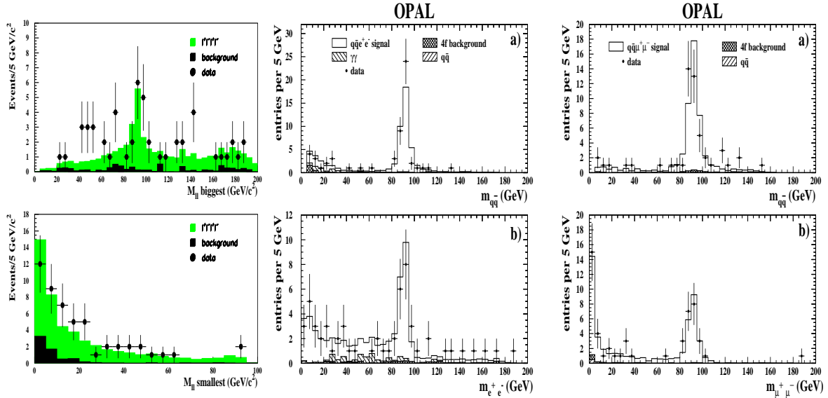
Figure 2.4: Maximum and minimum di-lepton invariant mass distribution for four lepton events detected with a flavour independent method by DELPHI(left). Invariant mass of same flavour fermion pairs in e^+e^-q\bar{q} (center) and \mu^+\mu^-q\bar{q} (right) channels(from OPAL analysis).
