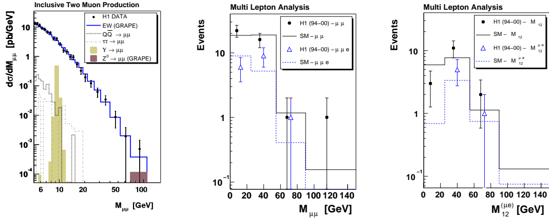
Figure 2.17: Muon pair production cross section as a function of the invariant di-muon mass (left). Distributions of the invariant mass M_{\mu\mu} for compared with the Standard Model predictions (right). Distribution of \mu\mu e events as function of mass M_{12} of the two highest P_t leptons, and of the mass M_{12}^{\mu e} for those events where the leptons with the highest P_t are a muon and the electron.
