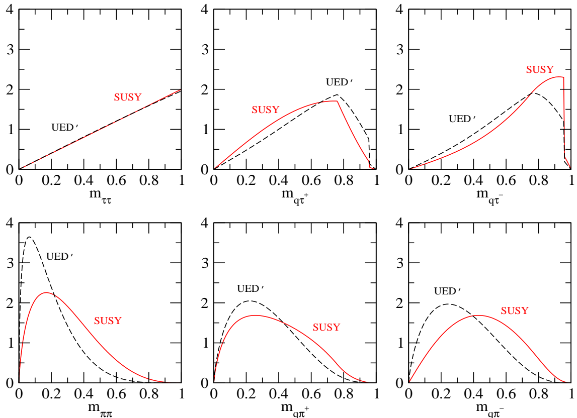
Figure 3: The “normalized” distributions in supersymmetry and UED’ for the particle spectrum corresponding to the SUSY scenario SPS1a; the distributions [\tau\tau] , [q\tau^+] and [q\tau^-] in the upper frames and the distributions [\pi\pi] , [q\pi^+] and [q\pi^-] in the lower frames.
