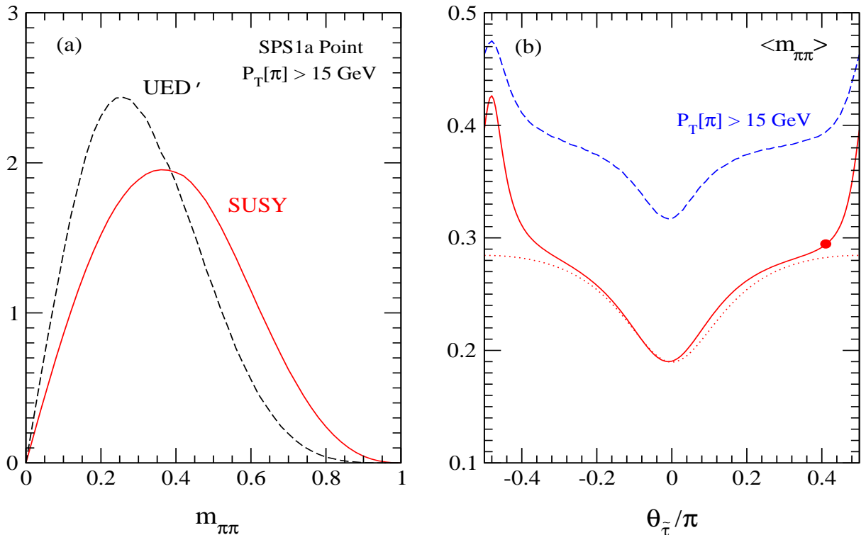
Figure 4: (a) The SUSY and UED' distributions of the \pi\pi invariant mass with a cut of 15 GeV on the pion transverse momenta; and (b) the dependence of the expectation value \langle m_{\pi\pi} \rangle on the stau mixing angle \theta_{\tilde{\tau}} [in units of \pi ] for the SPS1a values of \tan\beta, M_{1,2}, \mu and the lighter stau mass m_{\tilde{\tau}_1} [without (red) and with (blue) \pi transverse momentum cut]. The (red) dot on the solid line denotes the value of \langle m_{\pi\pi} \rangle at the SPS1a point. The (red) dotted line represents the average values of \langle m_{\pi\pi} \rangle if \tilde{\chi}_{1,2}^0 are unmixed pure bino-like and wino-like states, respectively.
