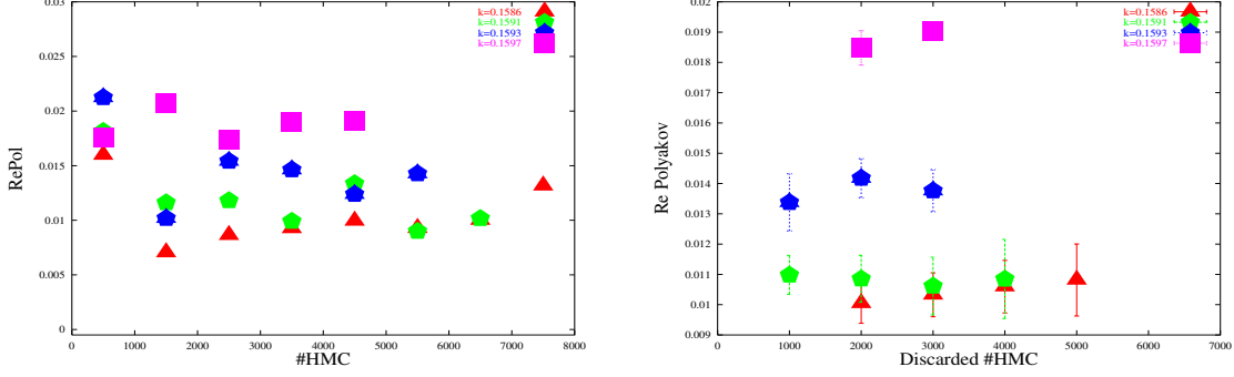
Figure 4: HMC evolution and error analysis for the high statistics runs at \beta = 3.9 : binned averages (left) as a function of the HMC trajectories, and results and errors as a function of the discarded HMC trajectories (right).
