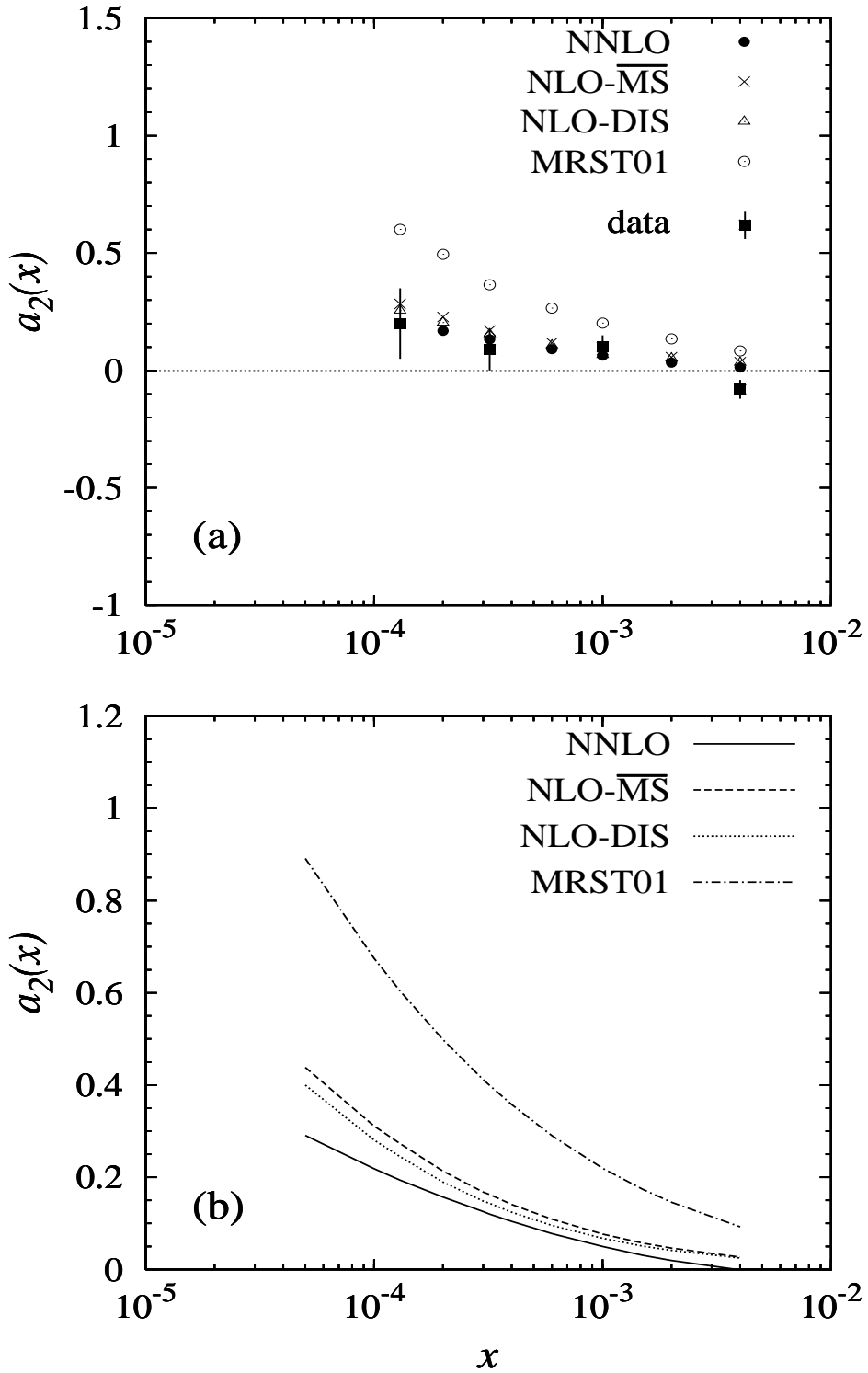
Figure 5: The curvature a_2(x) as defined in (15) for (a) the variable q -intervals in (16) and (b) the fixed q -interval in (17). Also shown are the corresponding MRST01 NLO results [20]. The data in (a) are taken from [1]. The NNLO prediction at the lowest x -value coincides with the data (full square).
