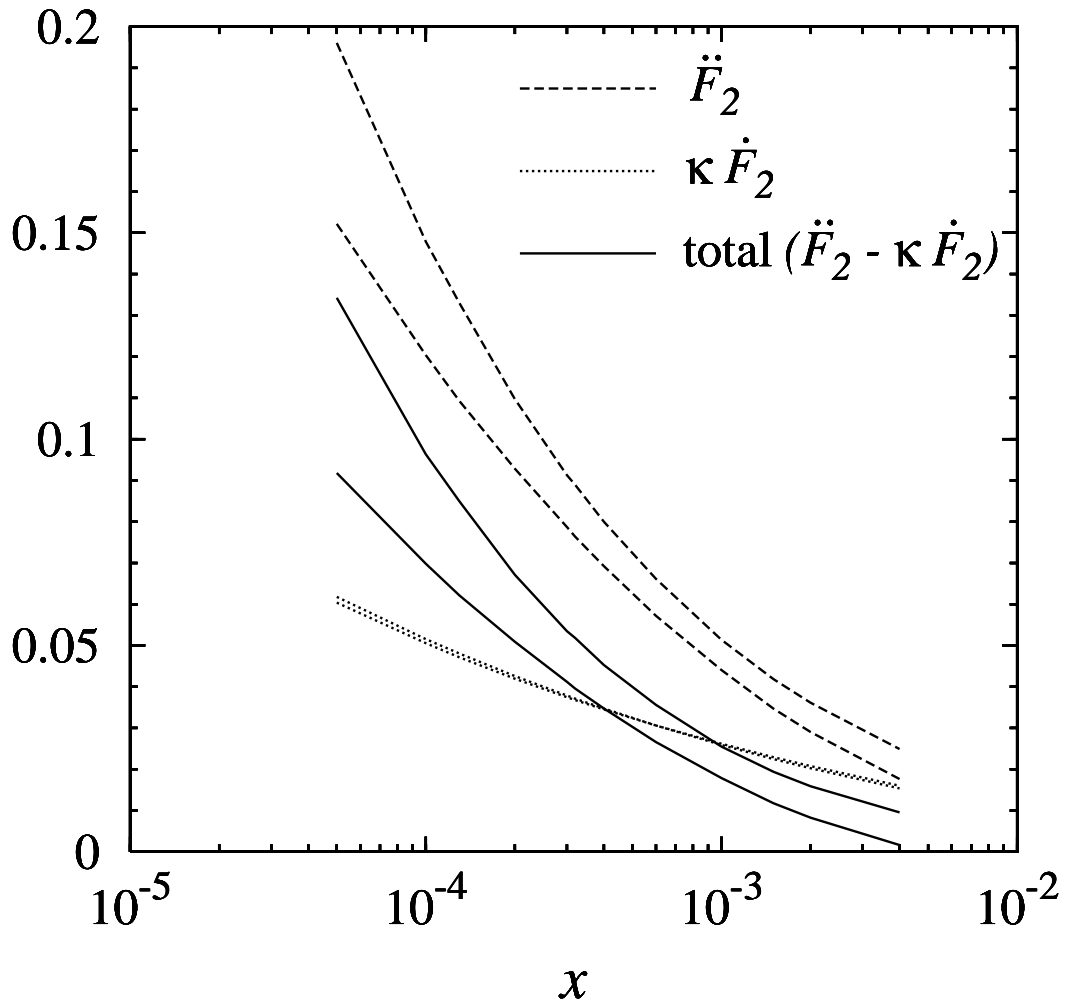
Figure 6: The predicted slope \dot{F}_2^p \equiv \partial F_2^p / \partial \ln Q^2 and curvature \ddot{F}_2^p appearing in (18) for the fixed q -interval in (17), with the suppression factor \kappa = 0.1 corresponding to an average Q^2 = 4.5 \text{ GeV}^2 ( q = 1 ). At smallest values of x , the individual upper curves always refer to NLO( \overline{\text{MS}} ) and the lower ones to NNLO( \overline{\text{MS}} ).
