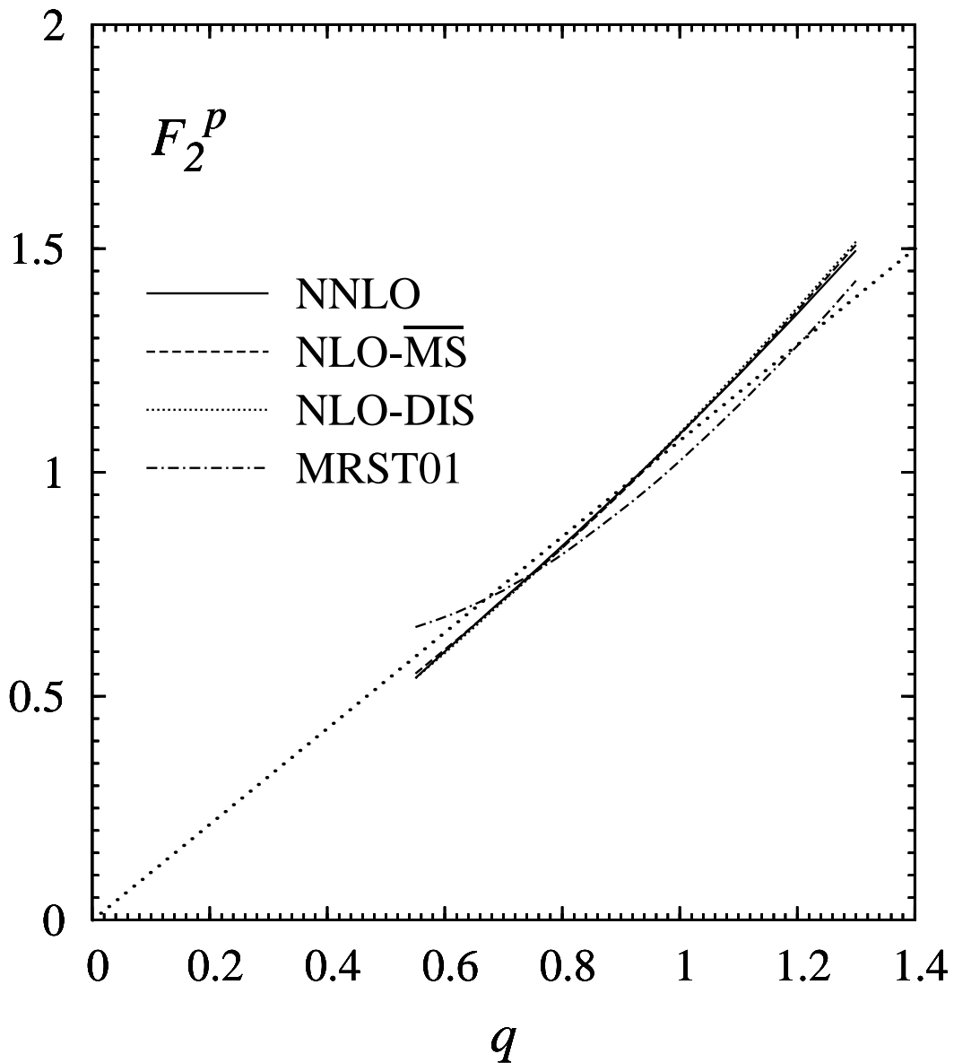
Figure 4: Predictions for F_2^p(x, Q^2) at x = 10^{-4} plotted versus q defined in (14). For comparison the global fit NLO result of MRST01 [20] is shown as well. The global CTEQ6M NLO fit [21] is very similar to our NLO and NNLO results as can be deduced from [2], and the same holds true for the H1 fit [15]. Most small- x data lie along the straight dotted line [1].
