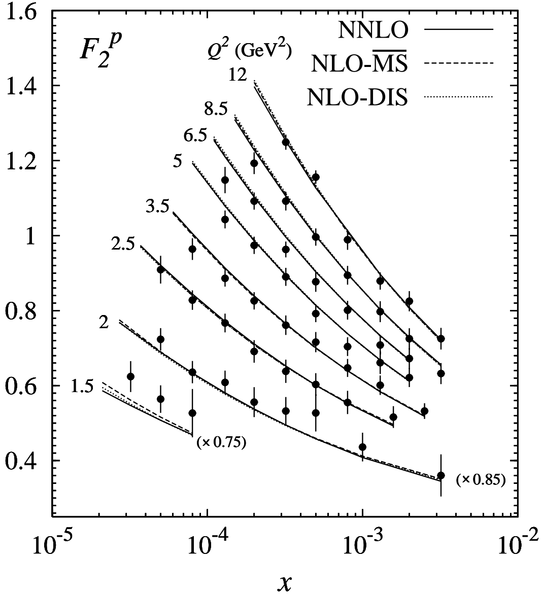
Figure 1: Comparison of our various perturbative fits with the H1 data [14] at very small- x . Our 3-loop NNLO results always refer to the \overline{\text{MS}} factorization scheme. To ease the graphical representation, the results and data for the lowest two bins in Q^2 have been multiplied by the numbers as indicated.
