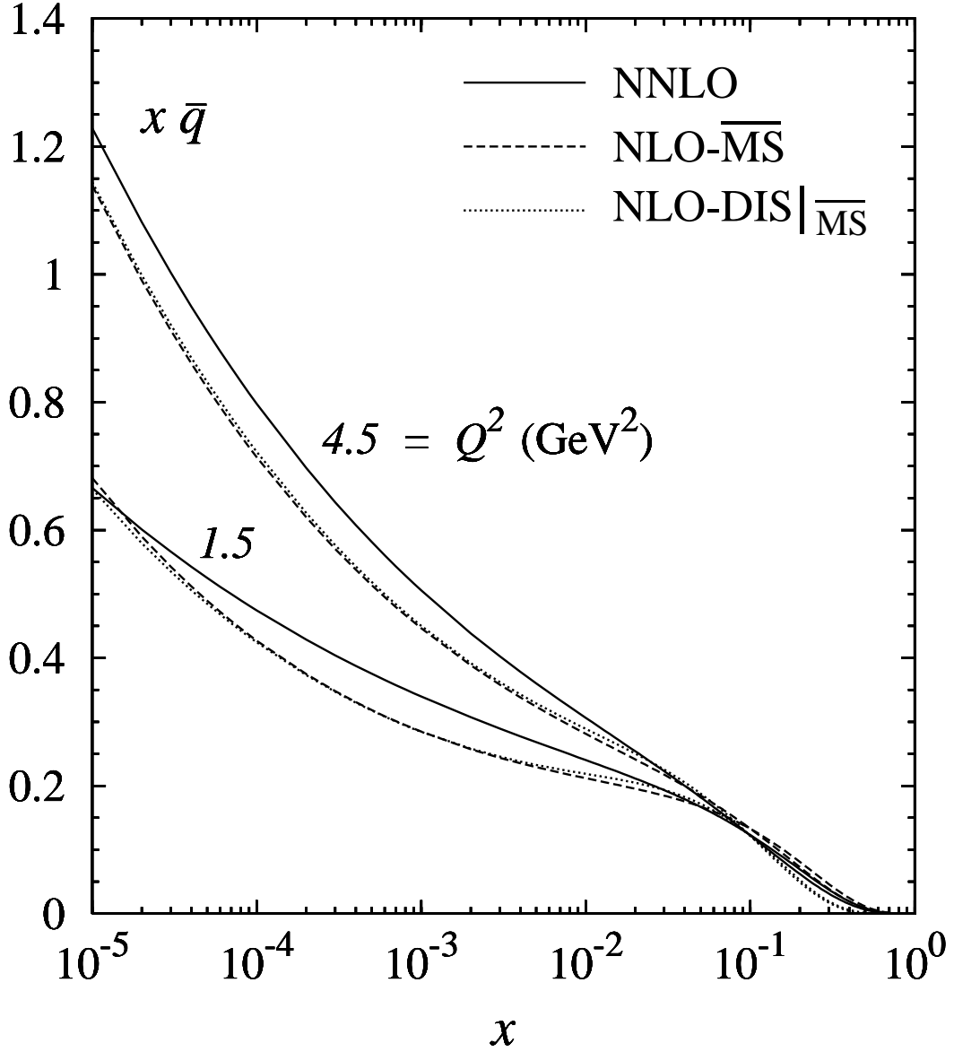
Figure 3: As in Fig. 2 but for the sea distribution x\bar{q}(x, Q^2) where \bar{q} \equiv \bar{u} = \bar{d} . The NLO-DIS results have been transformed to the \overline{\text{MS}} factorization scheme using (8) which are denoted by \text{NLO-DIS}|_{\overline{\text{MS}}} .
