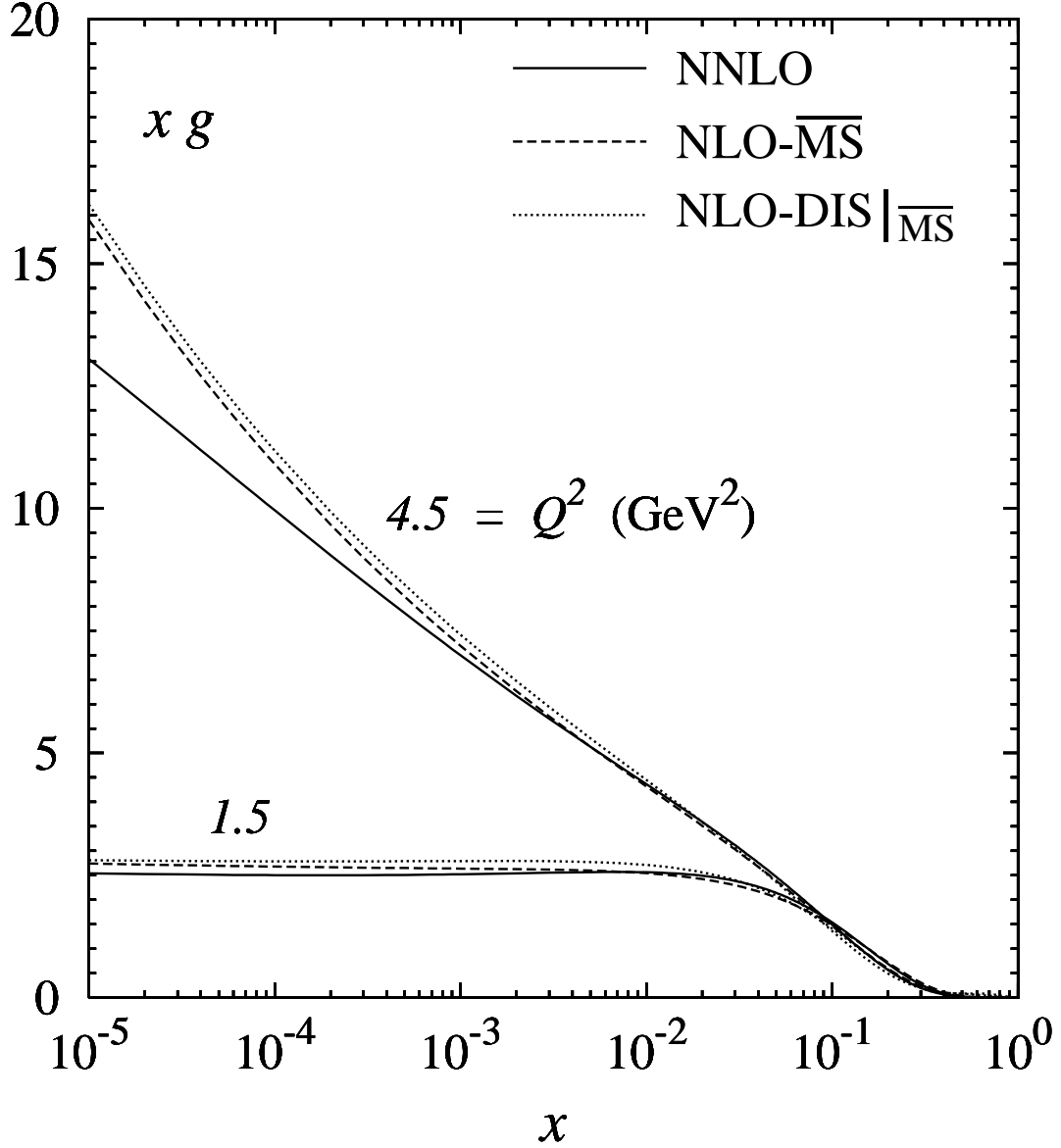
Figure 2: The gluon distributions at the input scale Q_0^2 = 1.5 \text{ GeV}^2 , corresponding to (13) with the parameters given in Table 1, and at Q^2 = 4.5 \text{ GeV}^2 . For a consistent comparison with the NNLO and NLO results in the \overline{\text{MS}} factorization scheme, we have transformed our NLO-DIS results to the \overline{\text{MS}} scheme using (9) which are denoted by \text{NLO-DIS}|_{\overline{\text{MS}}} .
