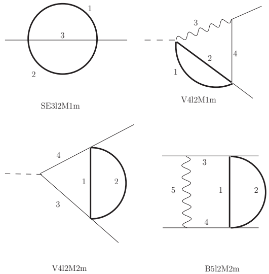
Figure 1. The topologies of the eight master integrals for the heavy-fermion corrections. Bold lines represent heavy fermions.
