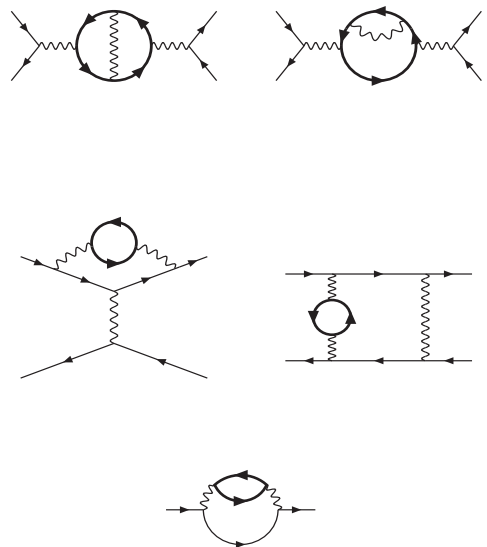
Figure 2. The diagrams for Bhabha scattering with two fermion flavors. Internal fermionic loops represent heavy leptons and the other fermion lines are electrons.
