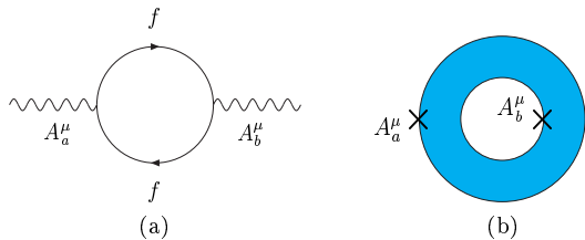
FIG. 1: (a) One-loop diagram which contributes to kinetic-mixing in field theory, and (b) its equivalent in open string theory (from Ref. [14]).
