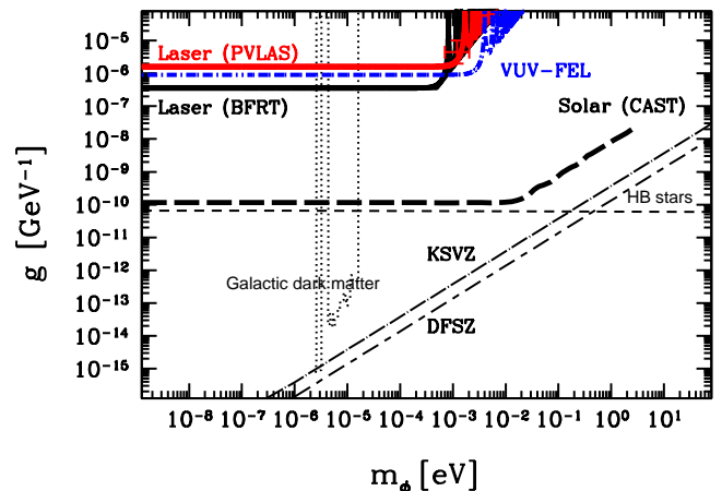
FIG. 3: Exclusion region in mass m_\phi vs. coupling g for various current and future experiments. The laser experiments [6, 7] aim at (pseudo-)scalar production and detection in the laboratory. The galactic dark matter experiments [12] exploit microwave cavities to detect pseudoscalars under the assumption that these pseudoscalars are the dominant constituents of our galactic halo, and the solar experiments search for axions from the sun [10]. The constraint from horizontal branch (HB) stars [9] arises from a consideration of stellar energy losses through (pseudo-)scalar production. The predictions from two quite distinct QCD axion models, namely the KSVZ [13] (or hadronic) and the DFSZ [14] (or grand unified) one, are also shown.
