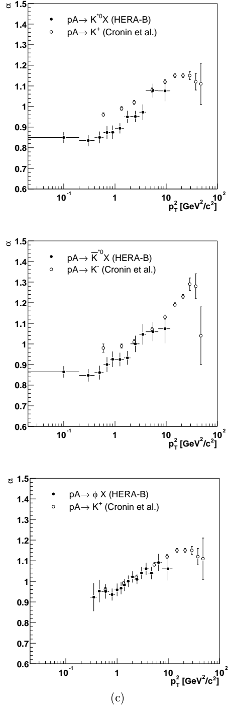
Figure 9. Measured values of \alpha(p_T) for a) K^{*0} , b) \bar{K}^{*0} and c) \phi production. The results of Cronin et al. [21] on the K^\pm mesons are superimposed. Numbers of this analysis are summarised in Table 7.
