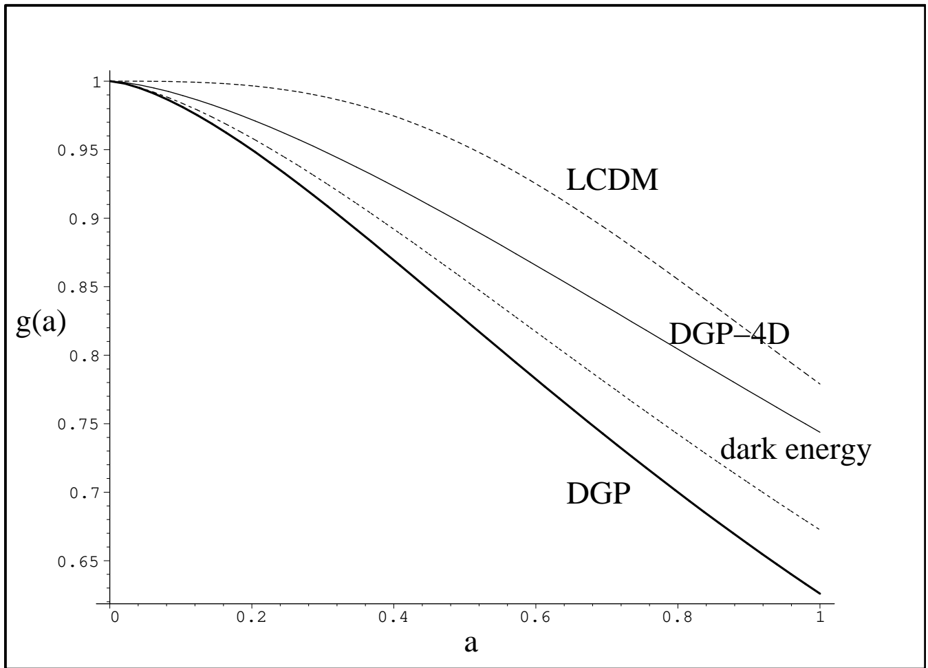
FIG. 4 The linear growth history g(a) \equiv \delta/a for flat \Lambda CDM (long dashed), DGP Dark Gravity (thick solid) and Dark Energy models in Fig. 3. Because the DGP model Newton's "constant" weakens with time, it shows a little more growth suppression than that in the mimicking Dark Energy model. DGP-4D (thin solid) shows the incorrect result obtained by neglecting perturbations of the DGP 5D Weyl tensor. The 5D Weyl tensor perturbations make dynamical Dark Gravity (DGP) and Dark Energy hard to resolve, but both dynamical models are distinguishable from static Dark Energy. (from (Koyama and Maartens, 2005))
