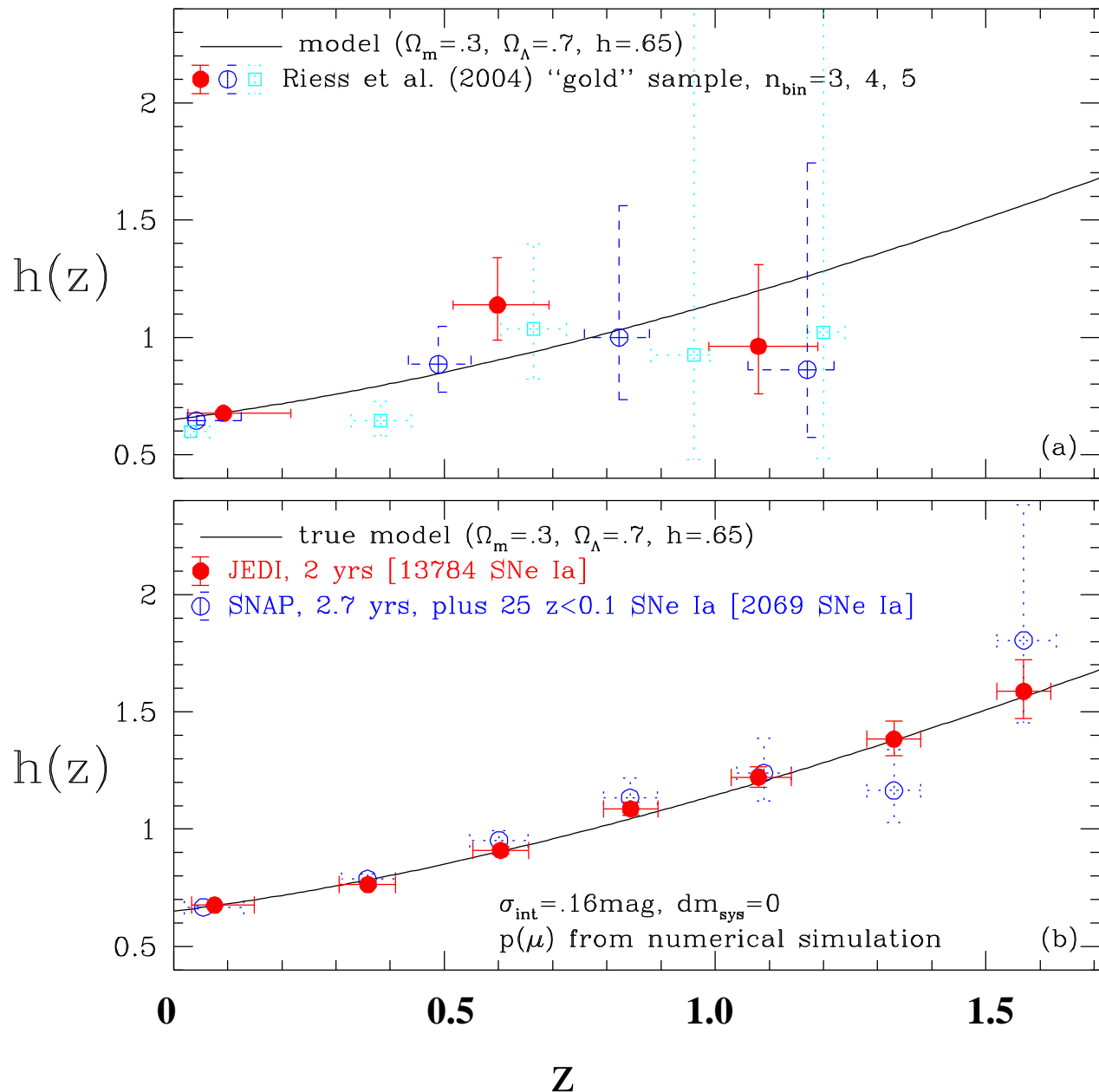
FIG. 1 The cosmic expansion history (dimensionless Hubble parameter h(z)=H(z)/100 ) from the Riess et al. (2004) Gold sample (top panel) and from simulated future data (bottom panel) for the NASA/JDEM mission concepts JEDI (solid points) and SNAP (dotted points) (Wang and Tegmark, 2005). The existing Gold sample data and the simulated future JEDI are both consistent with \Lambda CDM (solid curve) (from (Wang and Tegmark, 2005)).
