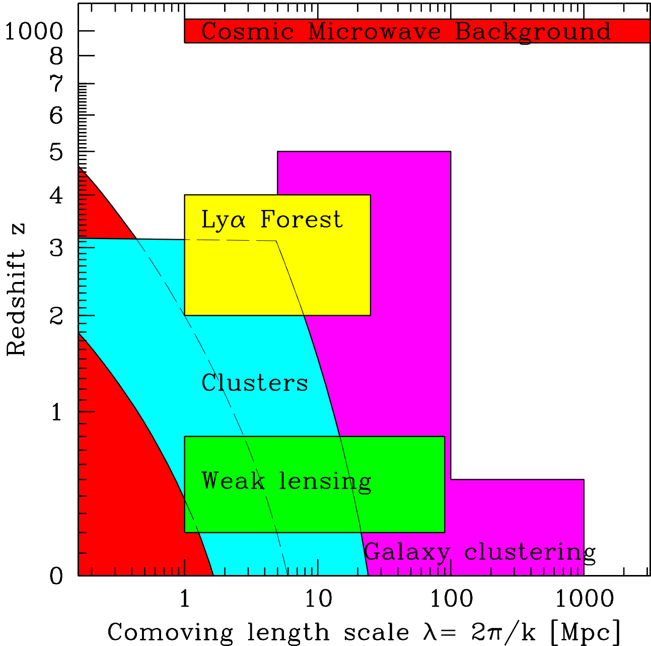
FIG. 2 Shaded regions show ranges of scale and redshift over which various cosmological observations are likely to measure spacetime fluctuations over the next few years. The lower left region, delimited by the dashed line, is the non-linear regime where rms density fluctuations exceed unity in the \Lambda CDM model (from (Tegmark, 2002)).
