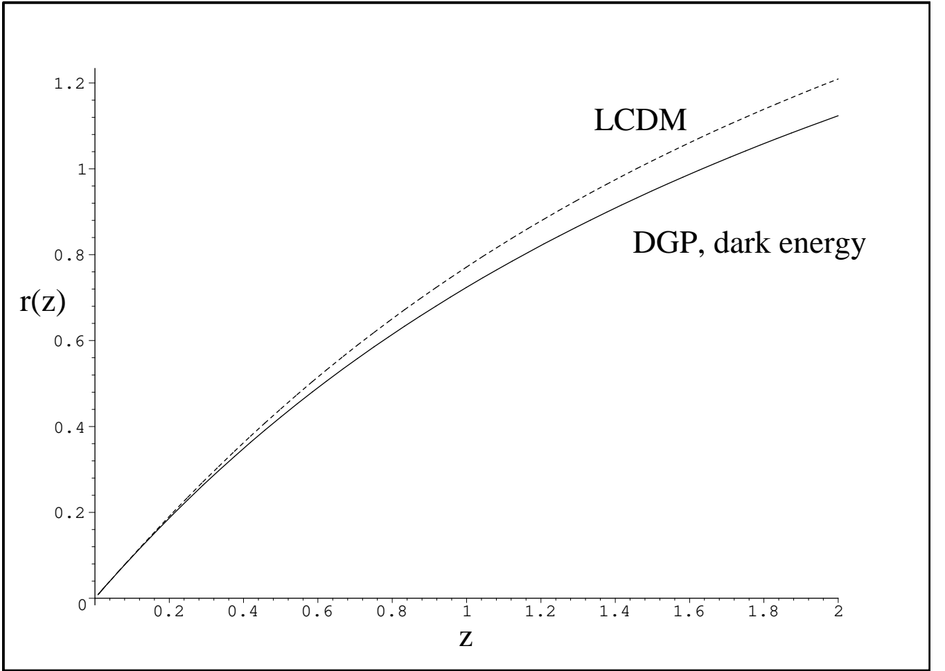
FIG. 3 The proper motion or conformal distance r(z) = c \int_0^z dz'/H(z') back to redshift z , calculated for flat \Lambda CDM (dashed) and DGP Dark Gravity (solid) models with present matter fraction \Omega_{m0} = 0.3 . The DGP Dark Gravity model is also mimicked by a Dark Energy model with w(a) = -0.78 + 0.32z/(1+z) . Between static and dynamic “dark energy”, the differences in distances and in expansion history H(z) = cz/r(z) are small, but the differences in growth factor will be larger in FIG. 4. (from (Koyama and Maartens, 2005)).
