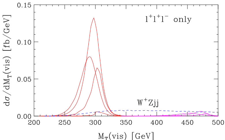
FIG. 5: Transverse mass distribution of the visible \ell^+\ell^+\ell^-jj\cancel{p}_T system in gg \rightarrow \eta \rightarrow ZH, H \rightarrow WW resonant production at the LHC. Red and magenta curves are for the Golden Point and F_{1,2} = 1.0, 2.0 TeV, respectively, and the dashed blue curve is the W^+Zjj background.
