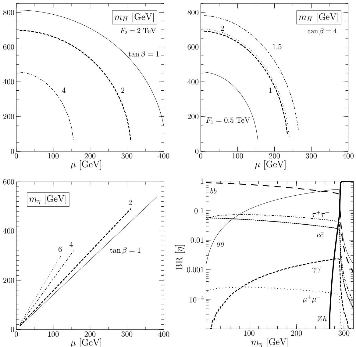
FIG. 1: Typical values for the pseudo-axion and Higgs masses in the Simplest Little Higgs model as a function of the explicit symmetry breaking parameter \mu . Upper pair: left, Higgs mass for fixed F_2 = 2 TeV; right, for fixed \tan\beta = 4 . Lower pair: left, \eta mass; right, \eta branching fractions.
