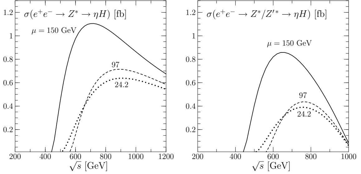
FIG. 6: Total cross section for H\eta production at an ILC for different values of \mu , m_\eta , m_h : the Golden Point with 150/309.2/131.7 GeV (solid), 97/200.0/368.4 GeV (dashed), and 24.2/50.0/451.3 GeV (dotted). The left panel is without the presence of a Z' resonance, while the right panel includes destructive Z - Z' interference for m_{Z'} = 1152 GeV.
