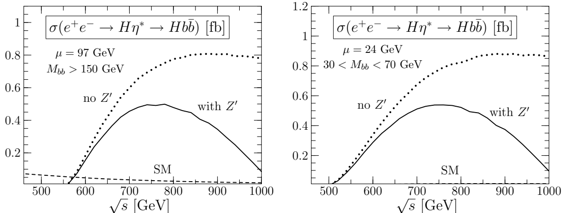
FIG. 8: Cross section for Hb\bar{b} production in the \mu -model pseudo-axion with (solid line) and without (dotted line) the Z' resonance at the Golden Point. The dashed line is the SM prediction. On the left is \mu = 97 GeV, right \mu = 24.2 GeV.
