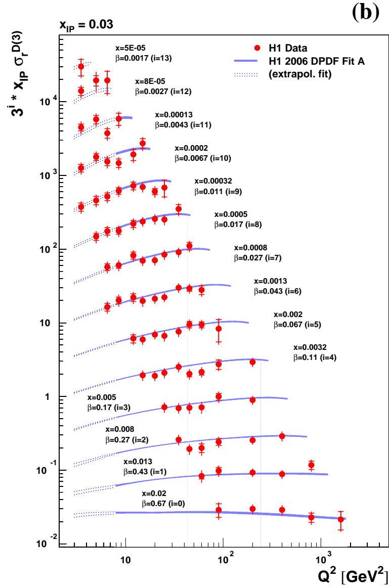
Figure 6: The \beta and Q^2 dependences of the diffractive reduced cross section, multiplied by x_{IP} , at x_{IP} = 0.03 . See the captions of figures 2 and 5 for further details.
