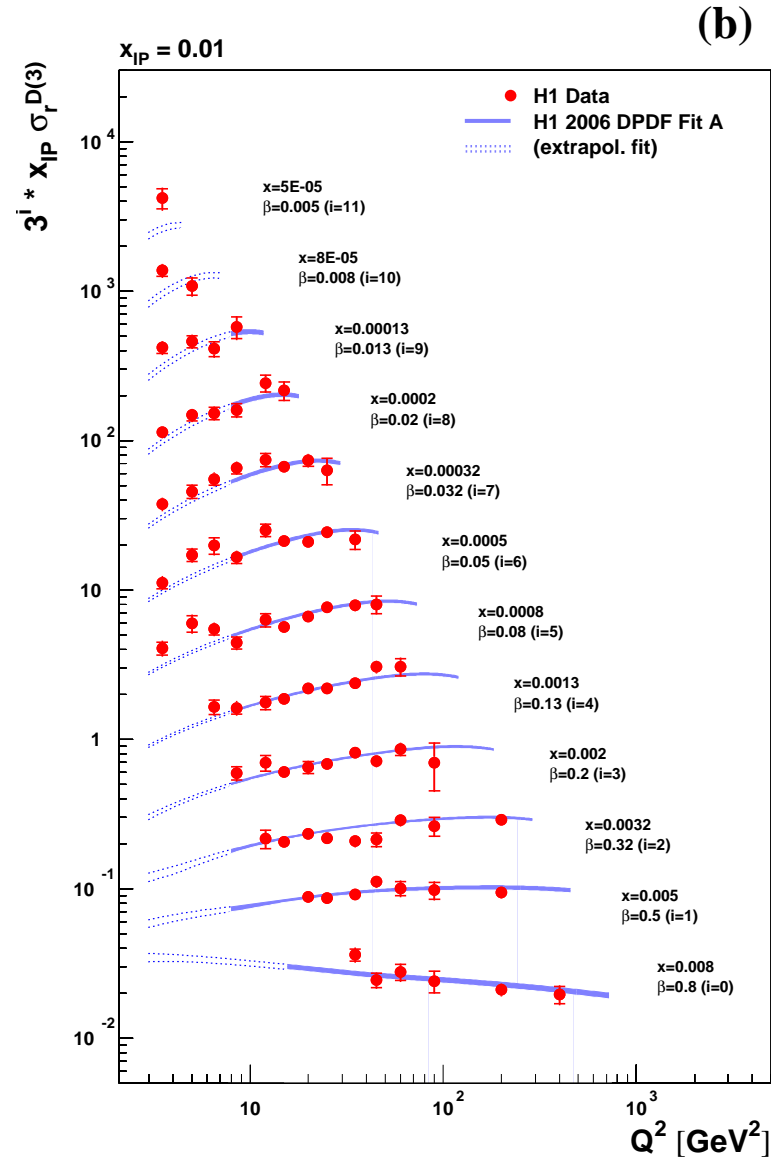
Figure 5: The \beta and Q^2 dependences of the diffractive reduced cross section, multiplied by x_{IP} , at x_{IP} = 0.01 . In (a), the contribution of the sub-leading exchange alone according to the ‘H1 2006 DPDF Fit A’ is also shown. The data with Q^2 \leq 90 \text{ GeV}^2 ( Q^2 \geq 200 \text{ GeV}^2 ) were obtained with E_p = 820 \text{ GeV} ( E_p = 920 \text{ GeV} ). The fit results are shown for E_p = 820 \text{ GeV} . See the caption of figure 2 for further details.
