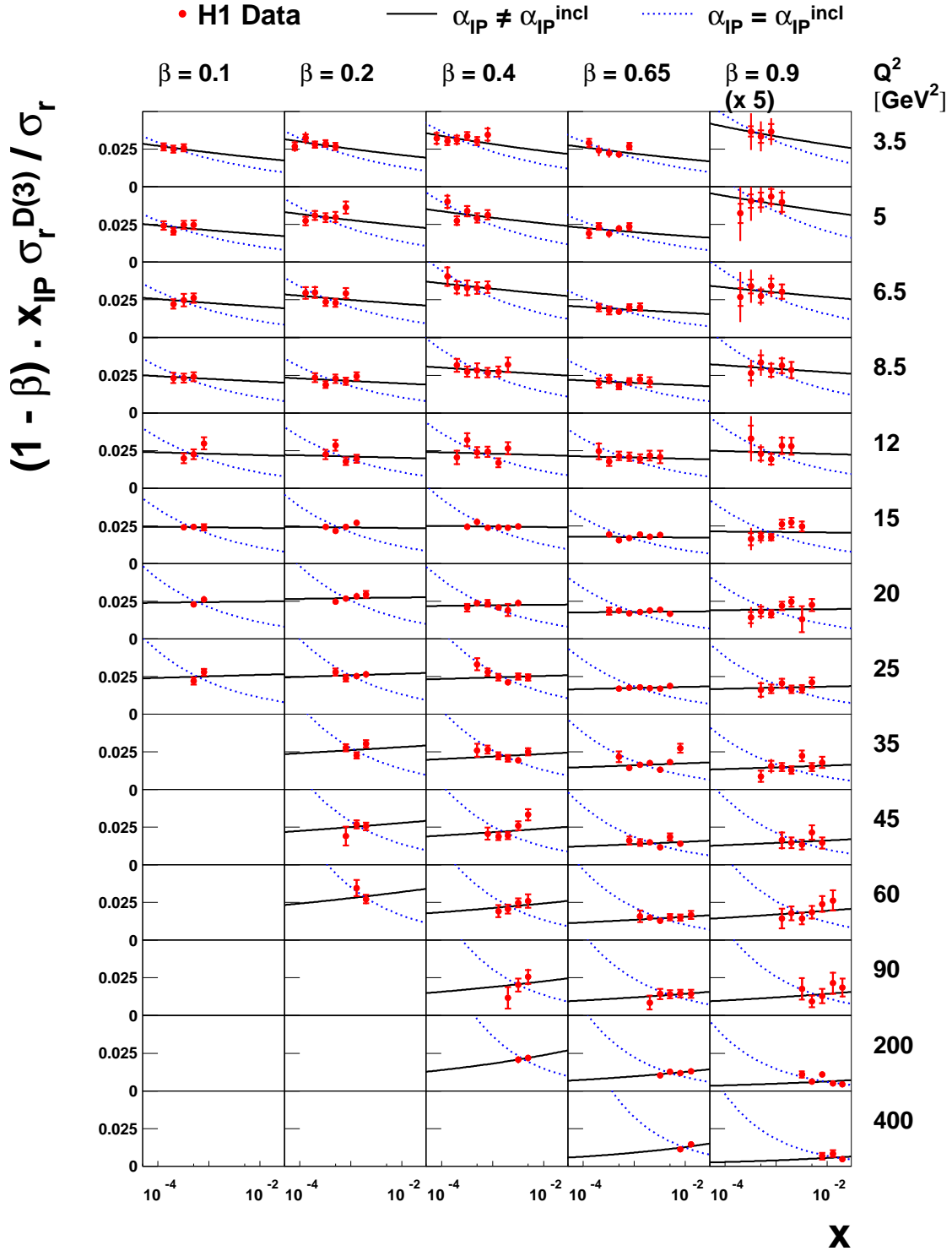
Figure 19: The ratio of the diffractive to the inclusive reduced cross section, multiplied by (1 - \beta)x_{\text{P}} . Data at \beta = 0.9 are multiplied by a further factor of 5 for visibility. Data which are significantly influenced by the sub-leading exchange or the longitudinal structure function according to the NLO QCD fit are excluded. The remaining data are compared with models motivated by Regge phenomenology as described in the text, for which the diffractive and inclusive effective pomeron trajectories are the same ( \alpha_{\text{P}} = \alpha_{\text{P}}^{\text{incl}} ) and for which they are different ( \alpha_{\text{P}} \neq \alpha_{\text{P}}^{\text{incl}} ).
