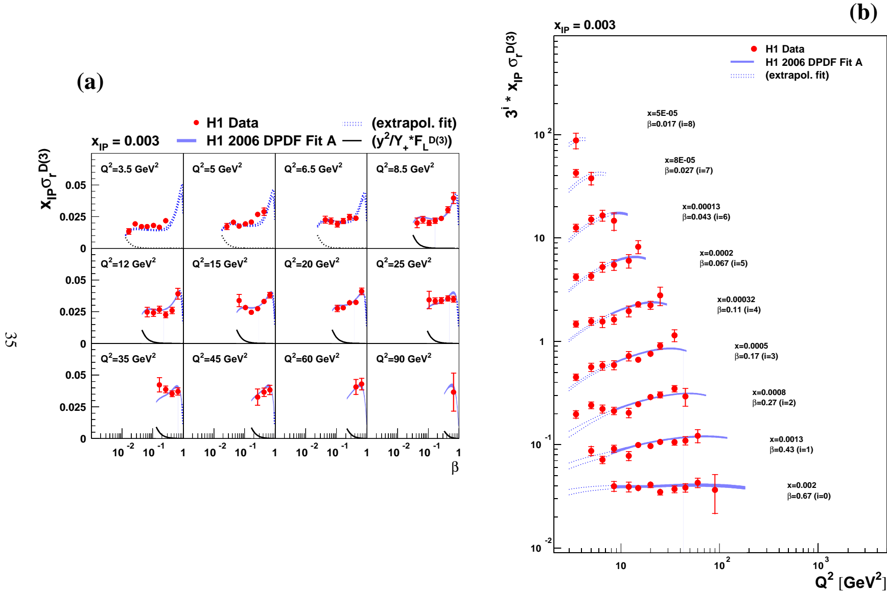
Figure 4: The \beta and Q^2 dependences of the diffractive reduced cross section, multiplied by x_P , at x_P = 0.003 . In (a), the quantity y^2/Y_+ \cdot F_L^{D(3)} is also shown, as extracted from the ‘H1 2006 DPDF Fit A’. Adding this quantity to the reduced cross section yields F_2^{D(3)} . See the caption of figure 2 for further details.
