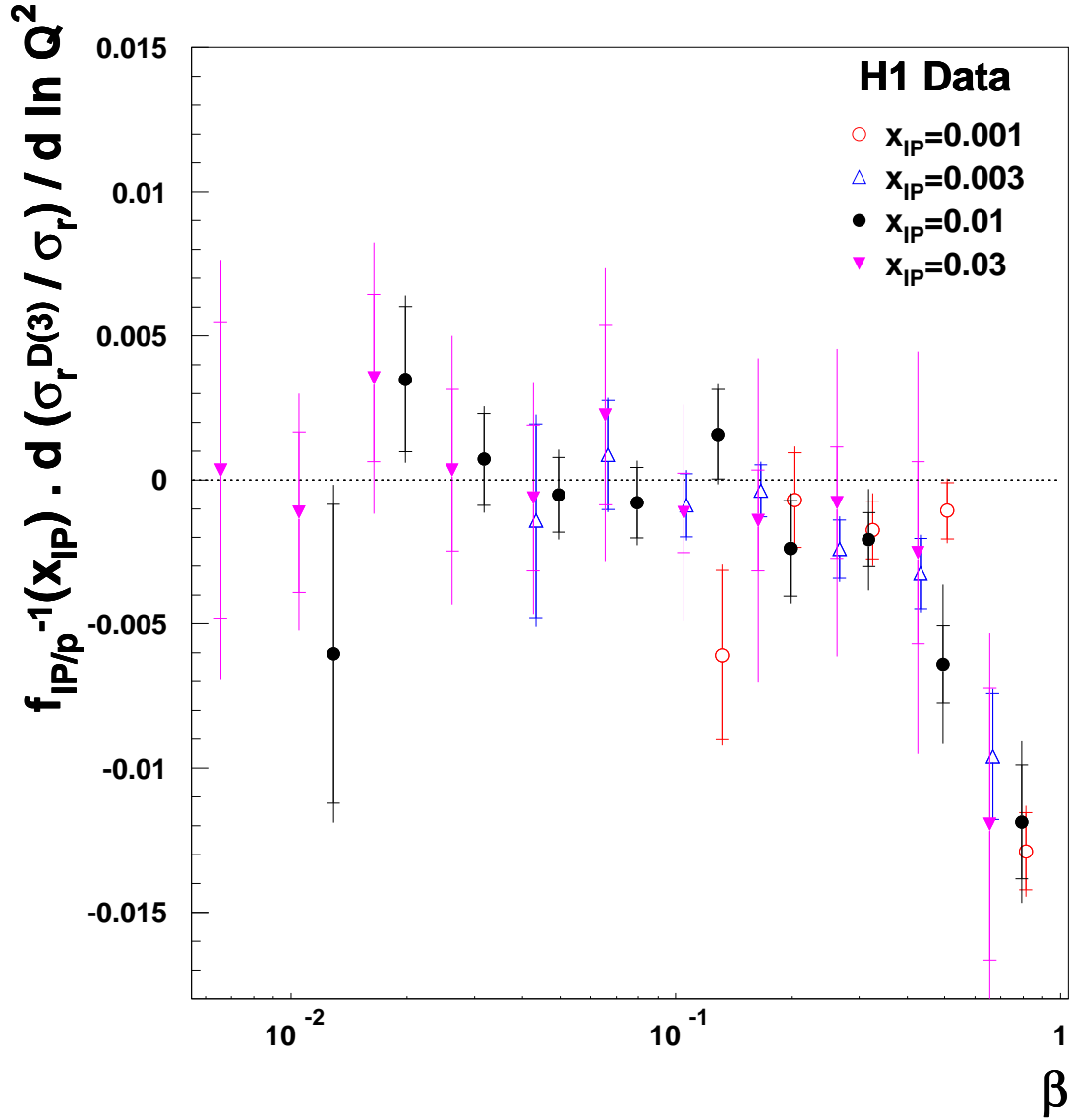
Figure 18: The logarithmic Q^2 derivative of the ratio of the reduced diffractive cross section to the reduced inclusive cross section at different fixed values of x_{IP} and \beta (see equation 19). The derivatives are divided by the diffractive flux factor as defined in equation 14. The inner and outer error bars represent the statistical and total uncertainties, respectively. Normalisation uncertainties are not shown.
