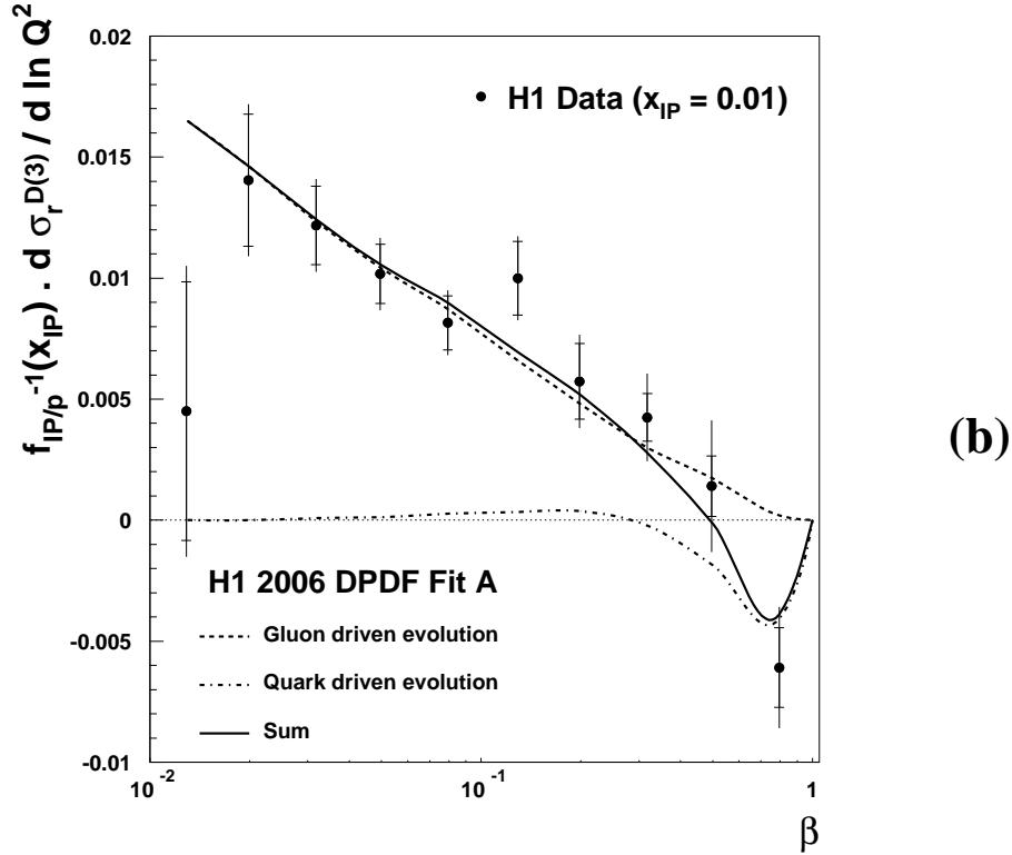
Figure 7: (a) Measurements of the logarithmic Q^2 derivative of the reduced diffractive cross section at different fixed values of x_{IP} and \beta , obtained by fitting equation 10 to the data. The derivatives are divided by the diffractive flux factor as defined in equation 14. (b) The logarithmic Q^2 derivative at x_{IP} = 0.01 , divided by the diffractive flux factor and compared with the prediction of the ‘H1 2006 DPDF Fit A’. The prediction is also decomposed into contributions to the evolution from the splittings g \rightarrow q\bar{q} (‘Gluon driven evolution’) and q \rightarrow qg (‘Quark driven evolution’). The inner and outer error bars represent the statistical and total uncertainties, respectively. Normalisation uncertainties are not shown.
