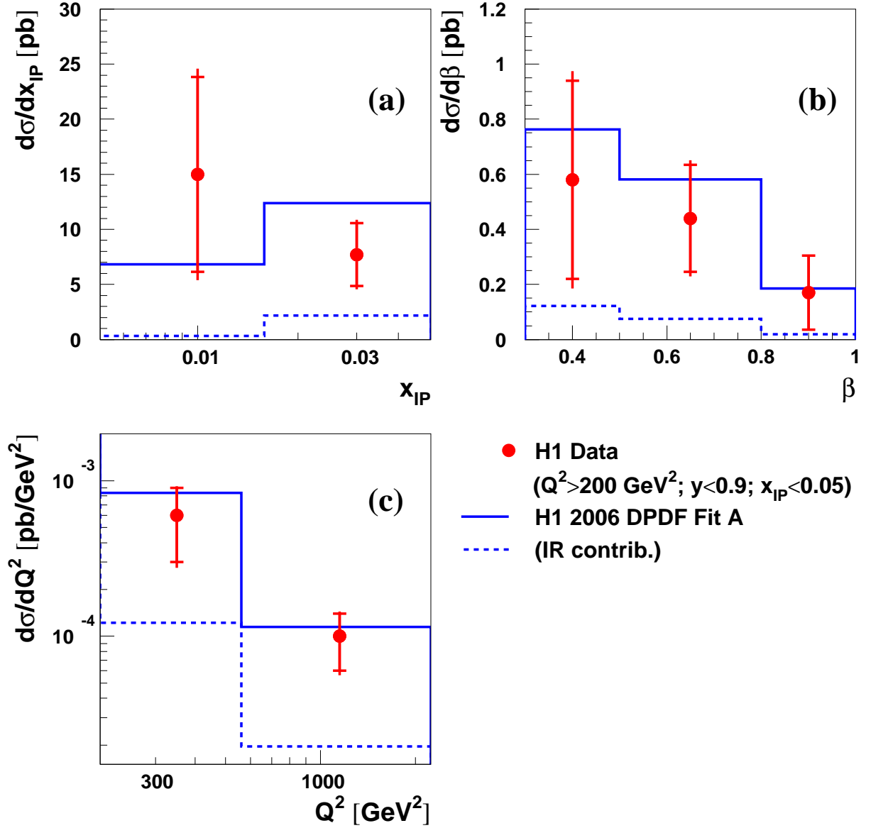
Figure 15: The cross section for the diffractive process e^+p \rightarrow \bar{\nu}_e XY at E_p = 920 GeV, shown differentially in (a) x_{IP} , (b) \beta and (c) Q^2 , for Q^2 > 200 GeV 2 , y < 0.9 and x_{IP} < 0.05 . The data are compared with the predictions of the ‘H1 2006 DPDF Fit A’ to the neutral current data, obtained using the RAPGAP Monte Carlo generator. The contribution to the predictions from the sub-leading exchange is also shown. The data points correspond to average values of the differential cross sections over the regions shown by the histograms. The inner and outer error bars on the data points represent the statistical and total uncertainties, respectively. Normalisation uncertainties are not shown.
