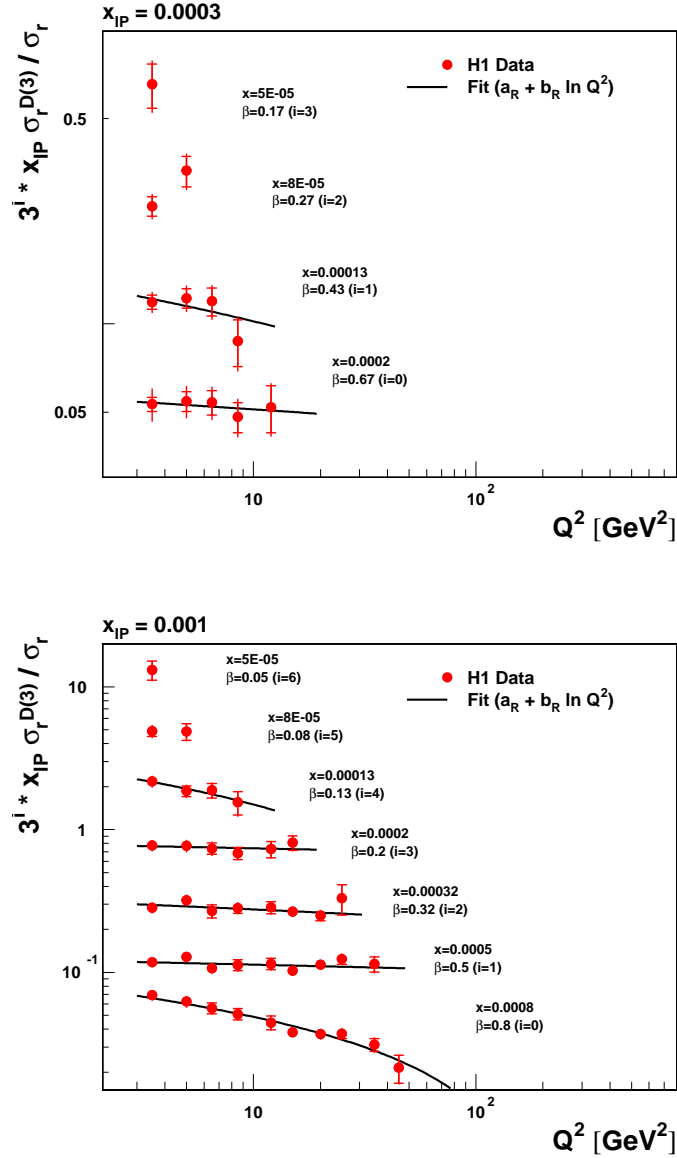
Figure 16: The ratio of the diffractive to the inclusive reduced cross section, multiplied by x_{IP} and shown as a function of Q^2 for fixed x and fixed x_{IP} = 0.0003, 0.001 and 0.003 . The data are multiplied by a further factor of 3^i for visibility, with i as indicated. The inner and outer error bars represent the statistical and total uncertainties, respectively. Normalisation uncertainties are not shown. The results of fits to a linear dependence on \log Q^2 (equation 19) to the data are also shown.
